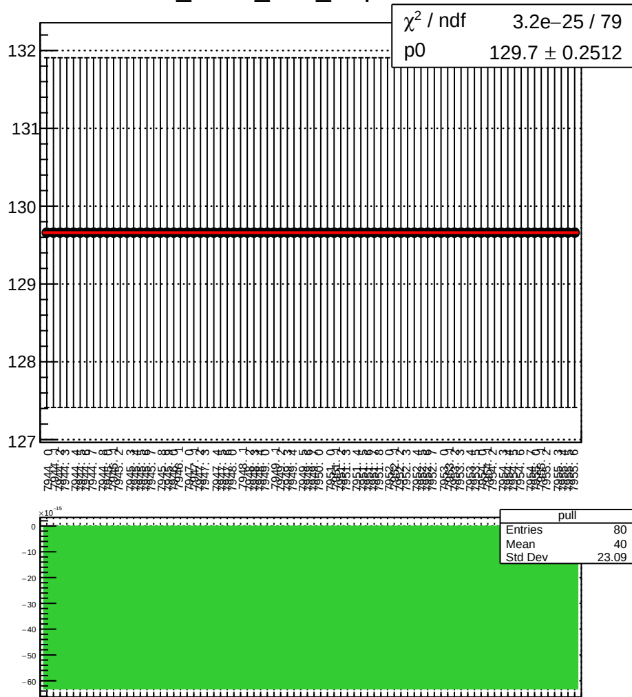
dit_sam5_4eY_slope vs run
