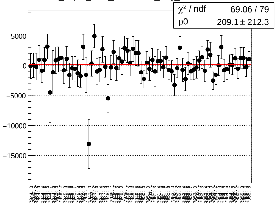
dit_asym_sam_12345678_avg_mean vs run
