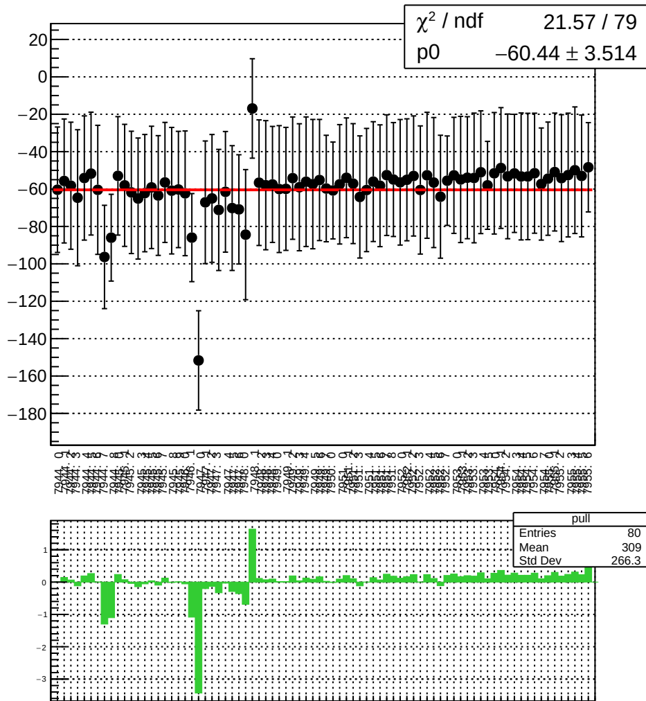
reg_asym_sam_48_dd_diff_bpm1X_slope vs run
