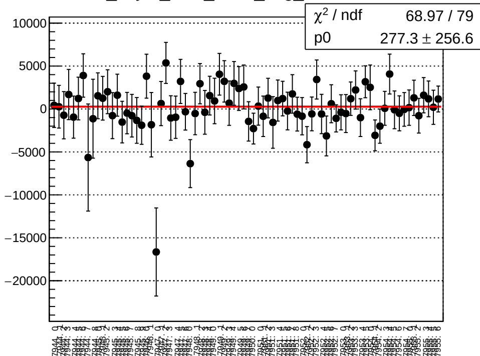
dit_asym_sam_2468_avg_g_mean vs run
