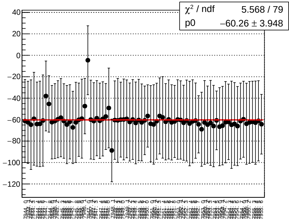
reg_asym_sam_24_68_dd_diff_bpm4eX_slope vs run
