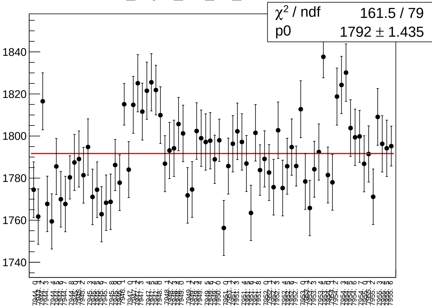
dit_asym_at2_dd_rms vs run
