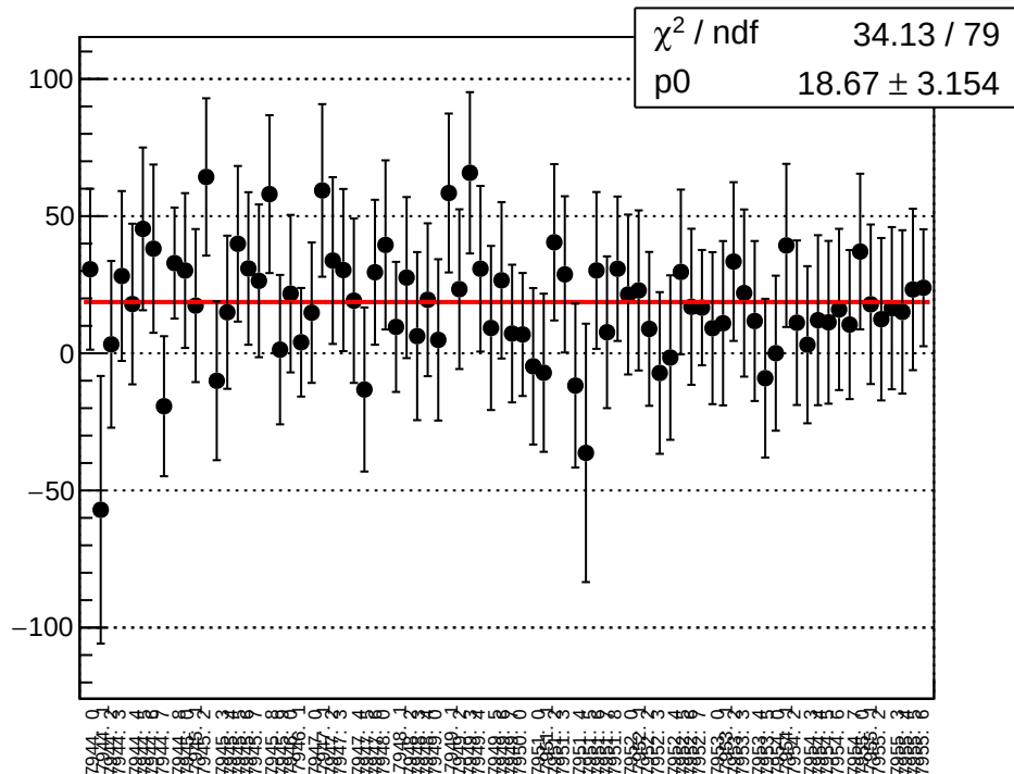
reg_asym_atl_dd_atr_dd_diff_bpm1X_slope vs run
