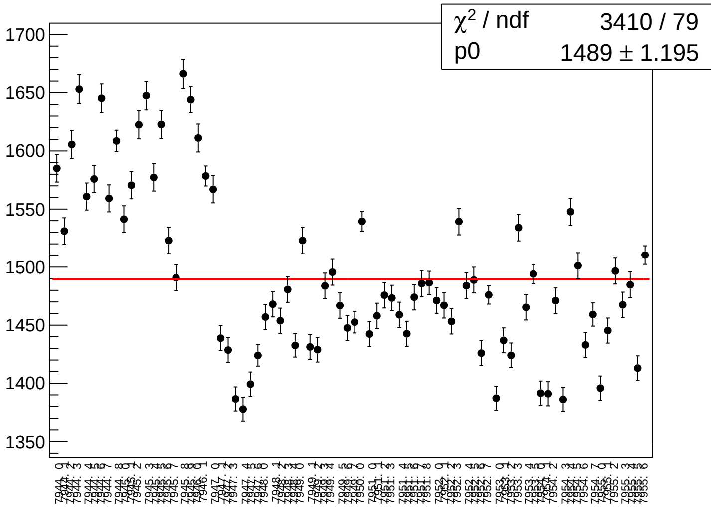
asym atl avg atr avg dd correction rms vs run
