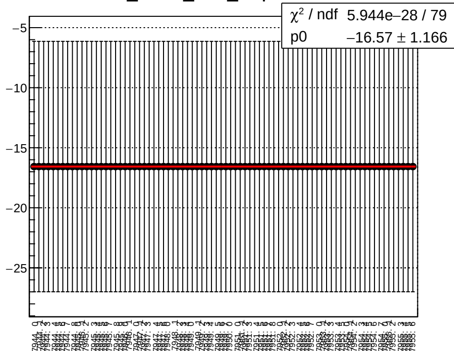
dit_sam4_4aY_slope vs run
