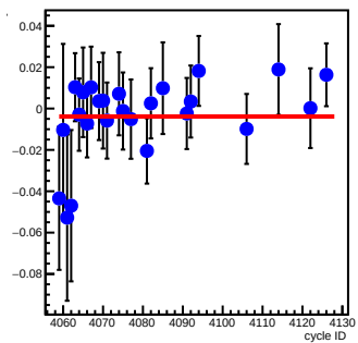
bpm12X_coil6(um/count)
