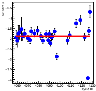
sam8_coil2(ppm/count)
