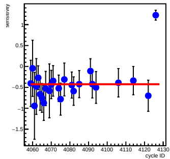
sam8_coil6(ppm/count)
