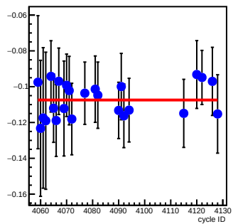
bpm4aX_coil5(um/count)
