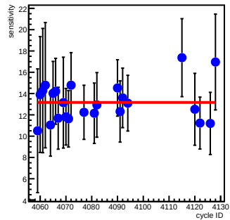
sam4_coil5(ppm/count)
