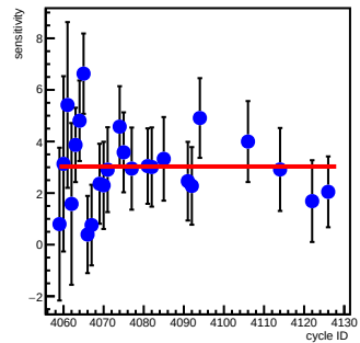
at11_coil6(ppm/count)
