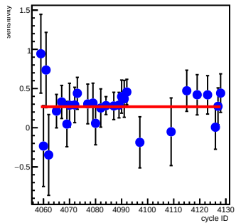
sam6_coil2(ppm/count)
