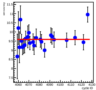
sam1_coil6(ppm/count)
