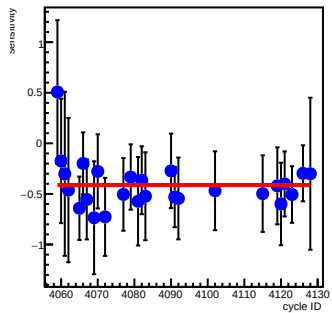
sam7_coil5(ppm/count)
