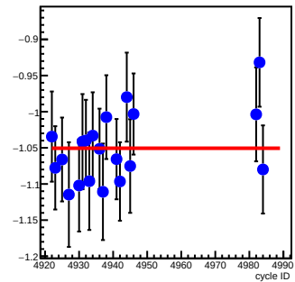
sam7_coil2(ppm/count)
