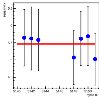
at12_coil6(ppm/count)
