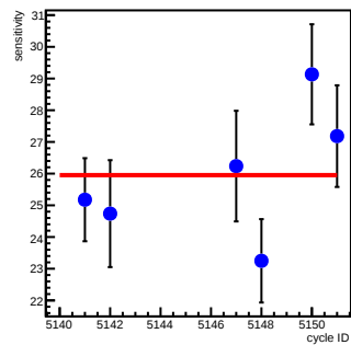
at12_coil5(ppm/count)
