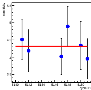
at12_coil2(ppm/count)
