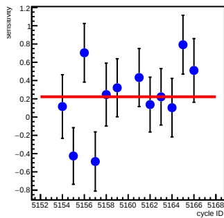
at11_coil6(ppm/count)
