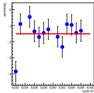
at11_coil5(ppm/count)
