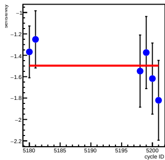
sam6_coil2(ppm/count)
