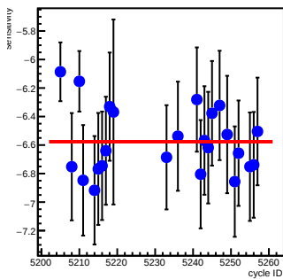
usl_coil5(ppm/count)
