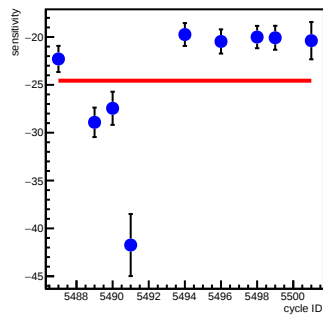
sam4_coil5(ppm/count)
