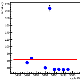
sam4_coil2(ppm/count)
