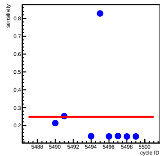
bpm4aY_coil2(um/count)
