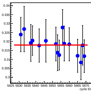
bpm1X_coil7(um/count)
