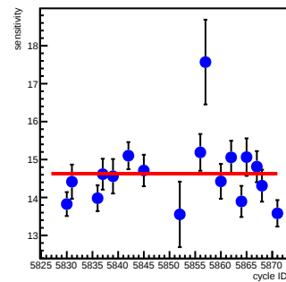
sam6_coil2(ppm/count)
