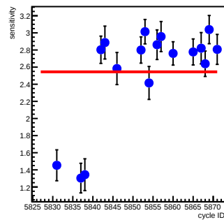
sam6_coil6(ppm/count)
