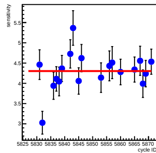
sam6_coil5(ppm/count)
