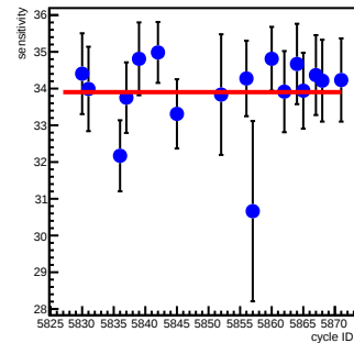
sam4_coil2(ppm/count)
