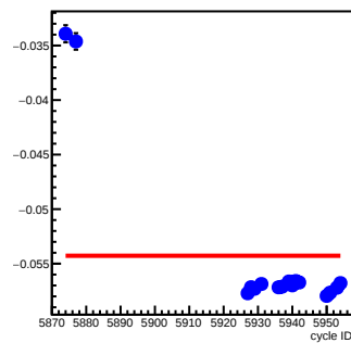
bpm4eY_coil6(um/count)
