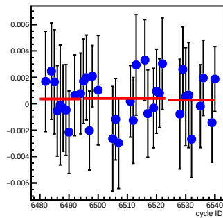
bpm11X_coil5(um/count)
