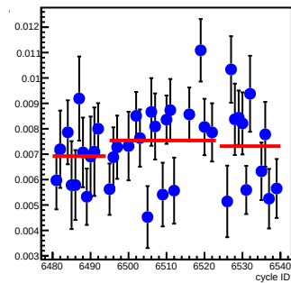
bpm11X_coil6(um/count)
