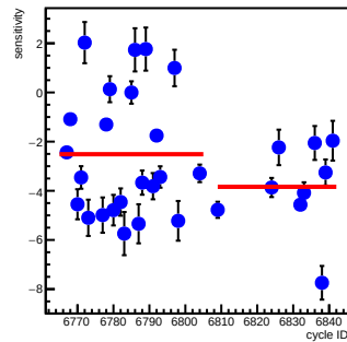
sam4_coil6(ppm/count)
