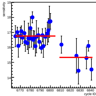
sam6_coil2(ppm/count)
