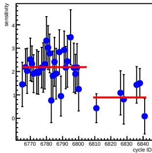
at1_coil2(ppm/count)
