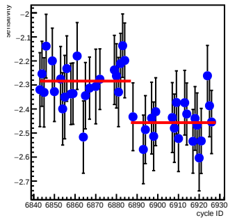
sam1_coil5(ppm/count)
