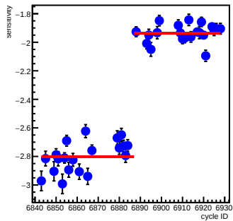
sam1_coil6(ppm/count)
