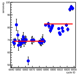
sam4_coil7(ppm/count)
