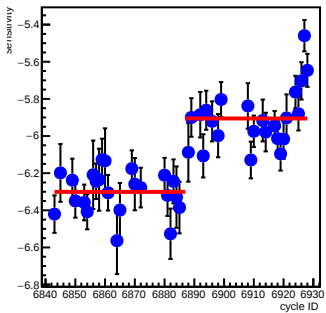
sam1_coil2(ppm/count)
