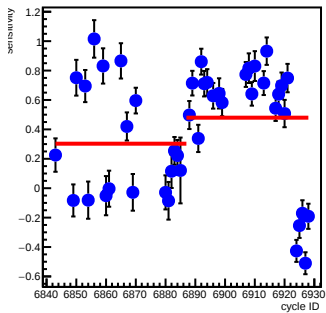
sam5_coil2(ppm/count)
