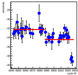
sam2_coil5(ppm/count)
