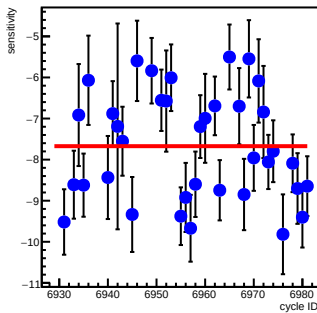
at12_coil6(ppm/count)
