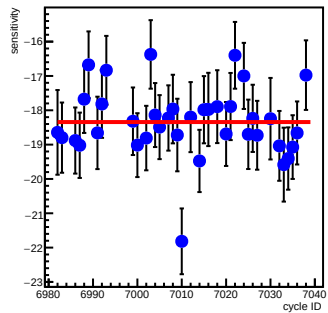
at11_coil7(ppm/count)
