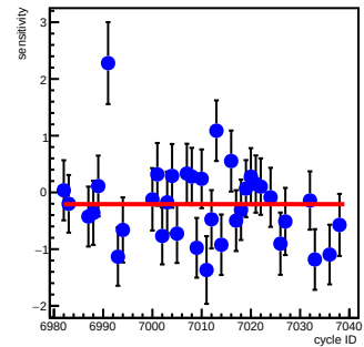
at11_coil2(ppm/count)
