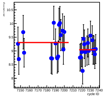
sam6_coil5(ppm/count)
