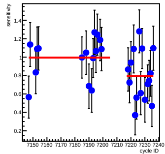
atr1_coil6(ppm/count)
