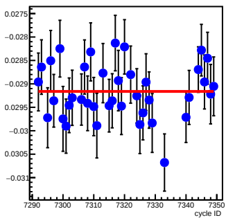
bpm4eY_coil6(um/count)
