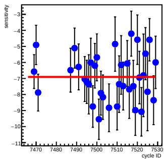
atr2_coil2(ppm/count)
