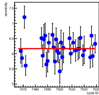
sam2_coil6(ppm/count)
