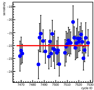
sam2_coil2(ppm/count)
