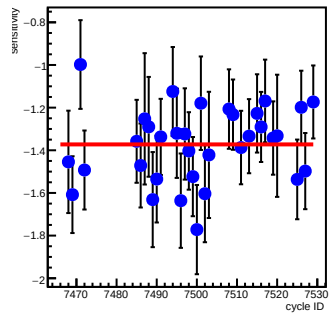
sam3_coil6(ppm/count)
