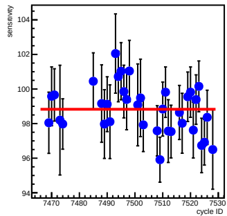
sam4_coil7(ppm/count)
