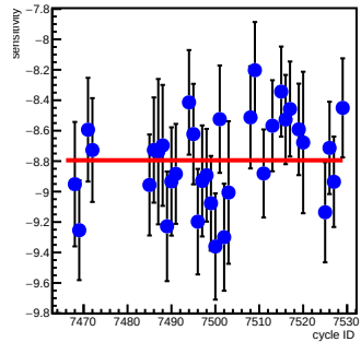
sam4_coil6(ppm/count)
