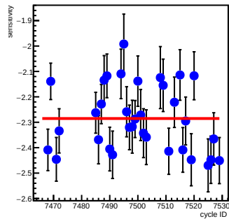
sam5_coil6(ppm/count)
