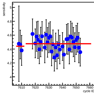
sam7_coil2(ppm/count)
