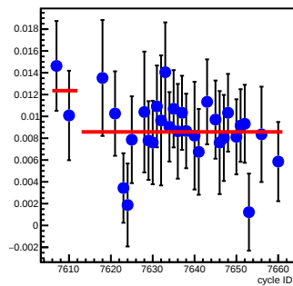
bpm4aX_coil2(um/count)
