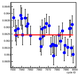
bpm4aY_coil6(um/count)
