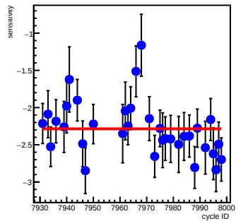
sam4_coil6(ppm/count)
