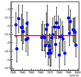
sam2_coil2(ppm/count)
