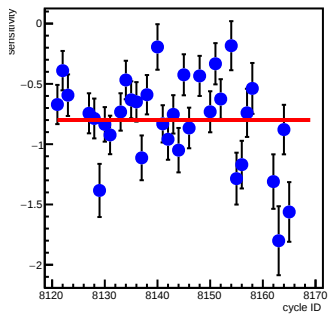
usl_coil6(ppm/count)
