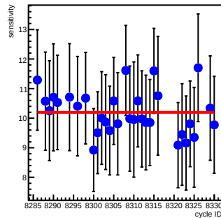
atr2_coil5(ppm/count)
