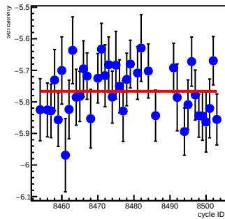
sam1_coil2(ppm/count)
