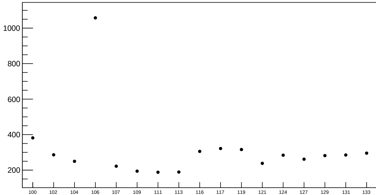
reg_asym_sam4 RMS (ppm)
