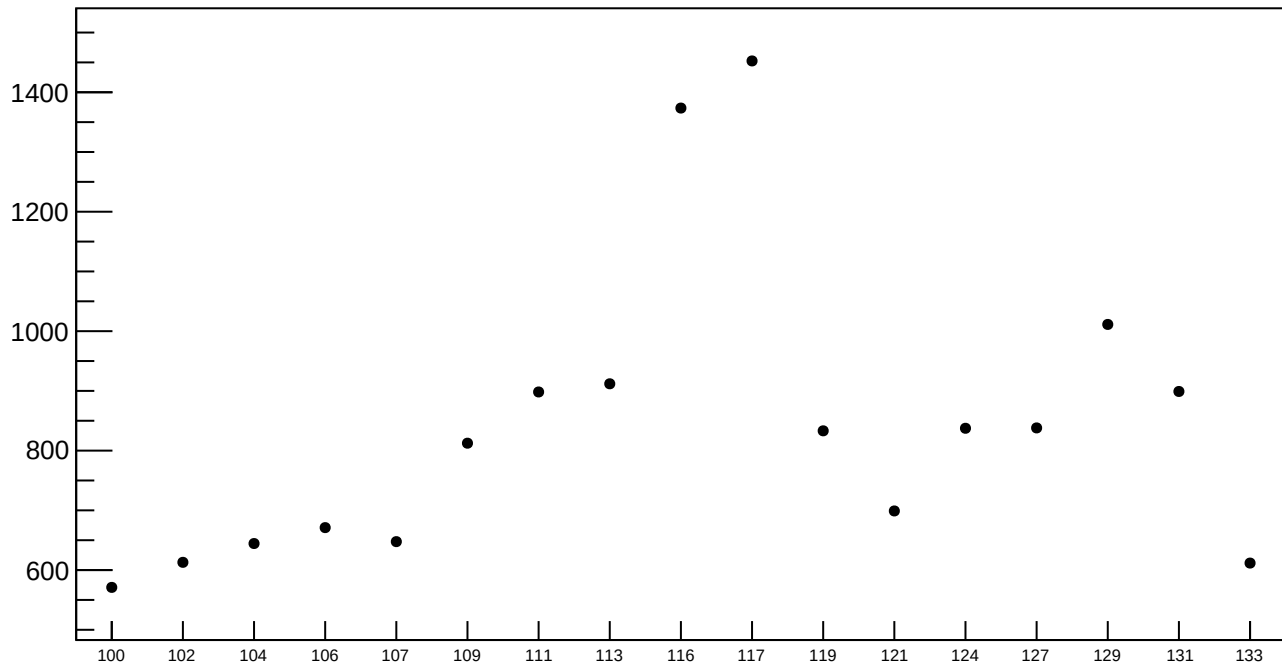
asym_sam_15_dd RMS (ppm)
