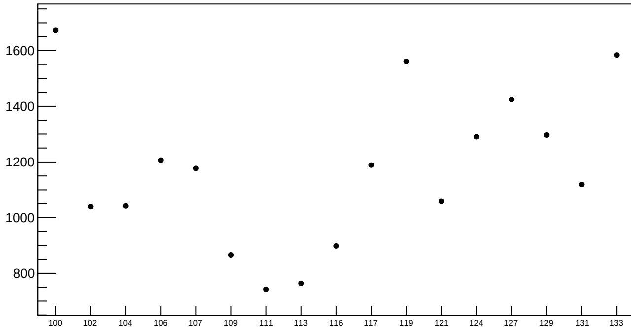
asym_sam_37_avg RMS (ppm)
