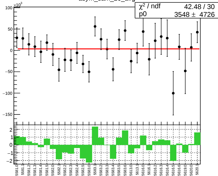
asym_sam_26_avg
