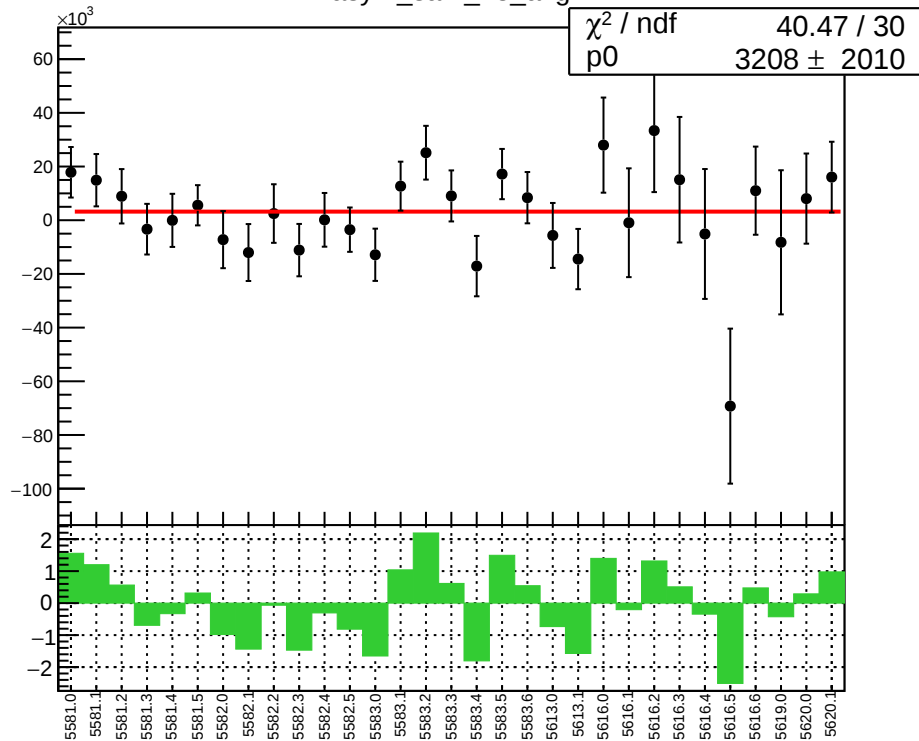
asym_sam_48_avg
