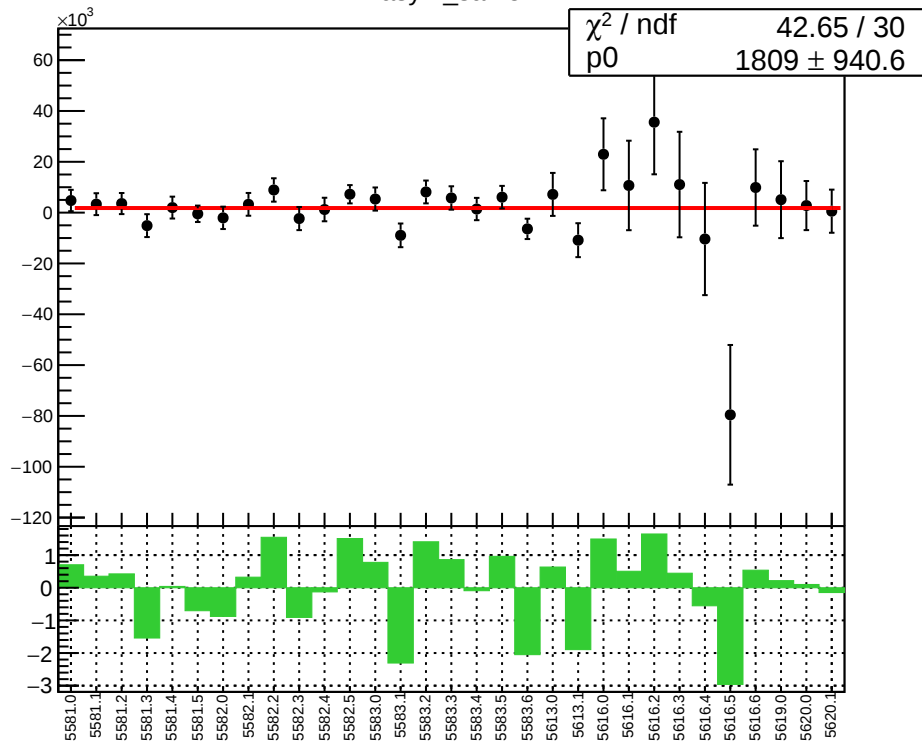
asym_sam5
