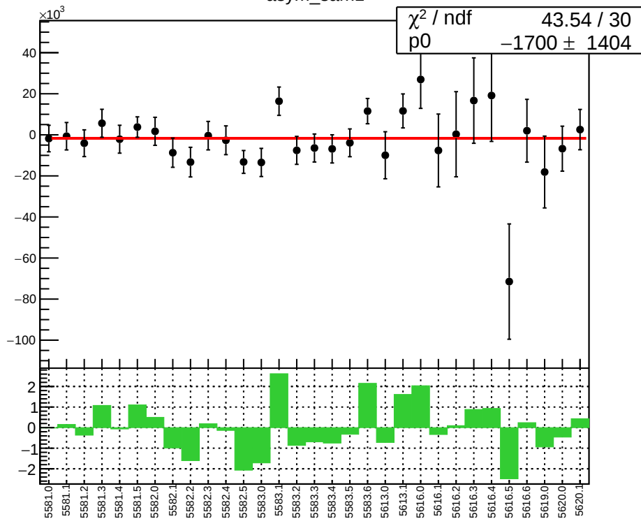
asym_sam1
