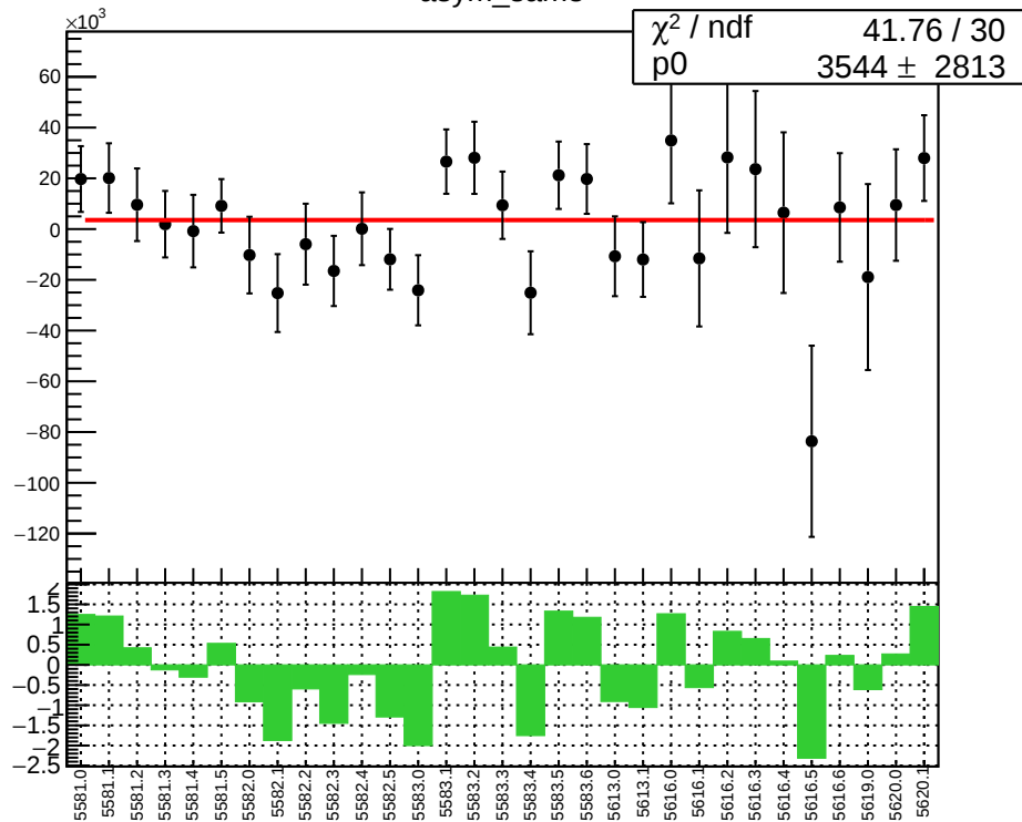
asym_sam3
