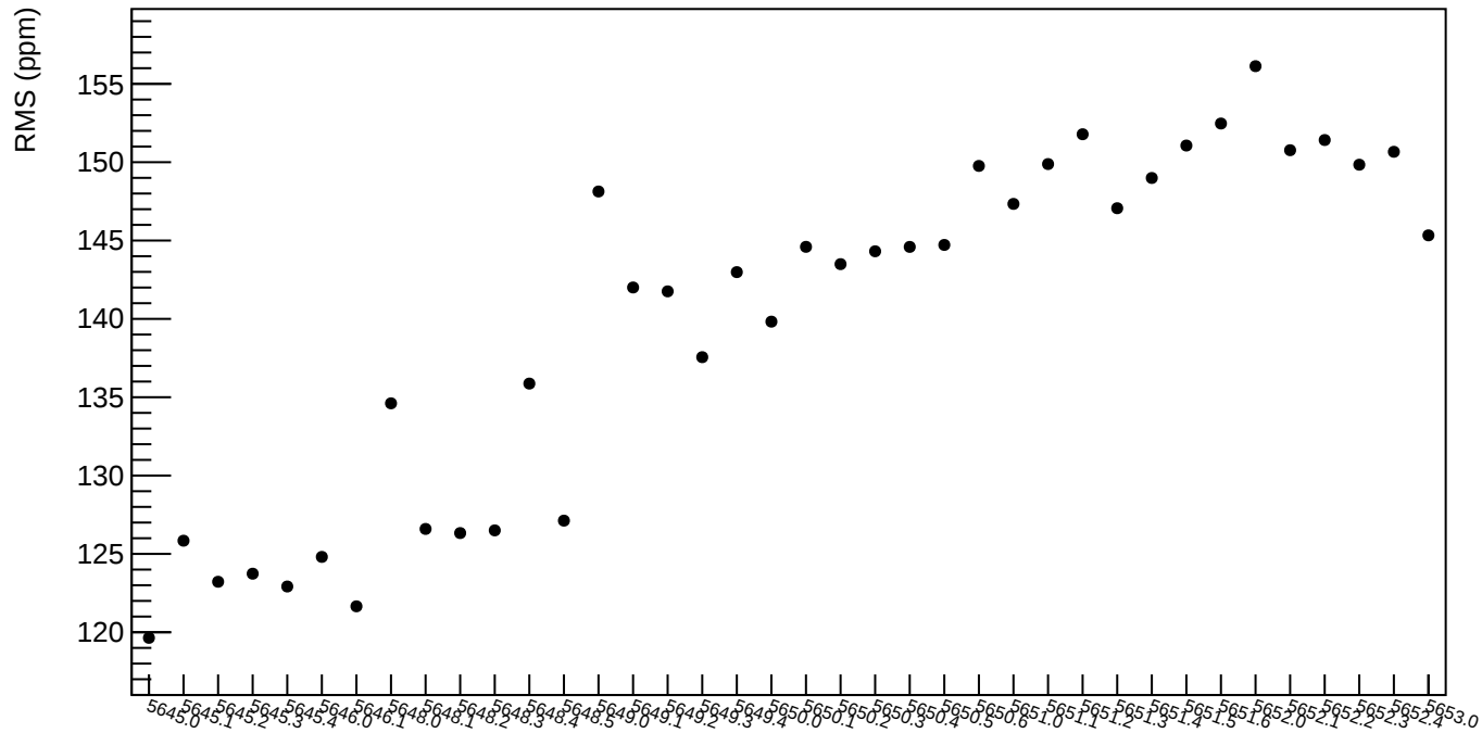
reg_asym_sam1 RMS (ppm)
