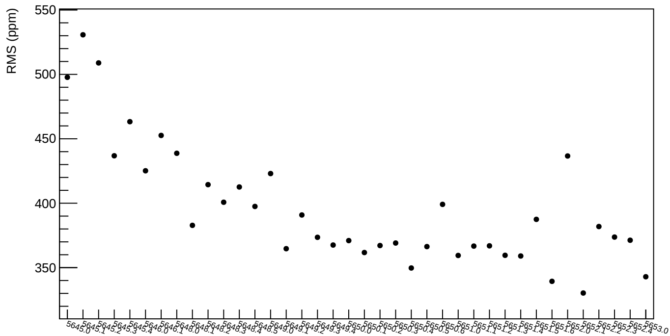
asym_sam6 RMS (ppm)
