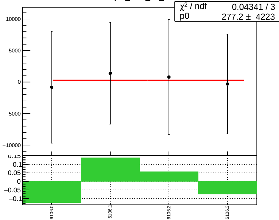
asym_sam_37_dd
