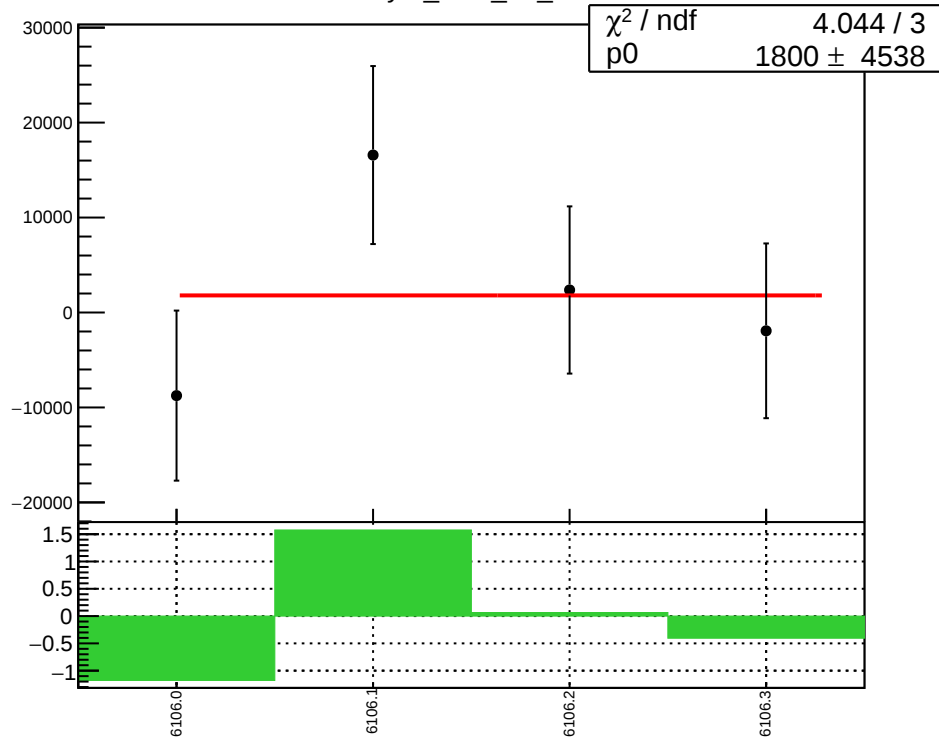
asym_sam_15_dd
