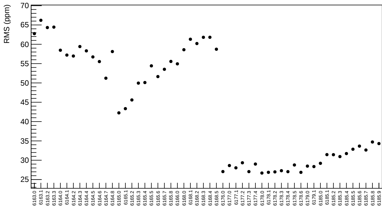
diff_bpm12X RMS (ppm)
