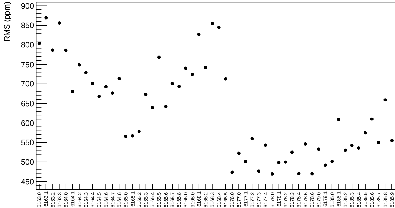
asym_sam7 RMS (ppm)
