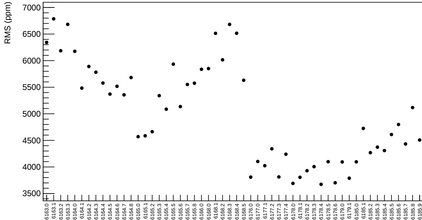
asym_sam2 RMS (ppm)
