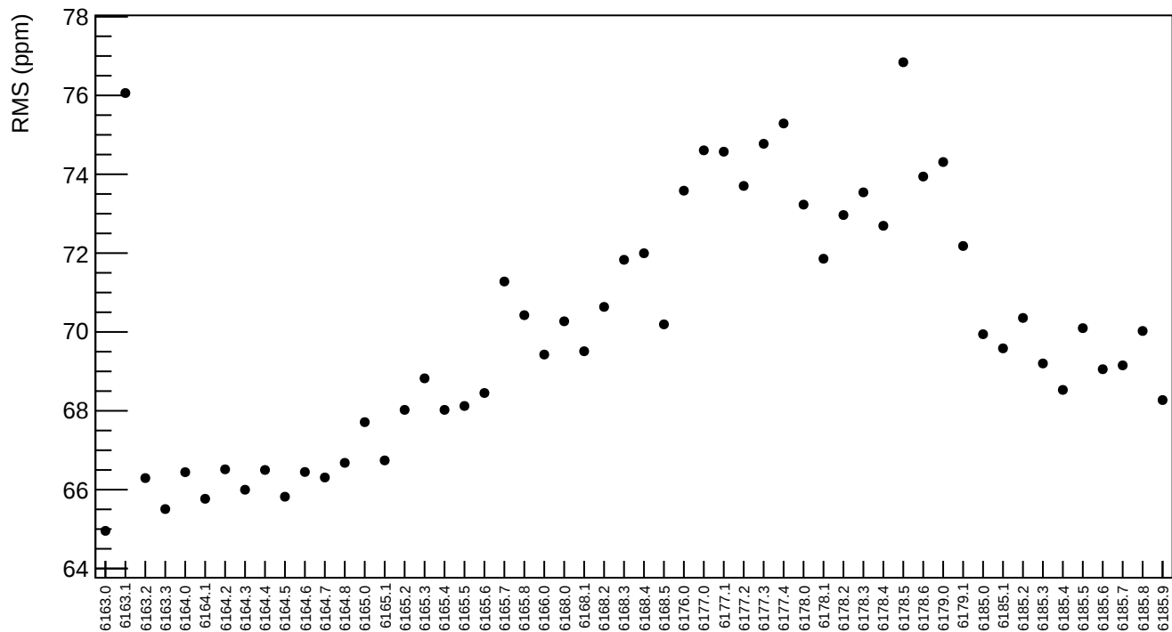
reg_asym_sam1 RMS (ppm)
