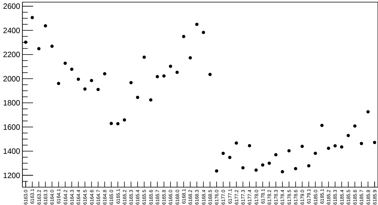
asym_sam_26_avg RMS (ppm)
