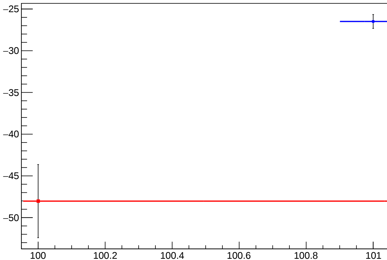
reg_asym_sam_1357_avg_diff_bpm4aX_slope vs Slug
