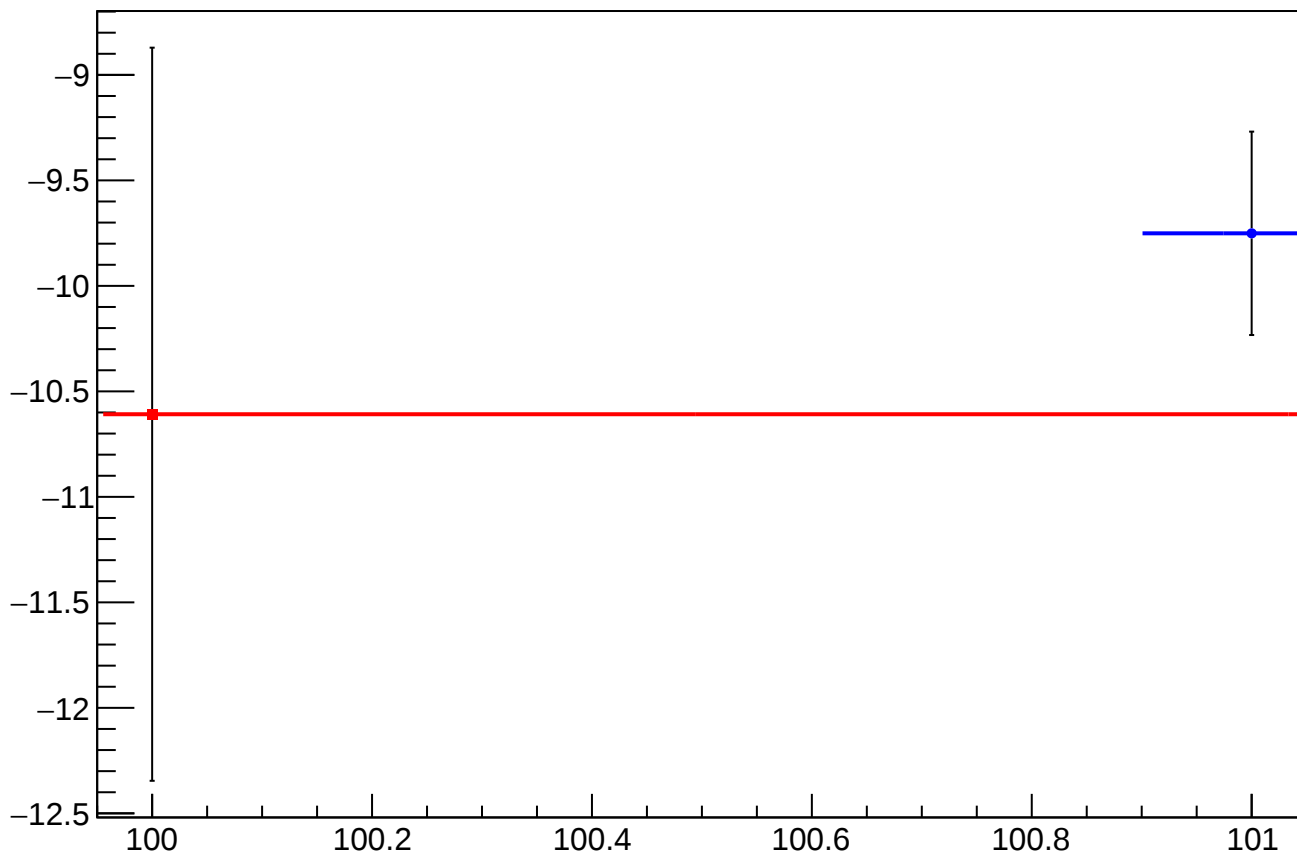
reg_asym_sam8_diff_bpm4aX_slope vs Slug
