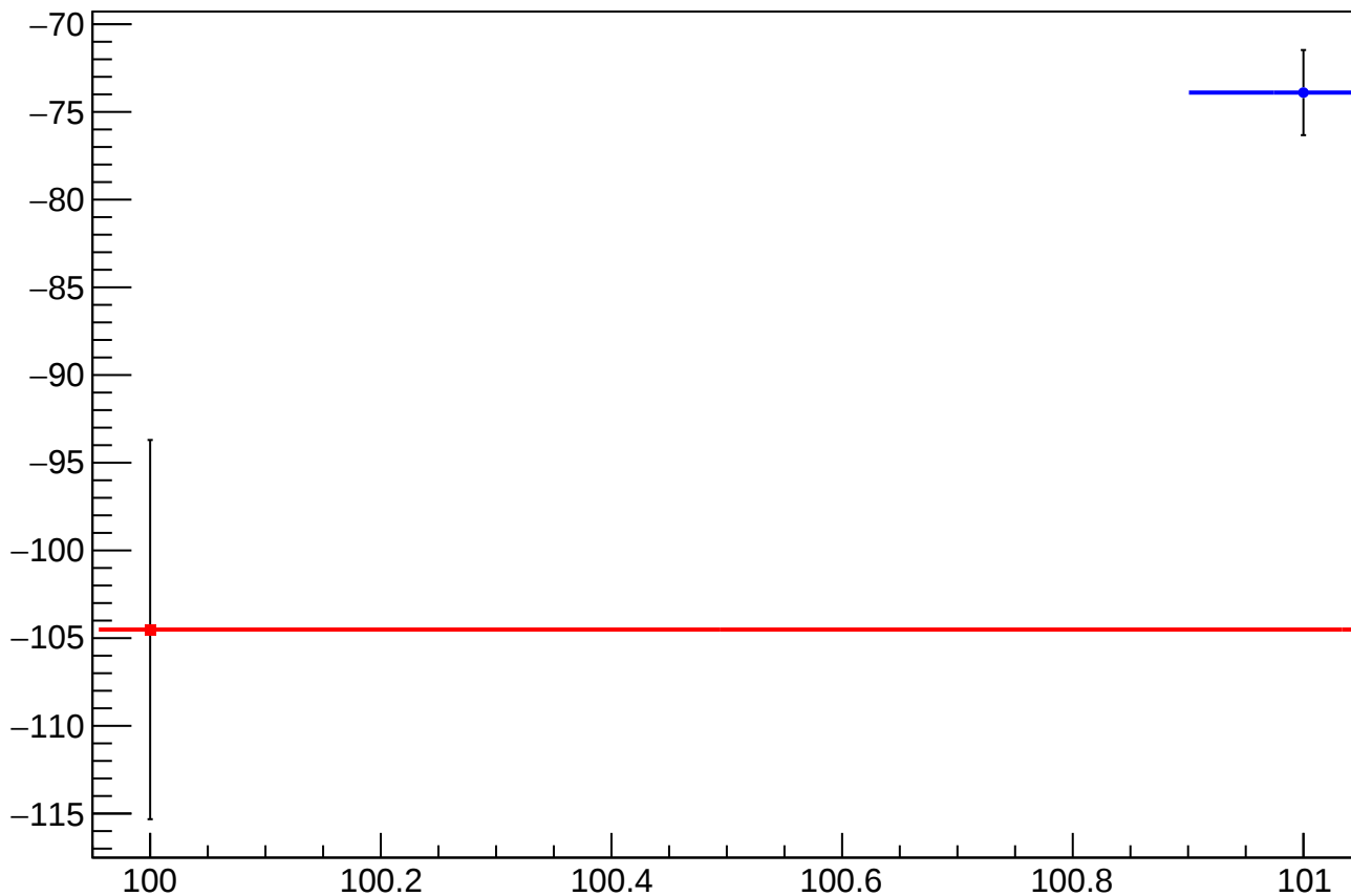
reg_asym_sam_2468_avg_diff_bpm4aX_slope vs Slug
