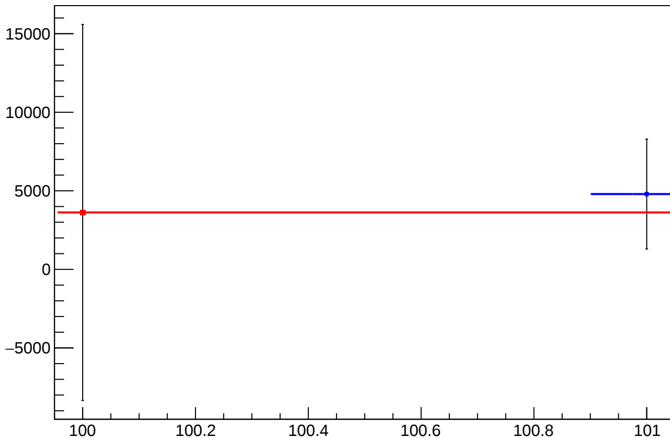
reg_asym_atl2_mean vs Slug
