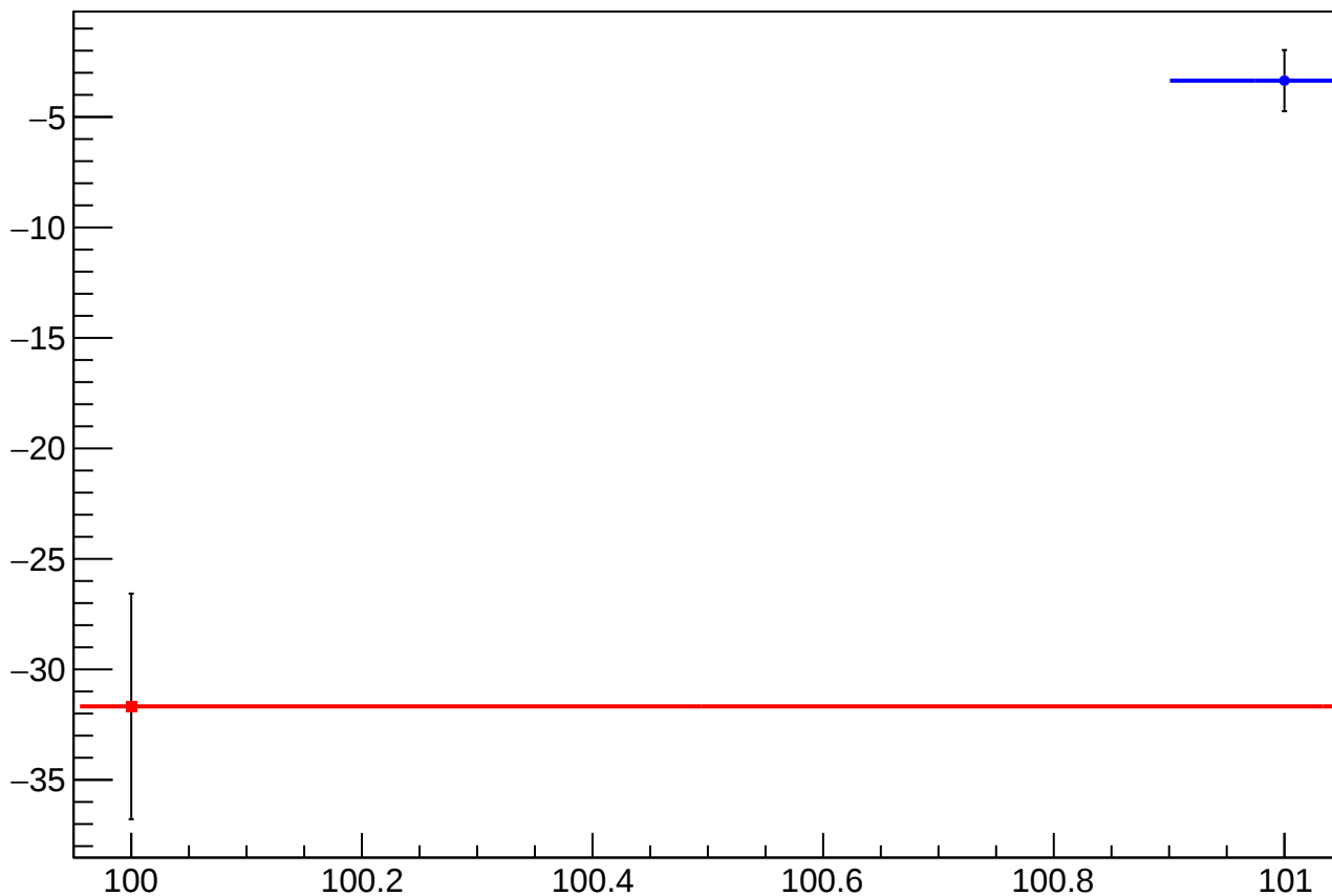
reg_asym_sam_26_48_dd_diff_bpm4aX_slope vs Slug
