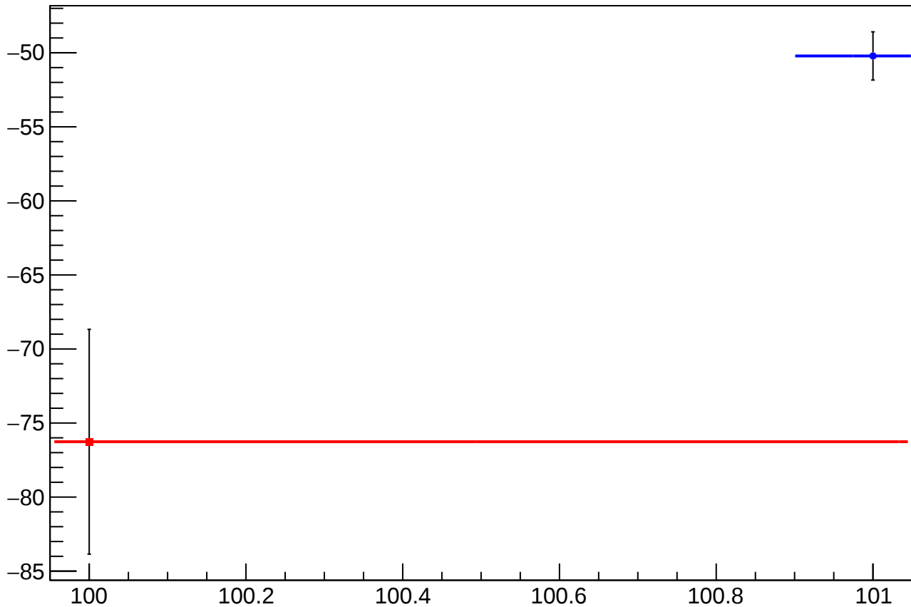
reg_asym_sam_12345678_avg_diff_bpm4aX_slope vs Slug
