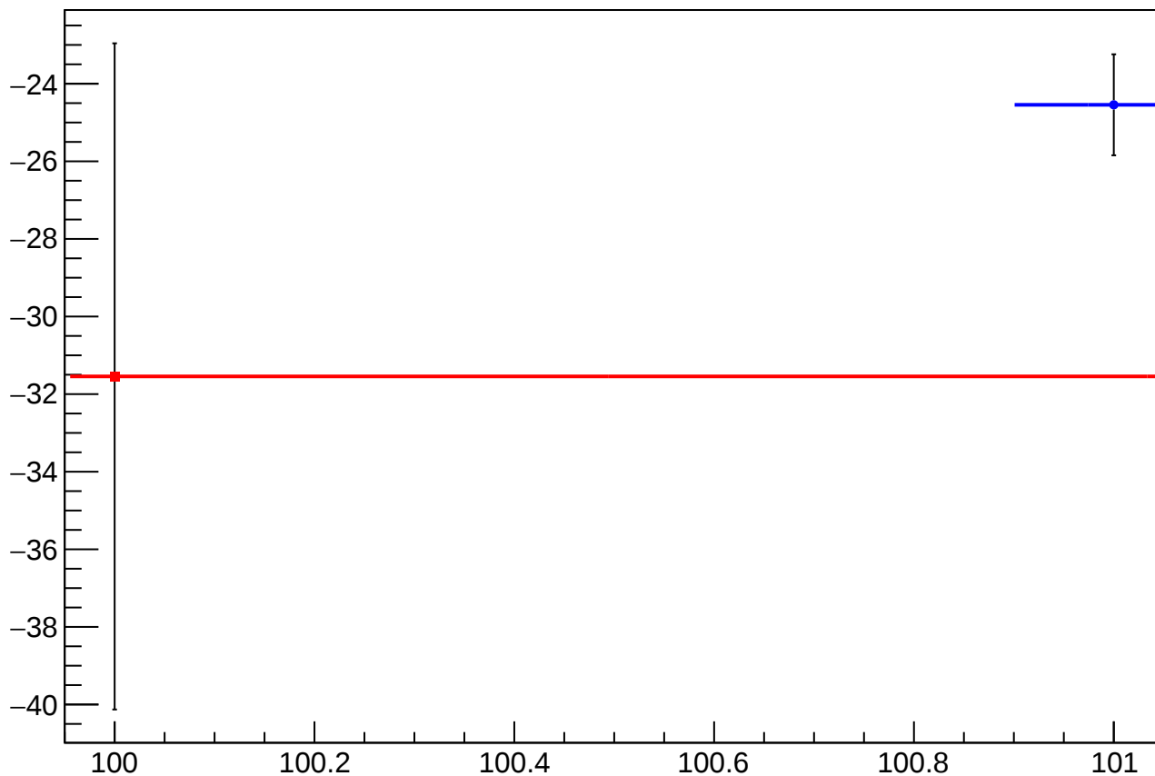
reg_asym_left_avg_diff_bpm4aX_slope vs Slug
