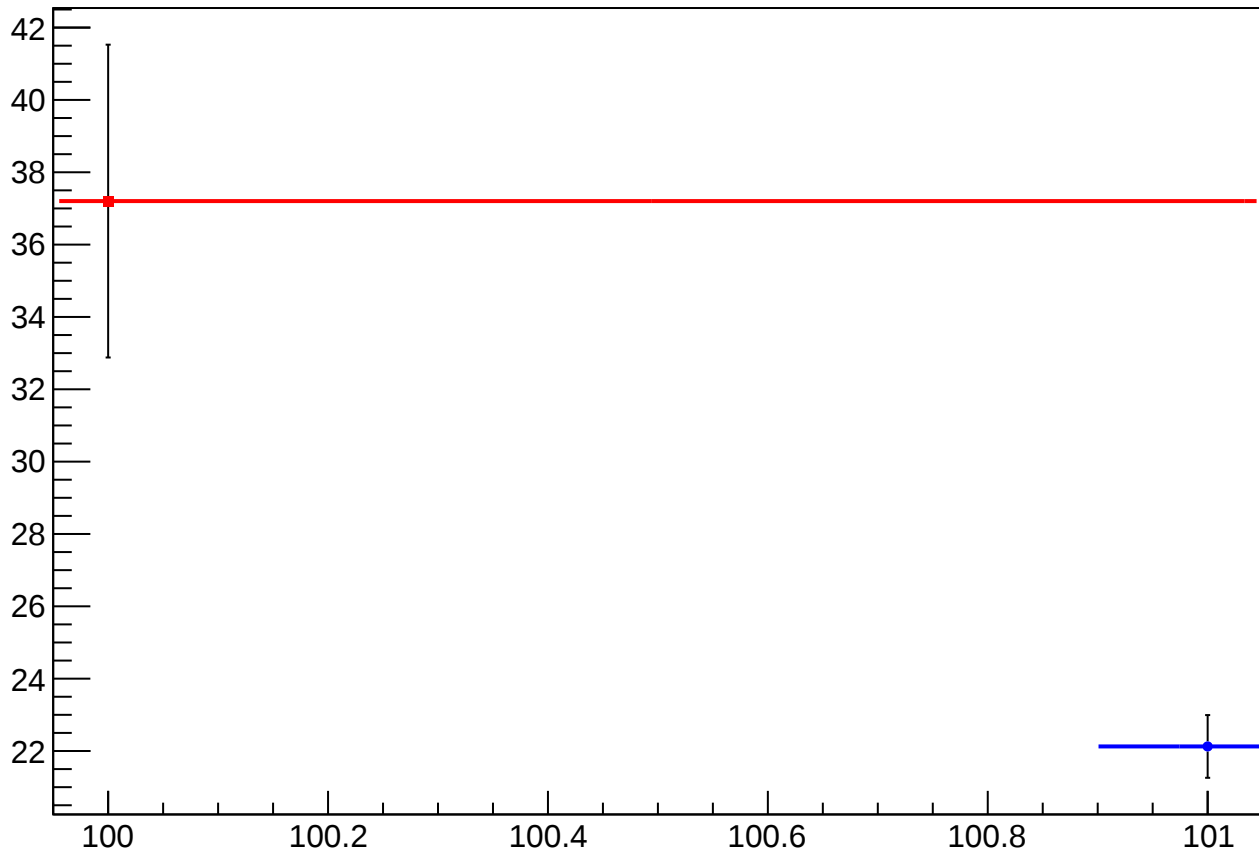
reg_asym_sam_15_37_dd_diff_bpm4aX_slope vs Slug
