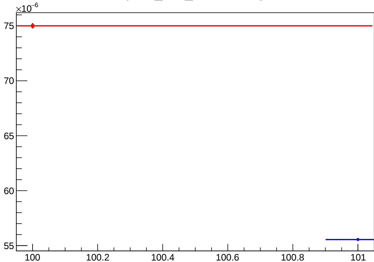
yield_atl1_rms vs Slug
