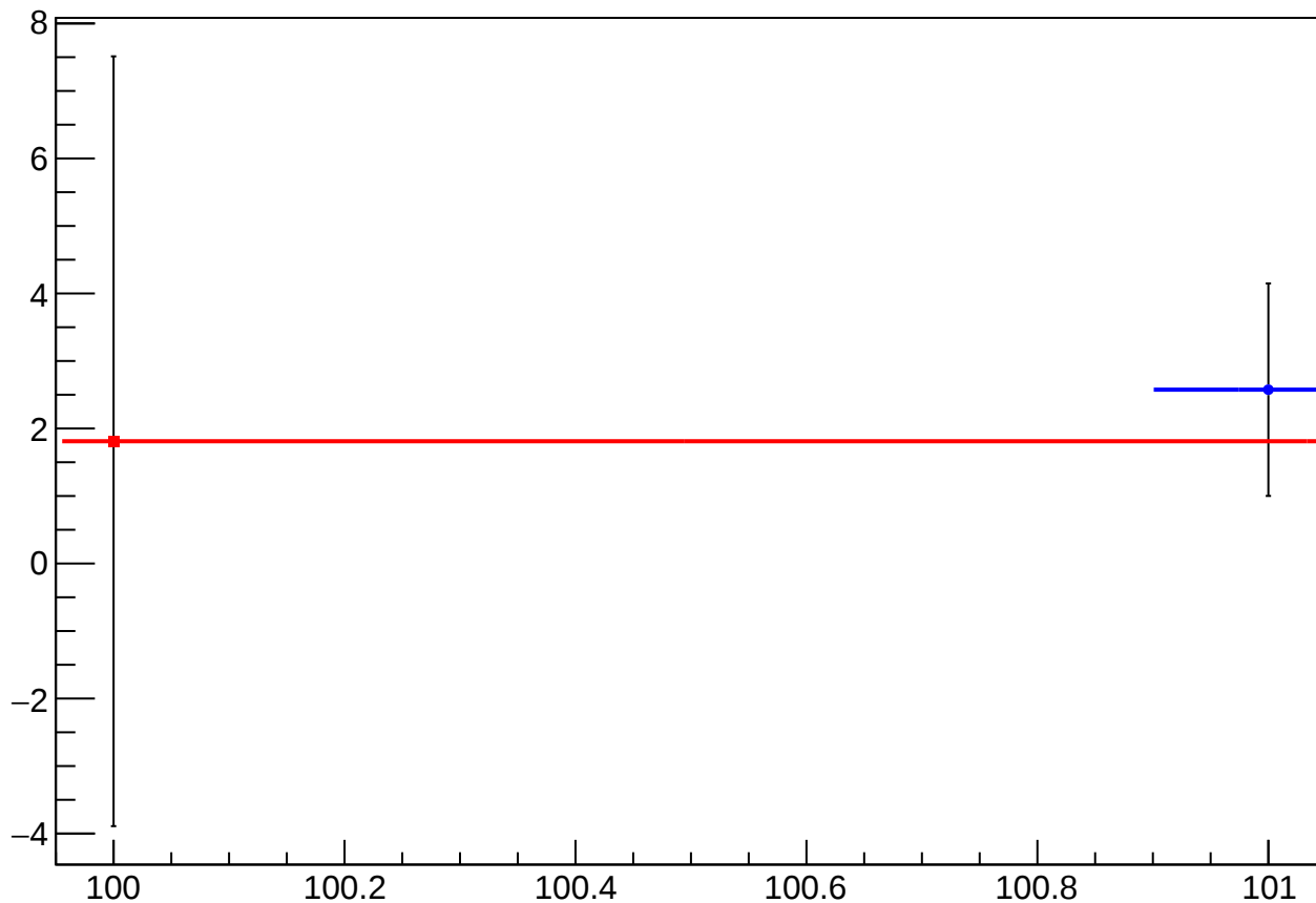
reg_asym_sam_48_dd_diff_bpm4eX_slope vs Slug
