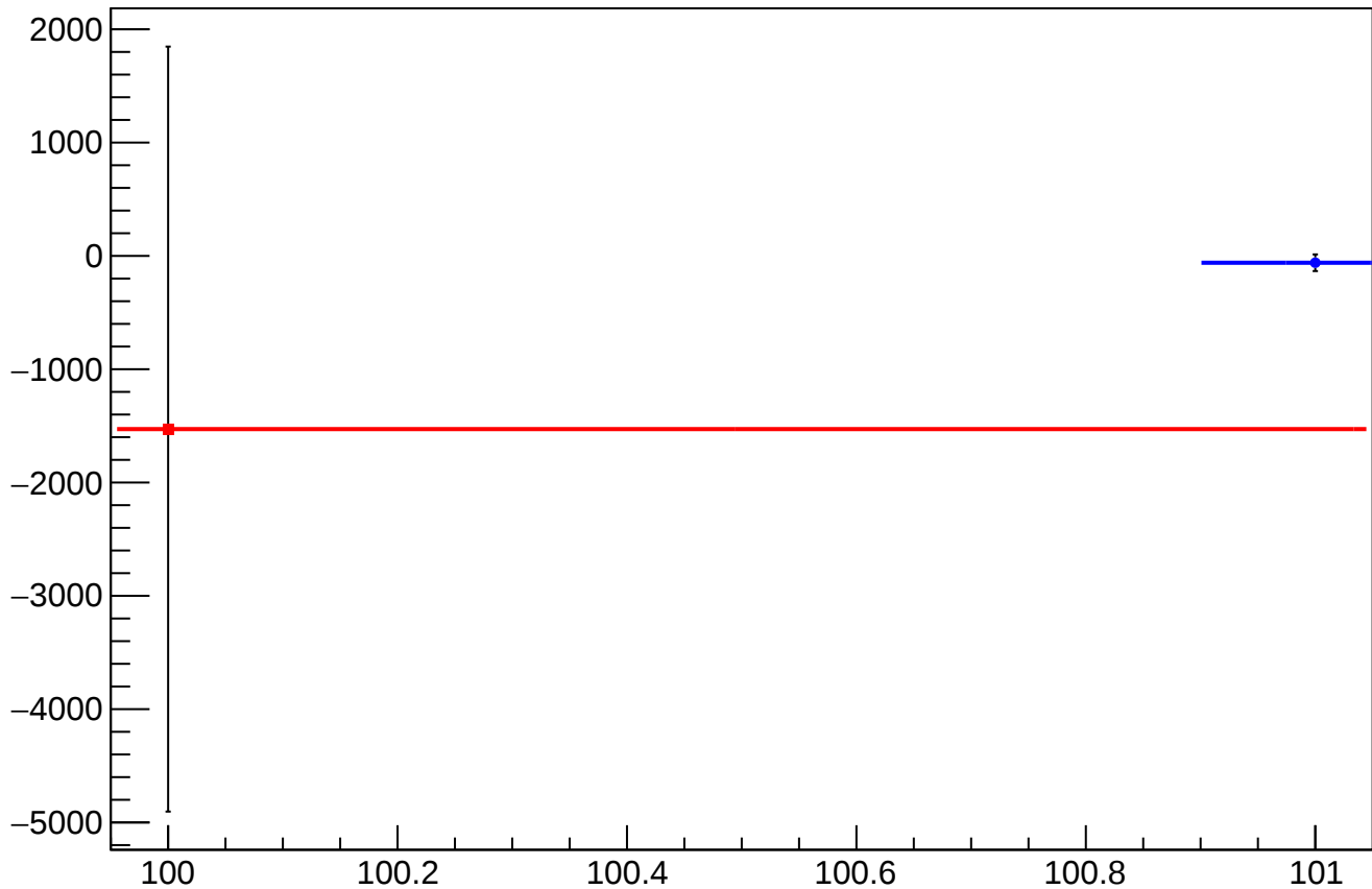
reg_asym_ds_avg_mean vs Slug
