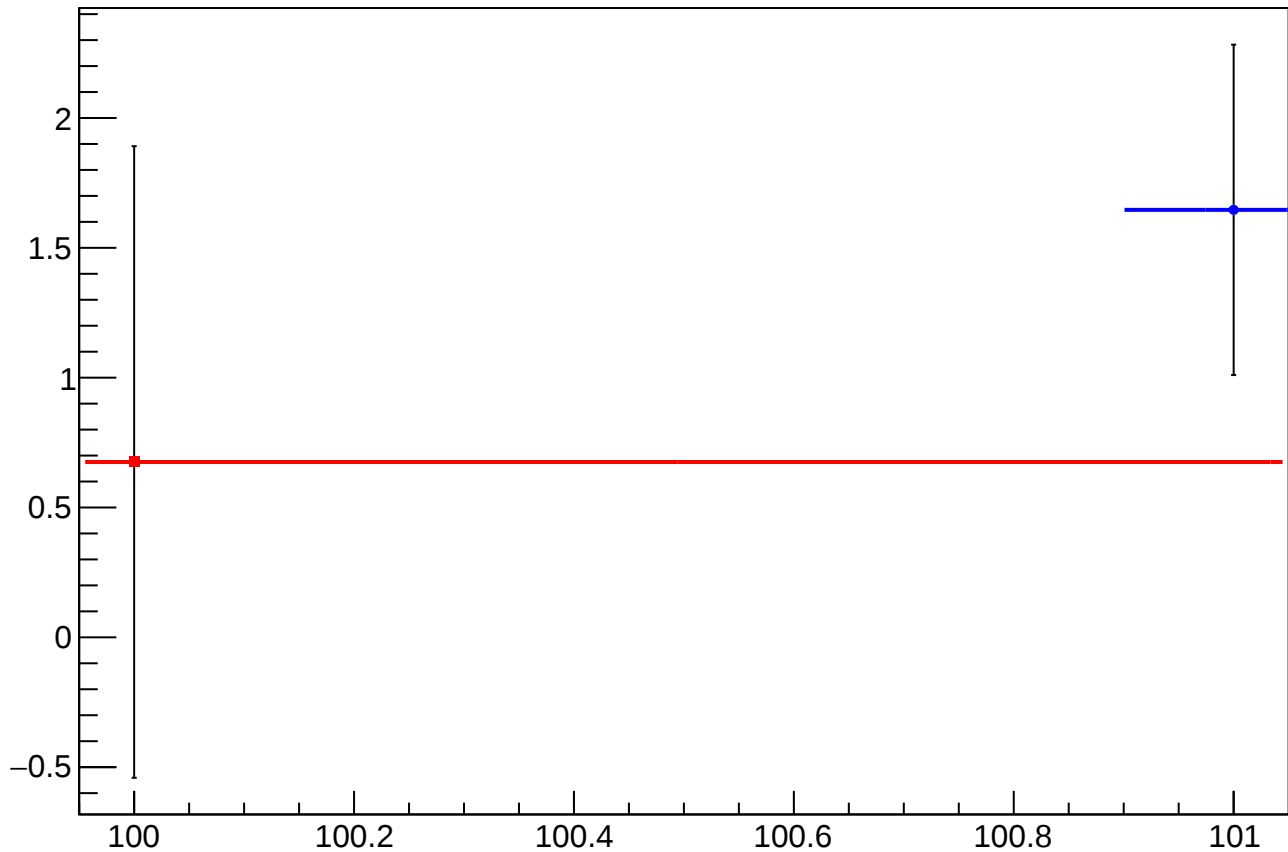
reg_asym_left_dd_diff_bpm4aY_slope vs Slug
