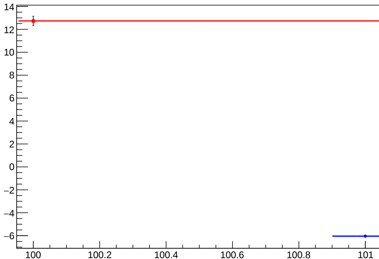
reg_asym_sam_15_avg_diff_bpm4eY_slope vs Slug
