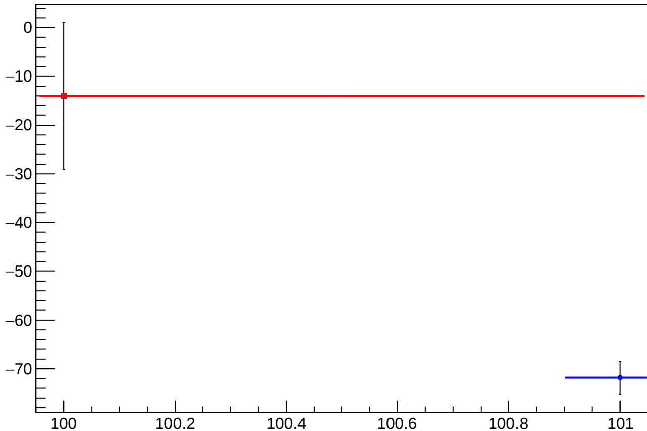
reg_asym_sam_26_avg_diff_bpm4eX_slope vs Slug
