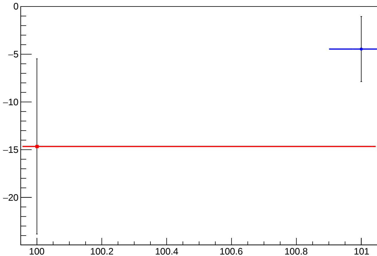
asym_cav4bQ_mean vs Slug, Sign Corrected
