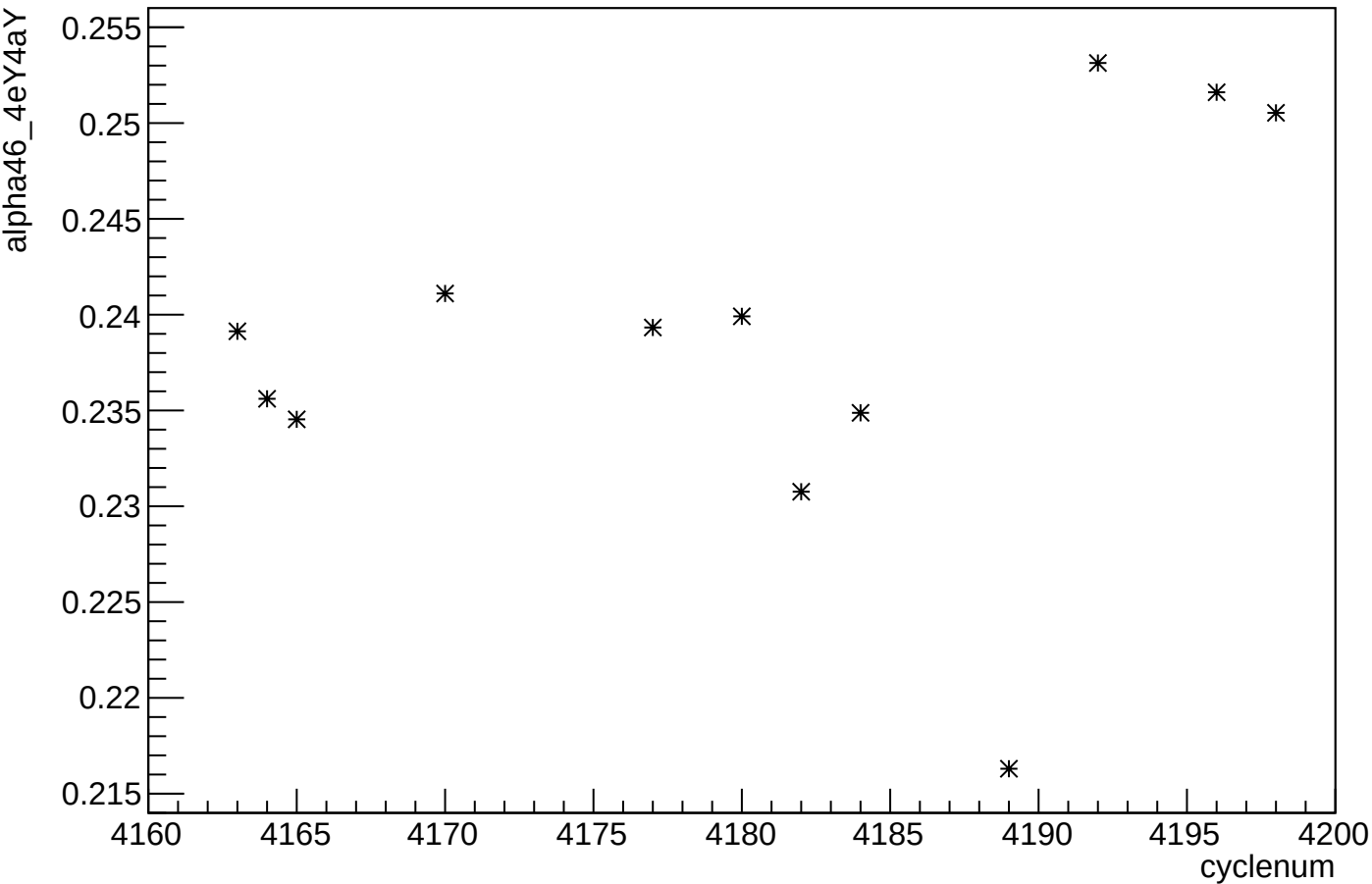
alpha46_4eY4aY:cyclenum
