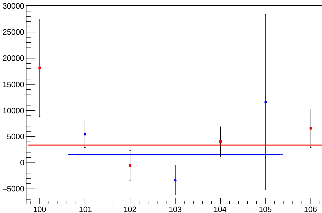
asym_sam4_mean vs slug
