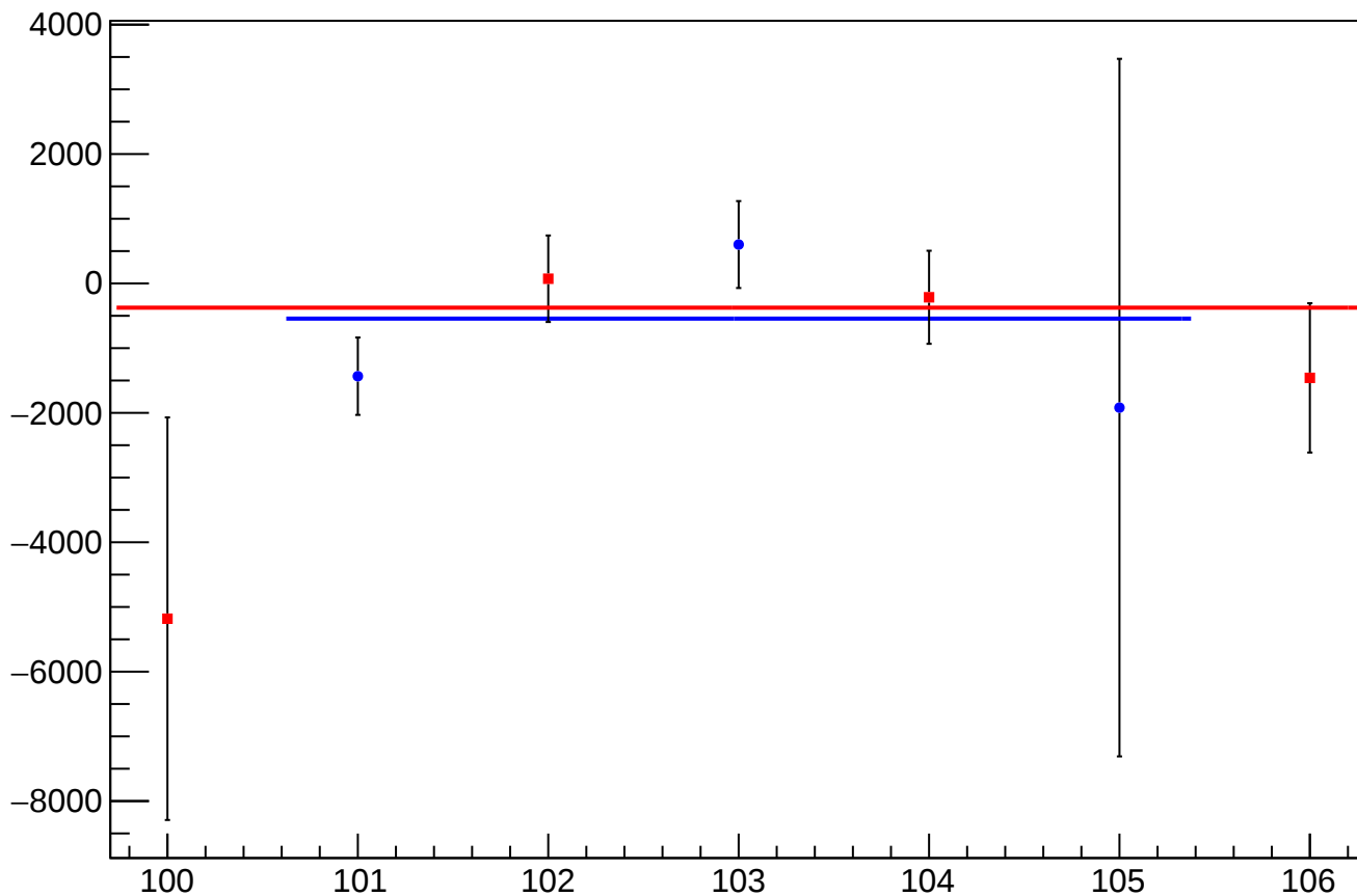
asym_sam_1357_avg_correction_mean vs slug
