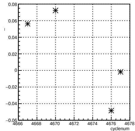
delta46_11X12X4eY:cyclenum
