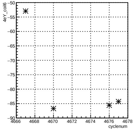
4eY_coil6:cyclenum
