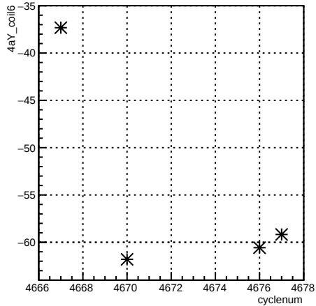
4aY_coil6:cyclenum
