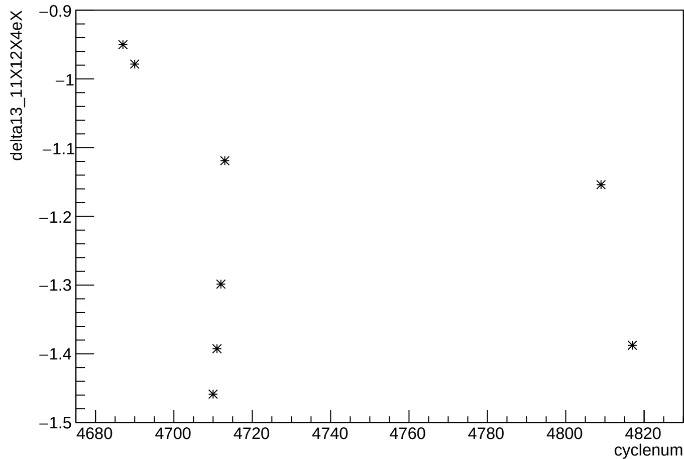
delta13_11X12X4eX:cyclenum
