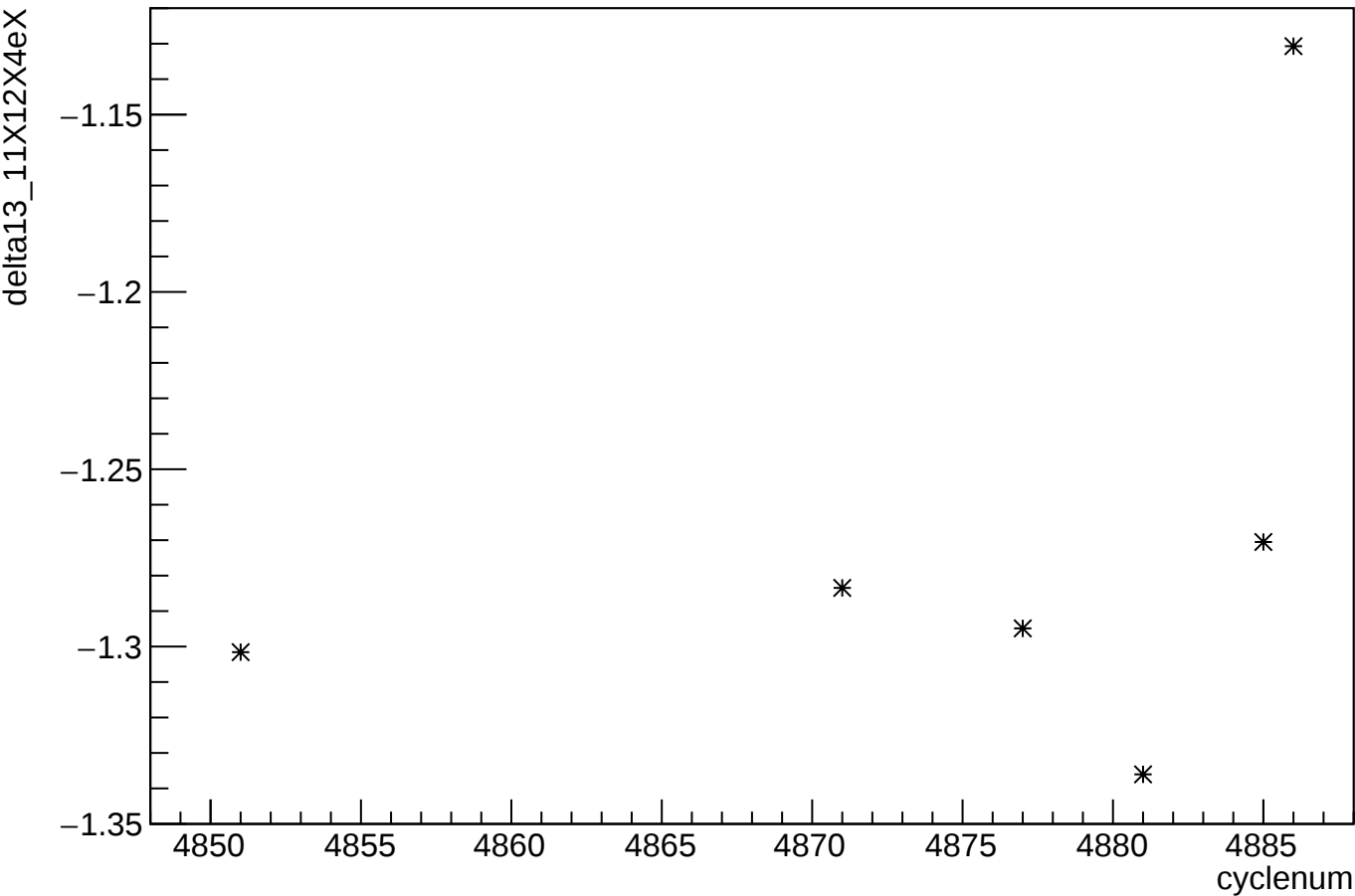
delta13_11X12X4eX:cyclenum
