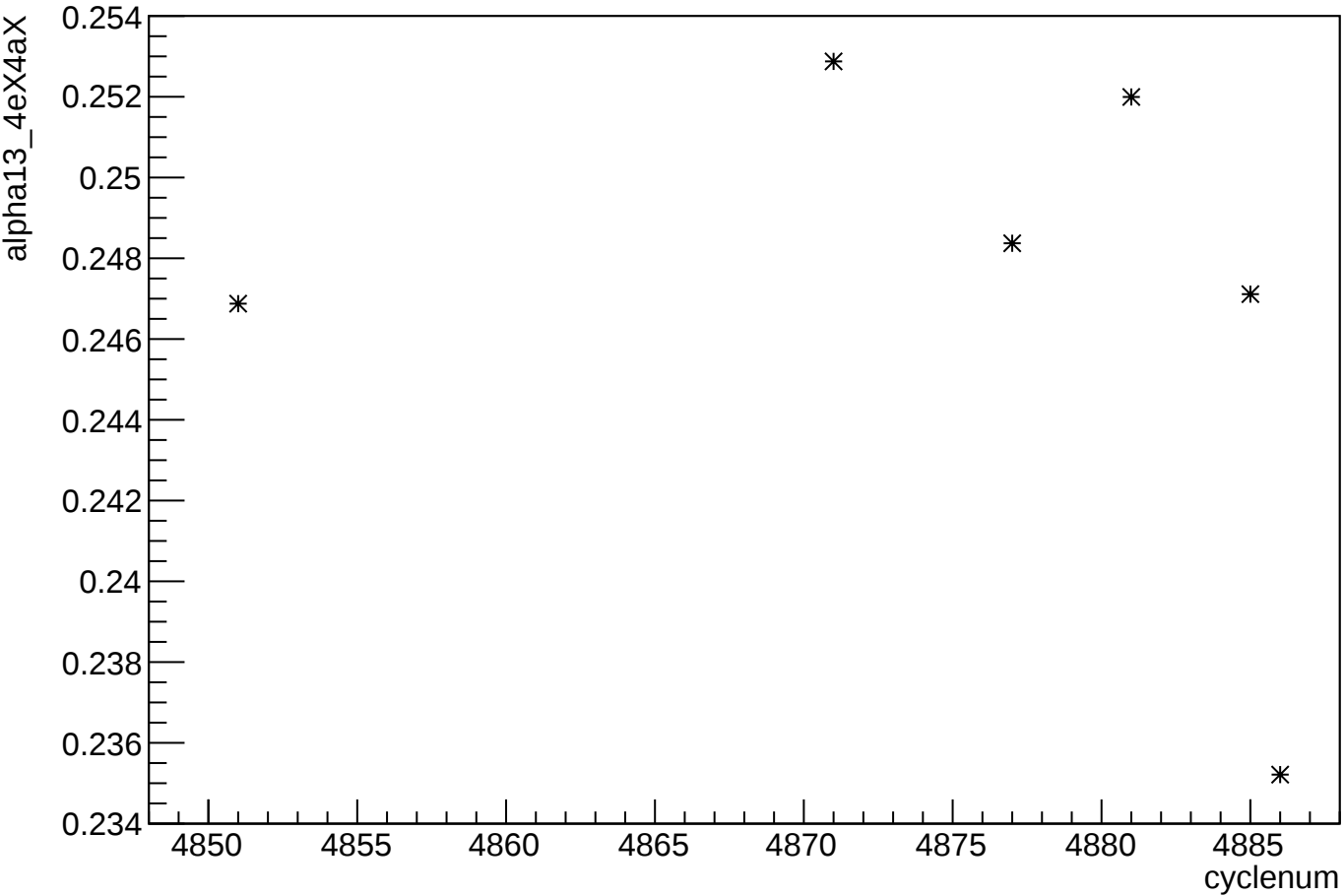
alpha13_4eX4aX:cyclenum
