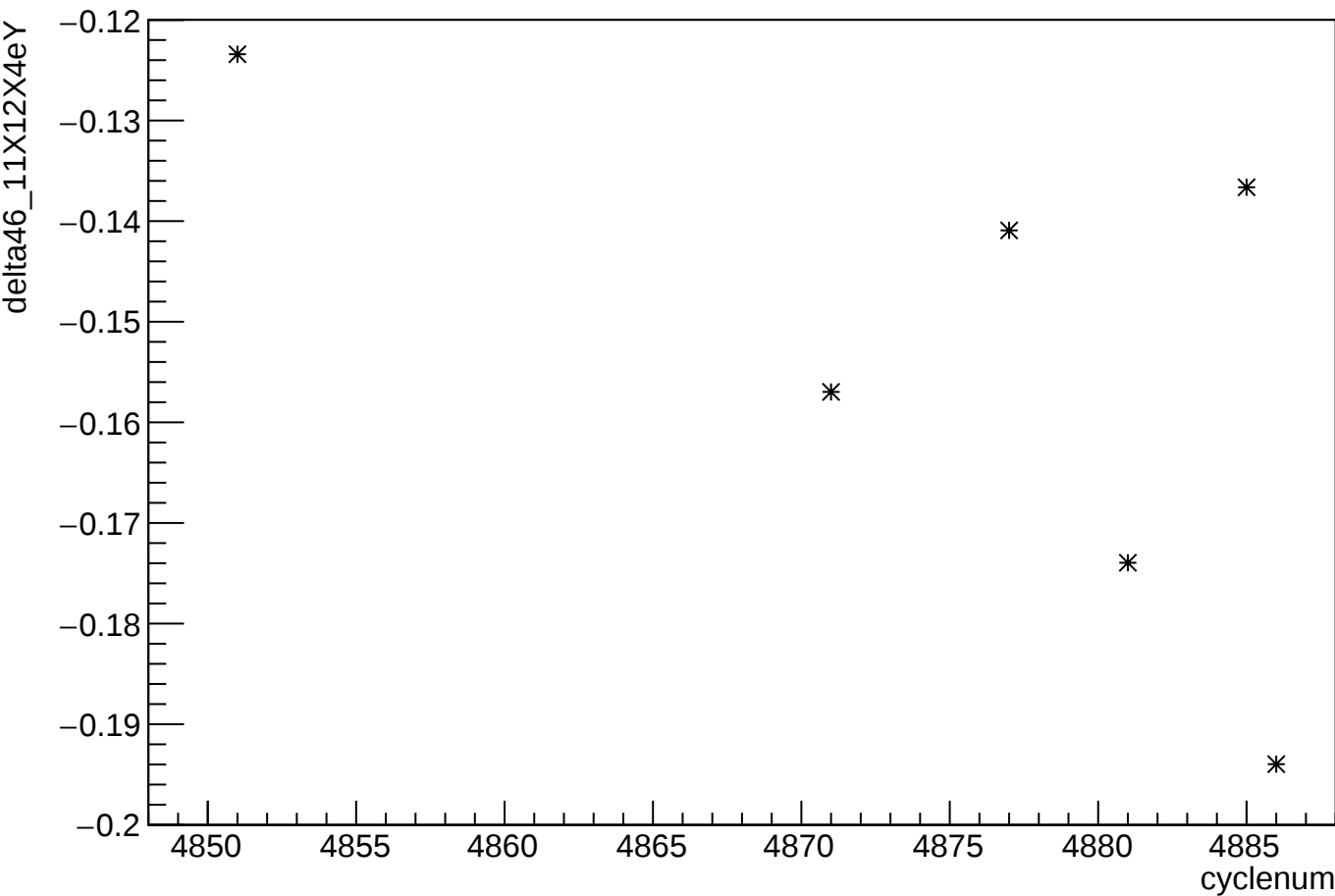
delta46_11X12X4eY:cyclenum
