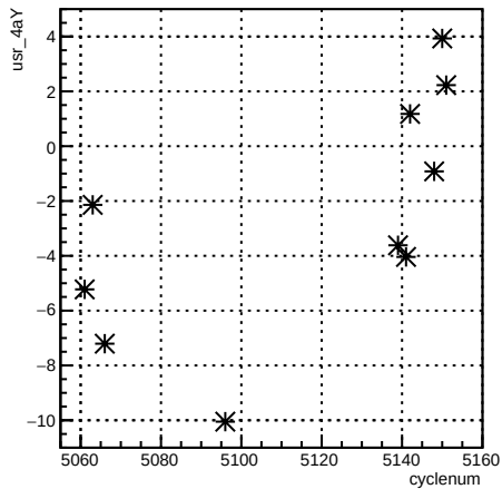
usr_4aY:cyclenum
