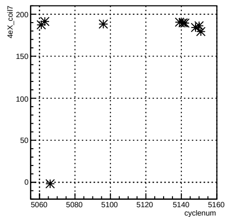
4eX_coil7:cyclenum
