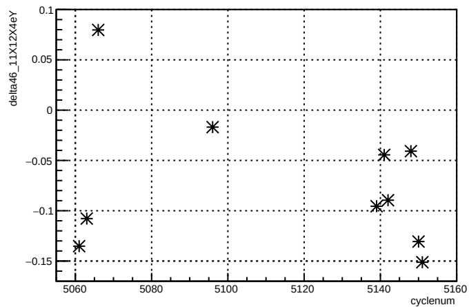
delta46_11X12X4eY:cyclenum
