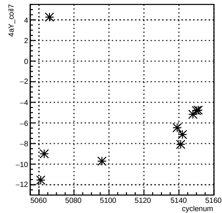
4aY_coil7:cyclenum
