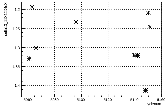
delta13_11X12X4eX:cyclenum
