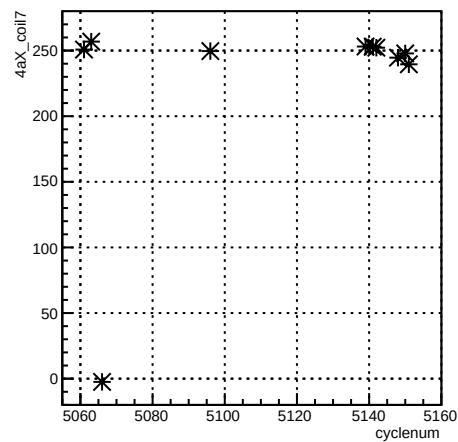
4aX_coil7:cyclenum
