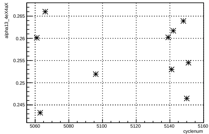
alpha13_4eX4aX:cyclenum
