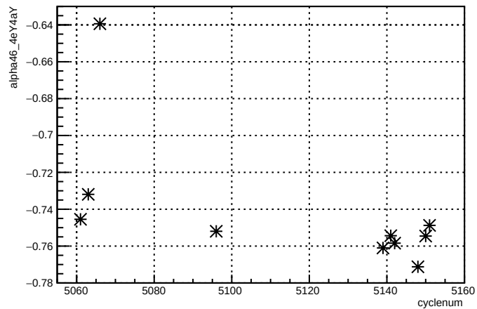
alpha46_4eY4aY:cyclenum
