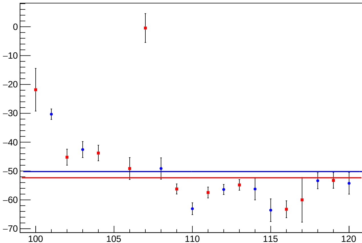
reg_asym_us_dd_diff_bpm4eX_slope vs Slug
