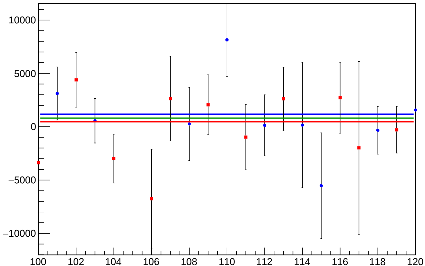
reg_asym_atl_avg_mean vs Slug, Sign Corrected
