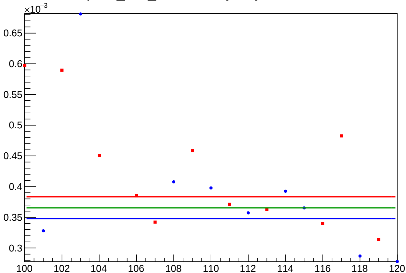
yield_atl2_rms vs Slug, Sign Corrected
