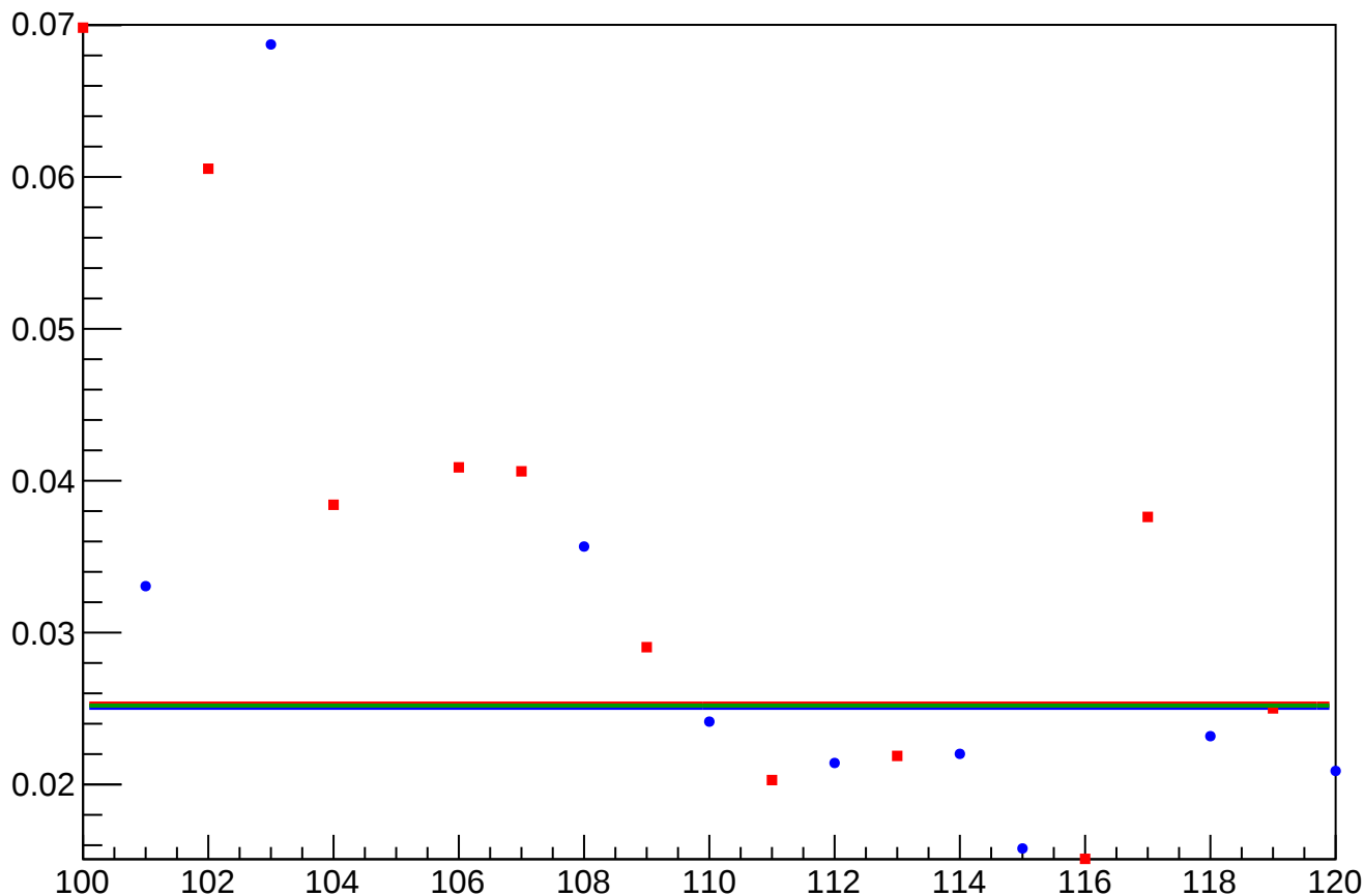
yield_bpm4acX_rms vs Slug, Sign Corrected
