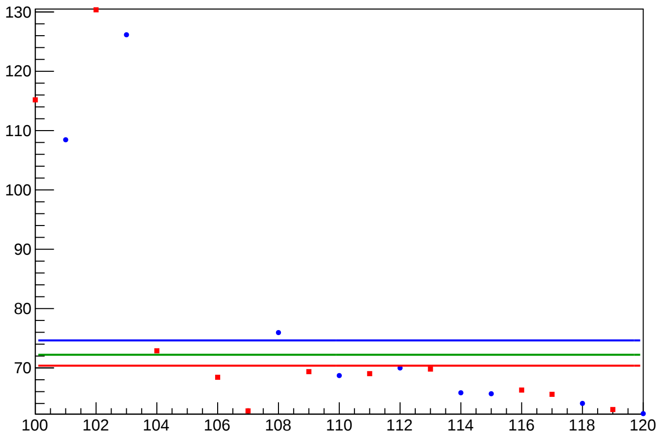
reg_asym_sam7_rms vs Slug, Sign Corrected
