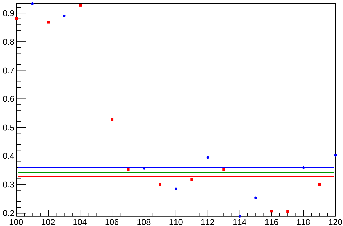
yield_bcm_an_us_rms vs Slug, Sign Corrected
