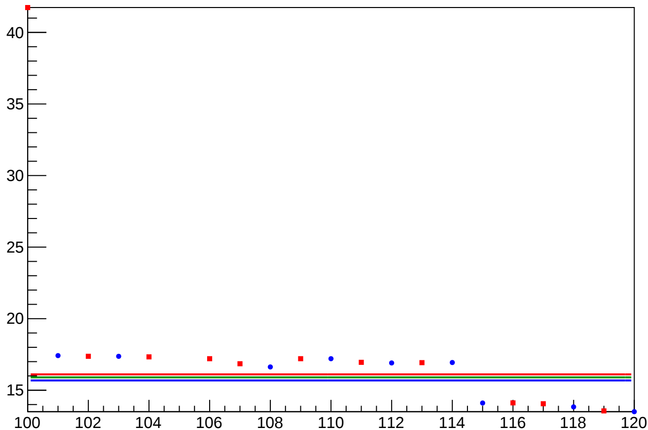
yield_sam4_mean vs Slug, Sign Corrected
