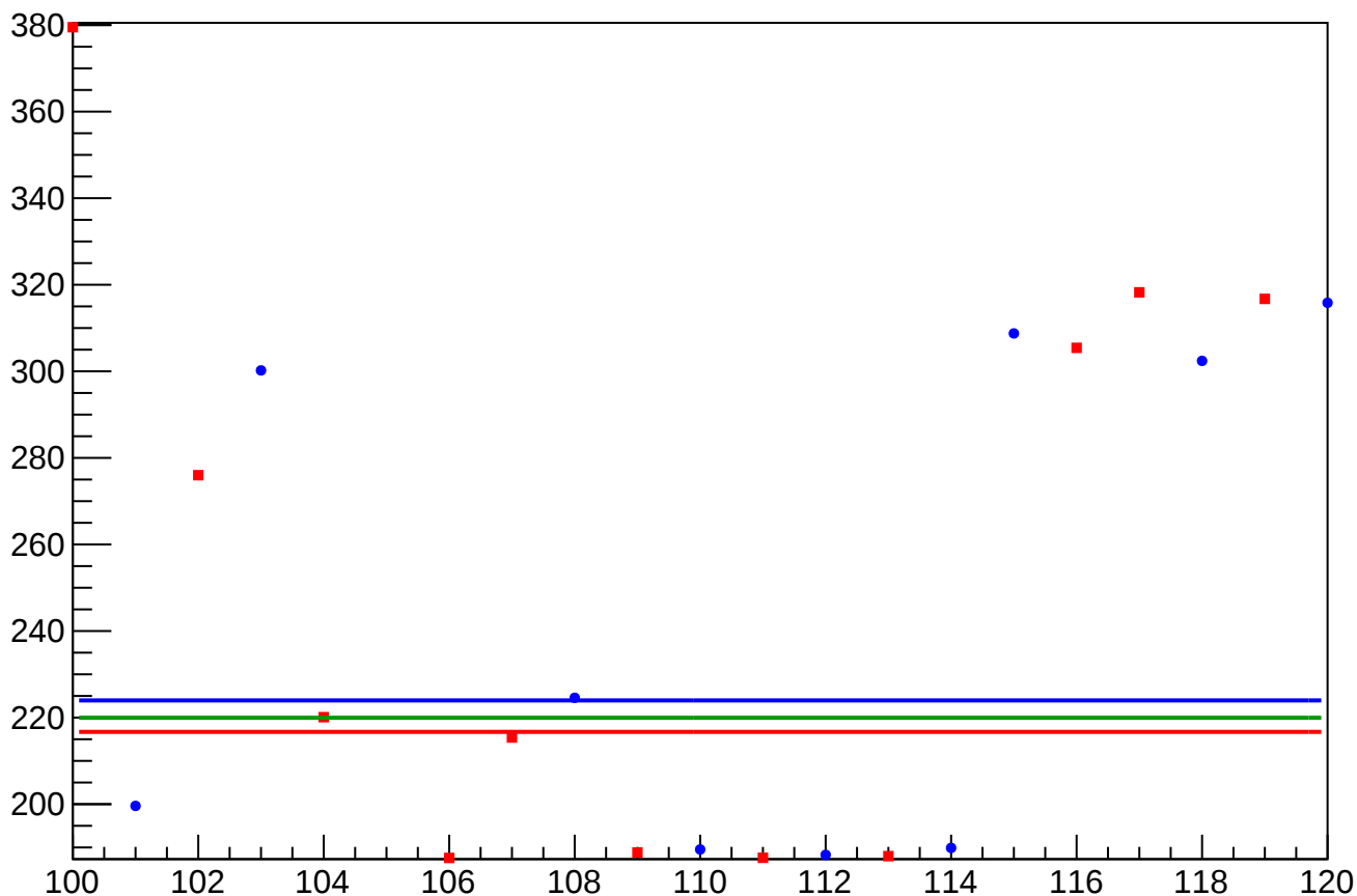
reg_asym_sam4_rms vs Slug, Sign Corrected
