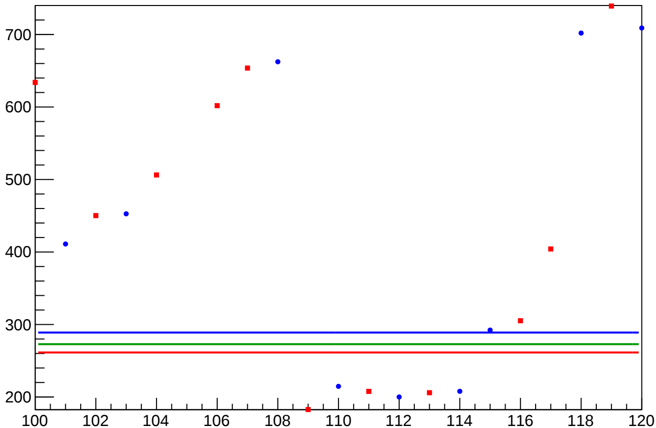
asym_sam7_rms vs Slug, Sign Corrected
