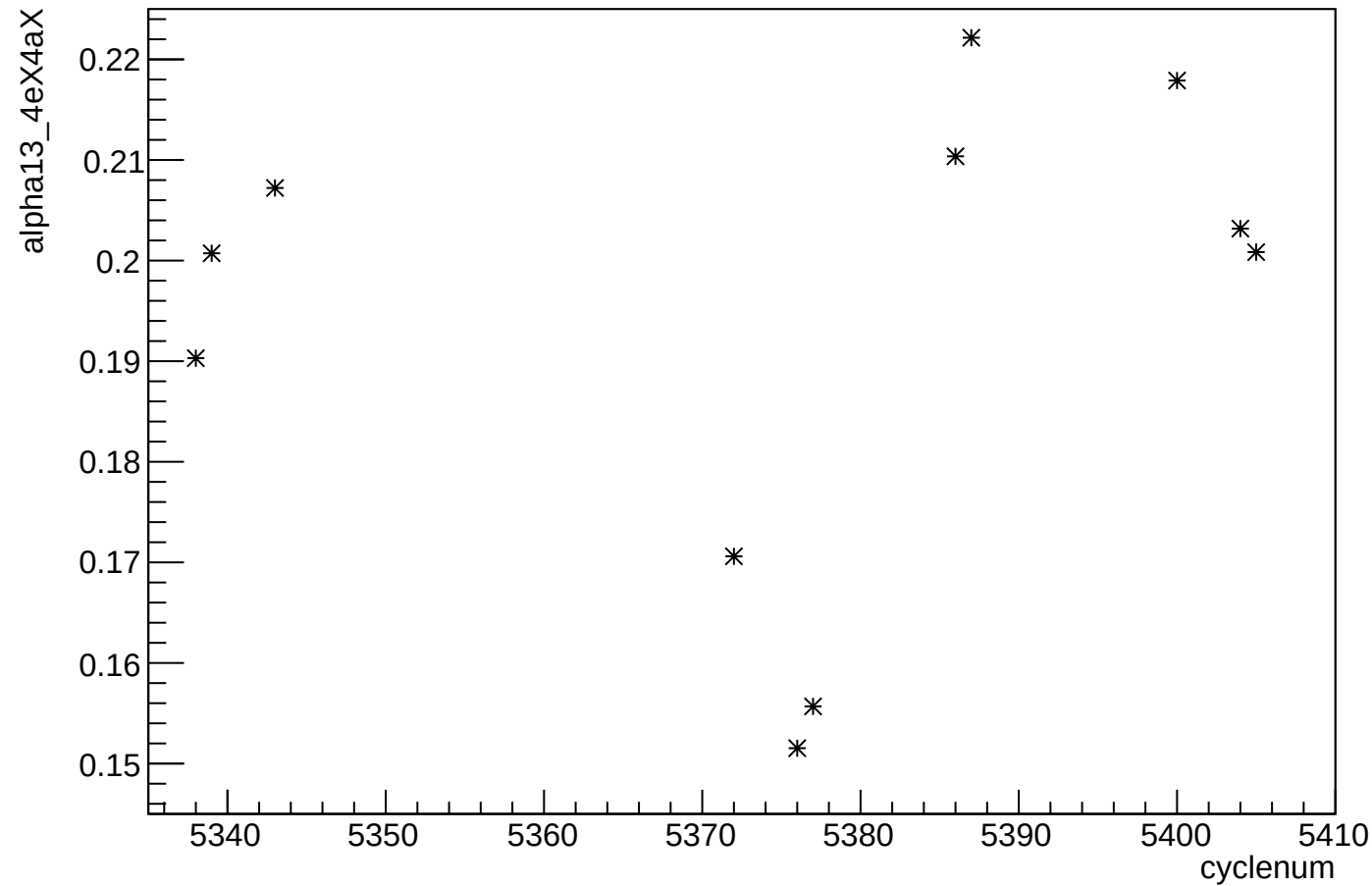
alpha13_4eX4aX:cyclenum
