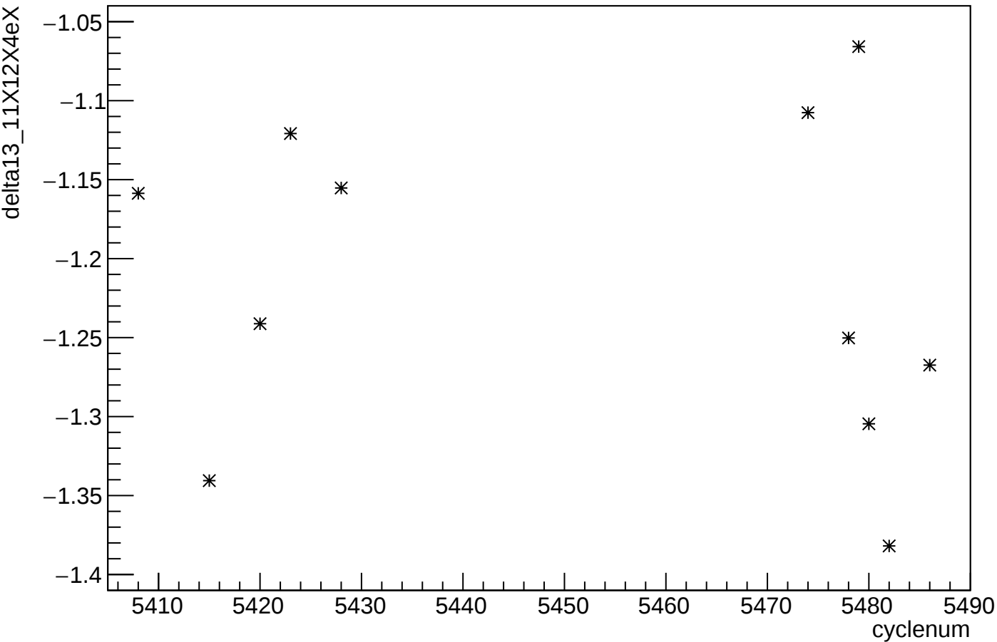
delta13_11X12X4eX:cyclenum
