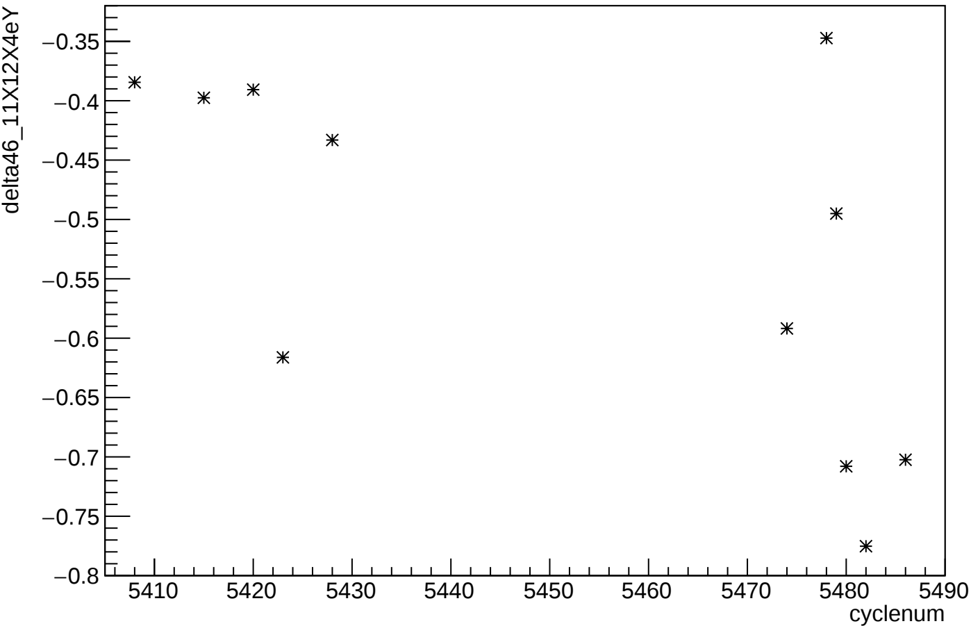
delta46_11X12X4eY:cyclenum
