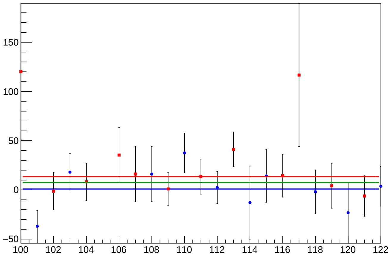
diff_bpm4eX_mean vs Slug, Sign Corrected
