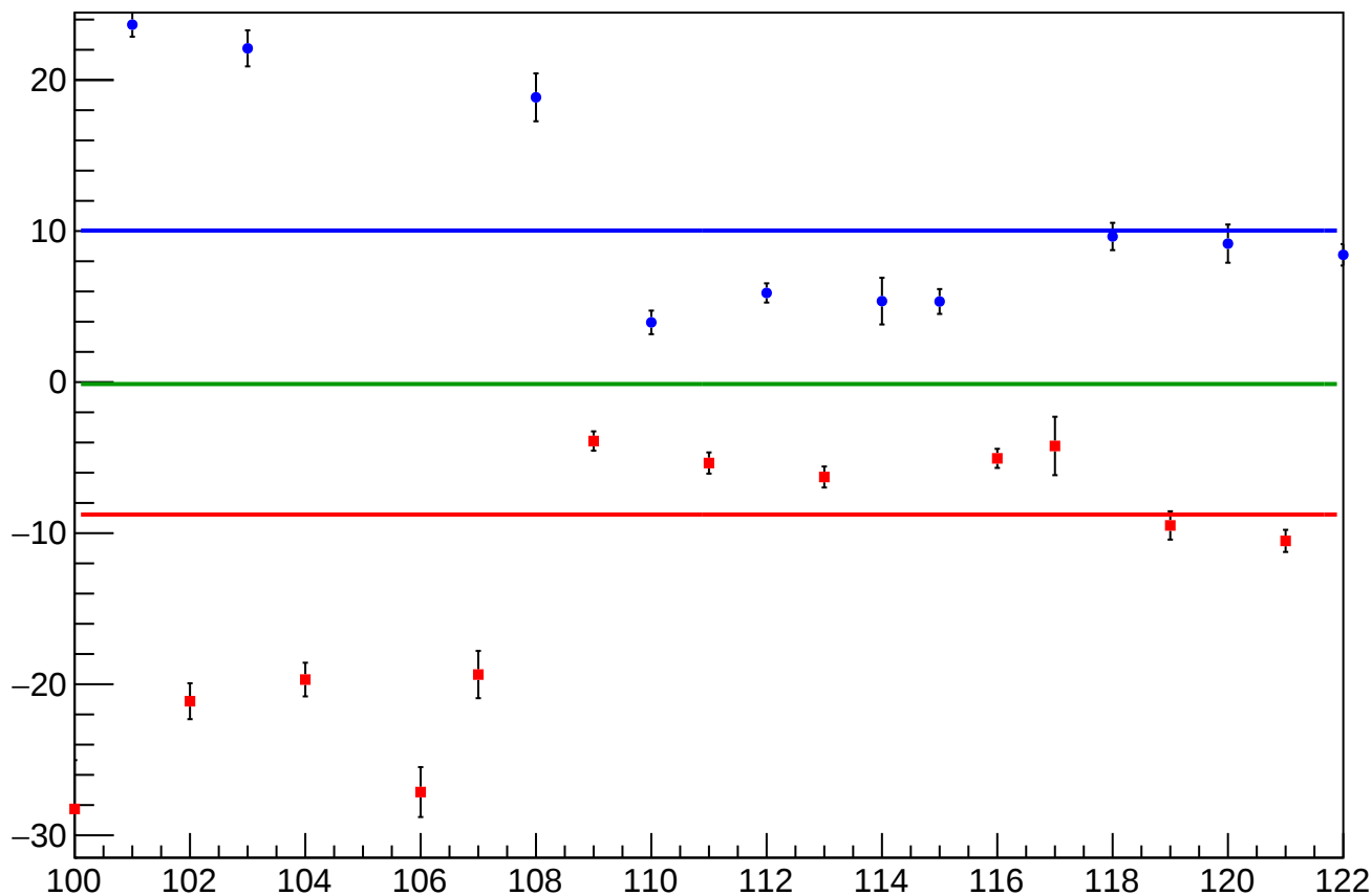
reg_asym_sam_1357_2468_dd_diff_bpm4aX_slope vs Slug, Sign Corrected
