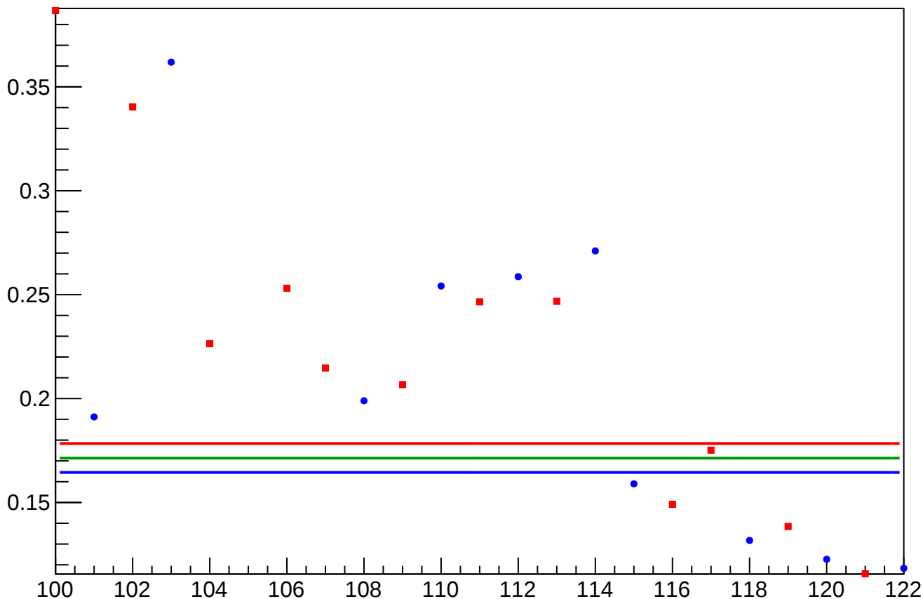
yield_sam2_rms vs Slug, Sign Corrected
