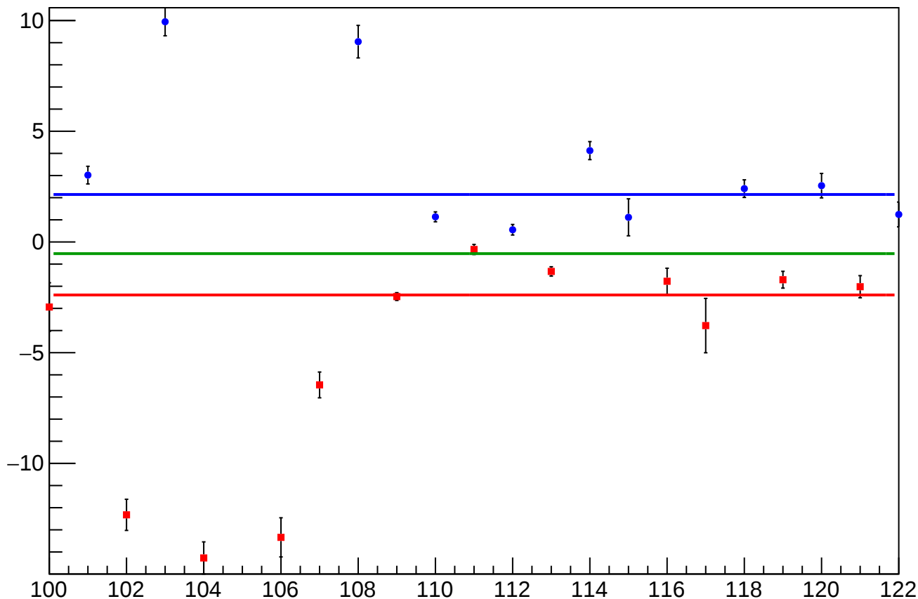
reg_asym_bcm_dg_us_diff_bpm4aX_slope vs Slug, Sign Corrected
