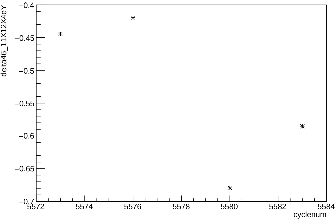
delta46_11X12X4eY:cyclenum
