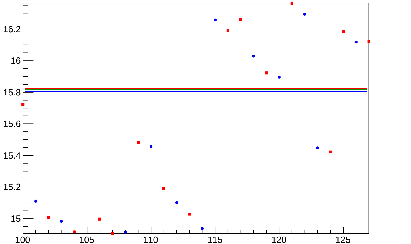
yield_sam1_mean vs Slug, Sign Corrected
