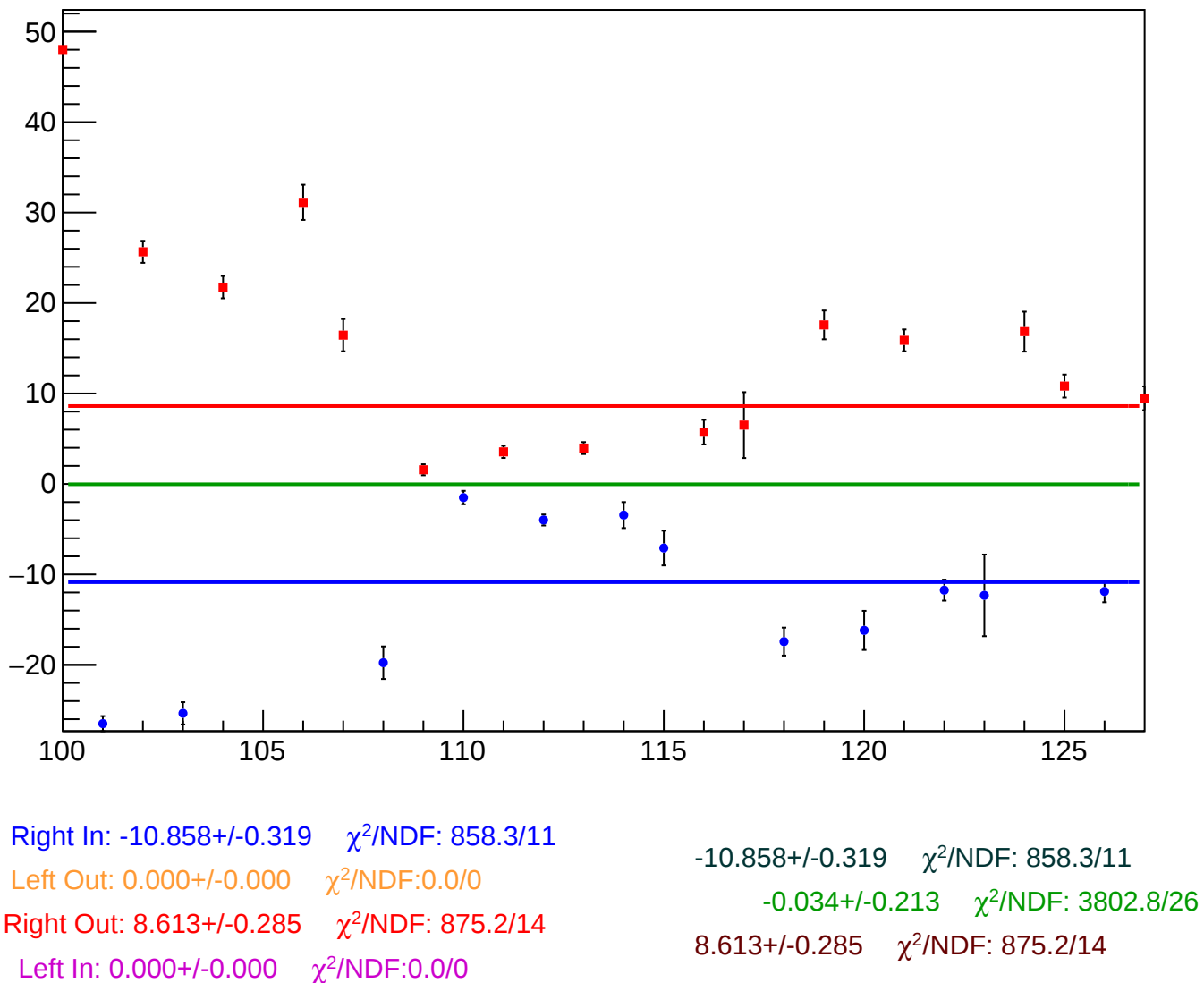
reg_asym_sam_1357_avg_diff_bpm4aX_slope vs Slug, Sign Corrected
