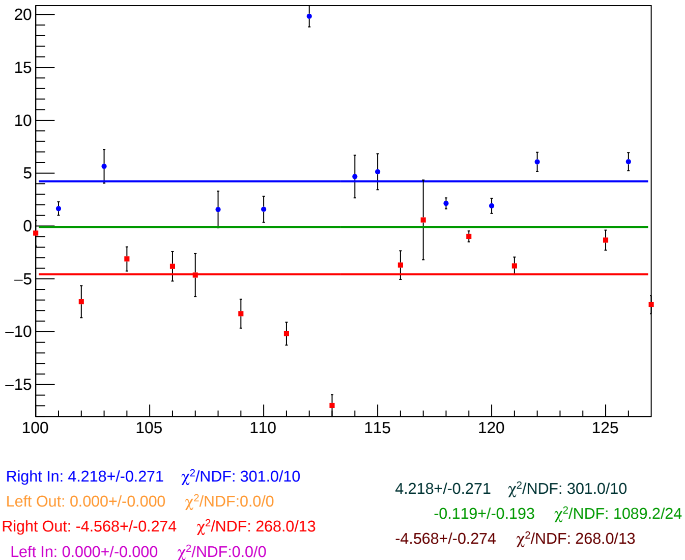
reg_asym_left_dd_diff_bpm4aY_slope vs Slug, Sign Corrected
