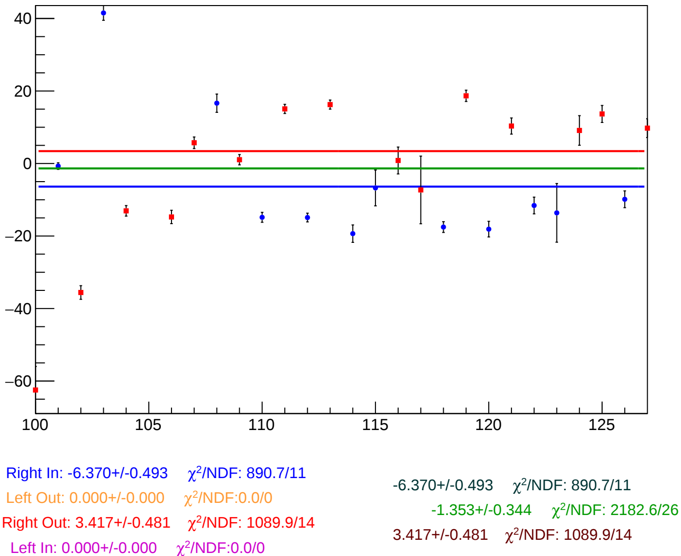
reg_asym_sam_48_avg_diff_bpm4aY_slope vs Slug, Sign Corrected
