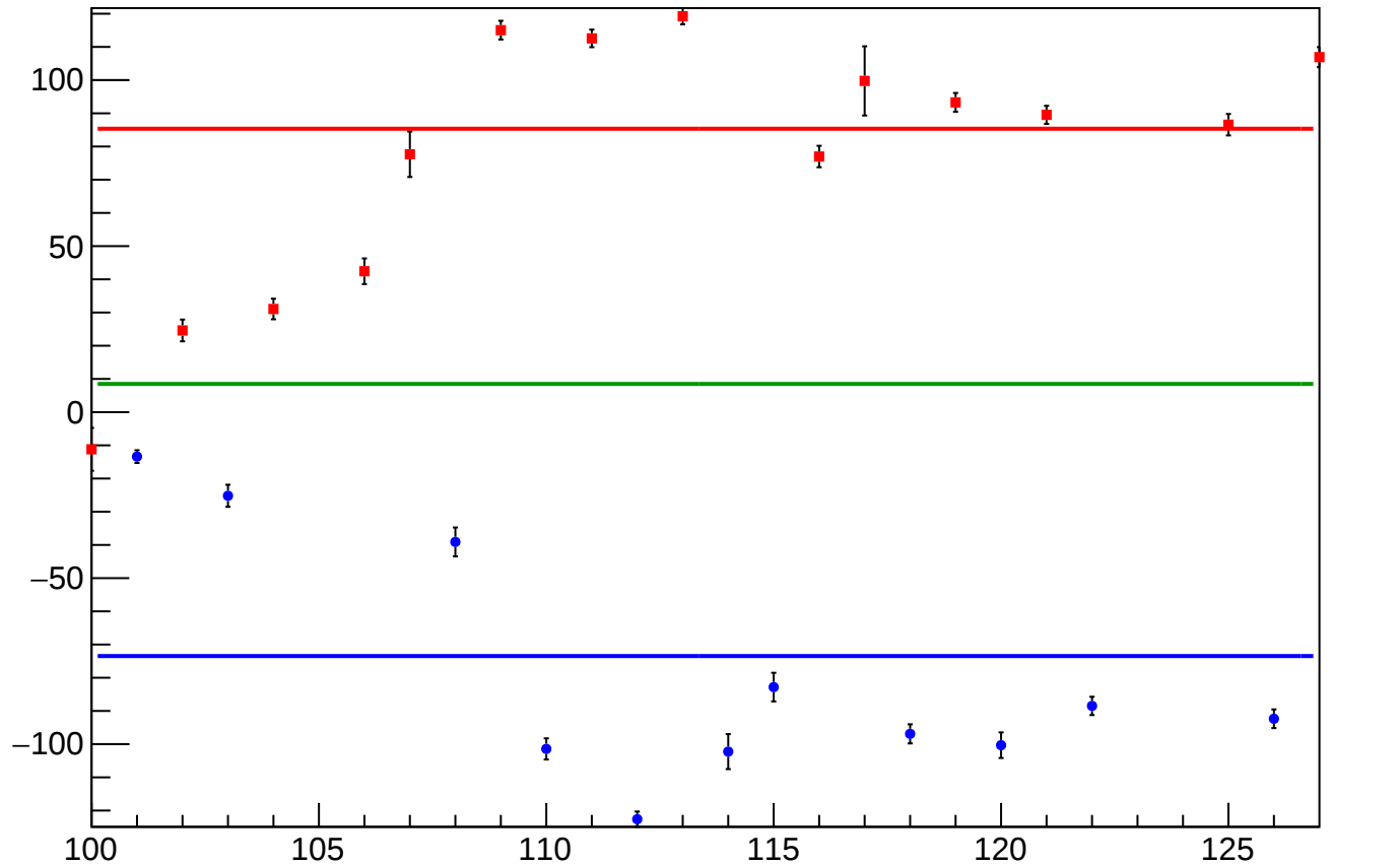
reg_asym_us_avg_diff_bpm4aX_slope vs Slug, Sign Corrected
