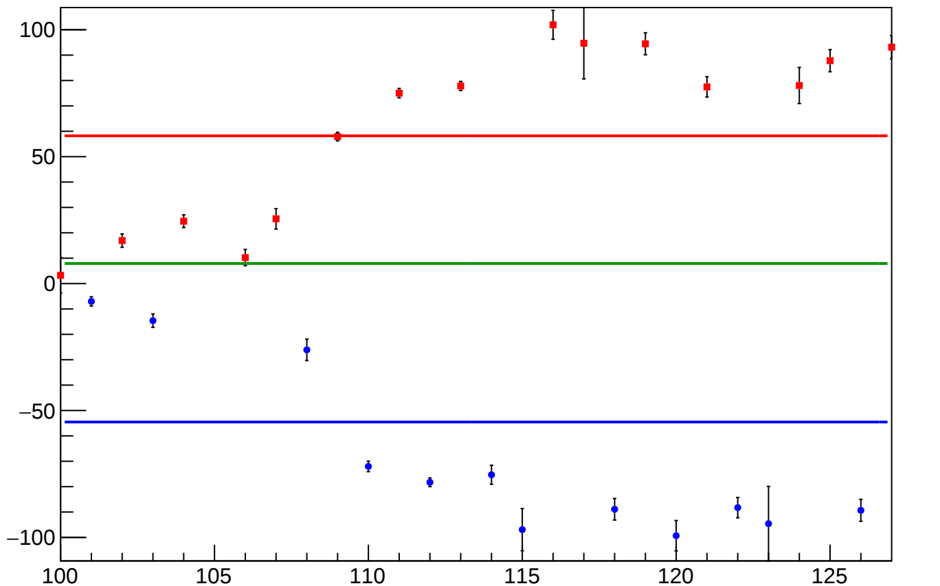
reg_asym_sam_48_avg_diff_bpm4eX_slope vs Slug, Sign Corrected
