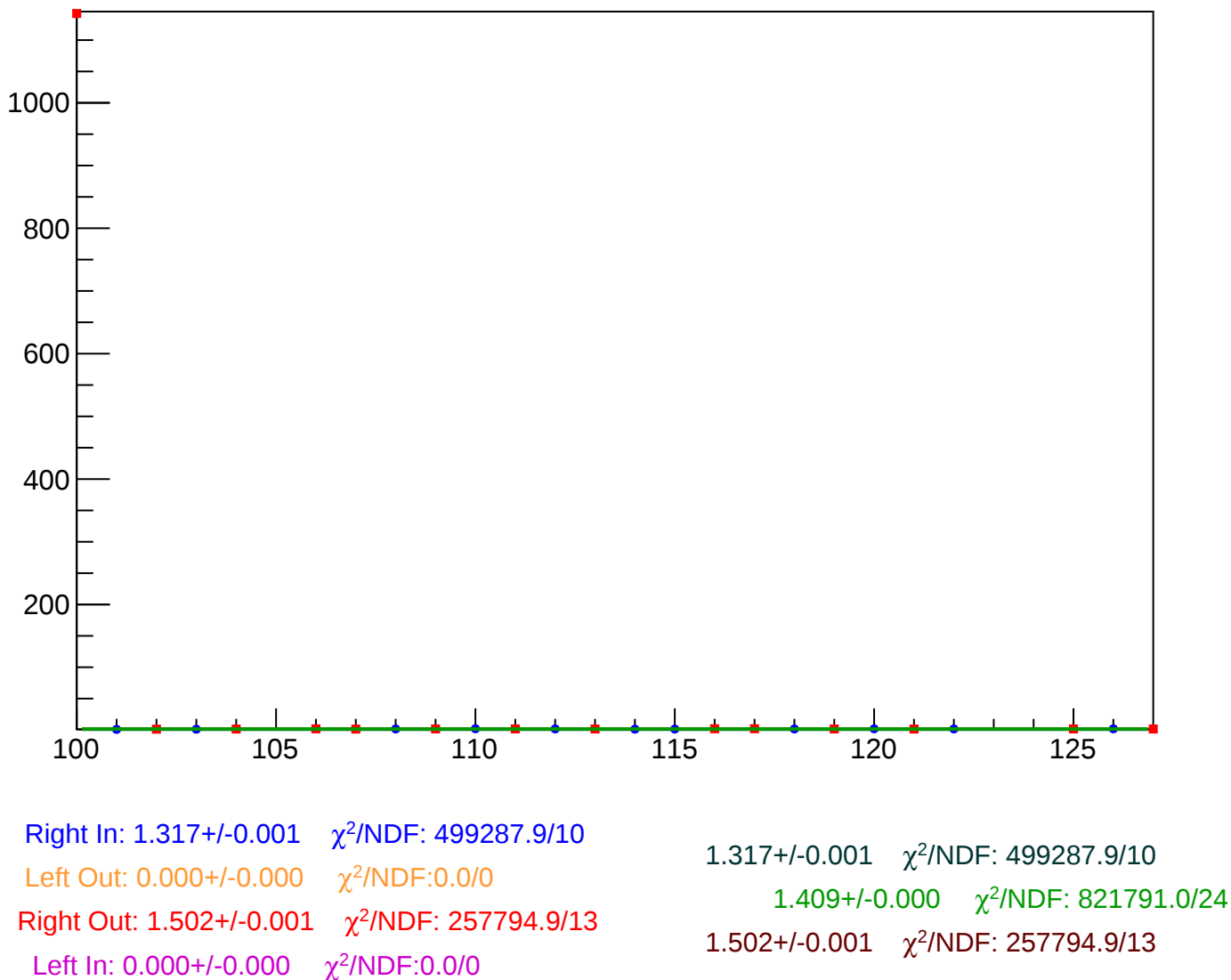
asym_dsl_correction_rms vs Slug, Sign Corrected
