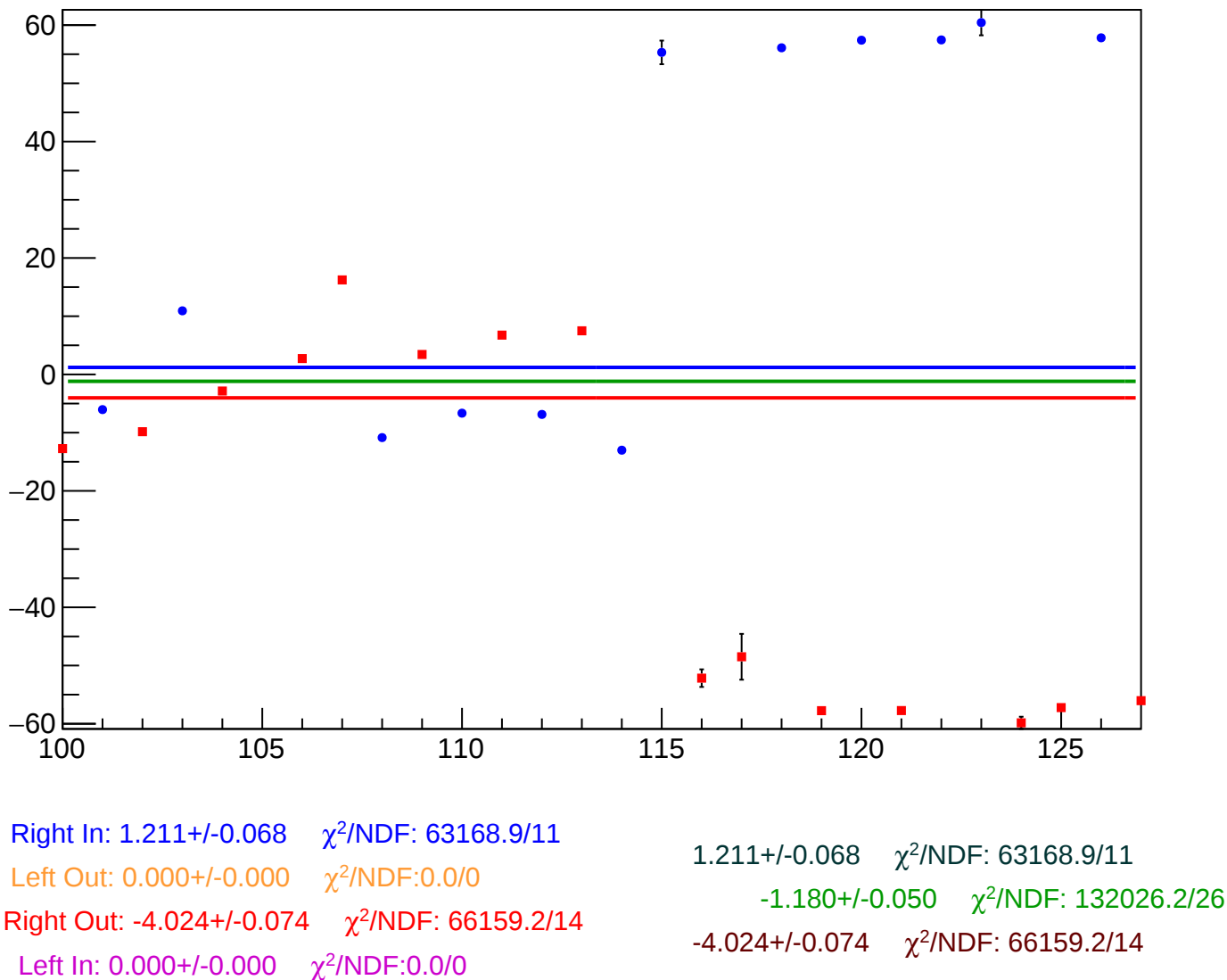
reg_asym_sam_15_avg_diff_bpm4eY_slope vs Slug, Sign Corrected
