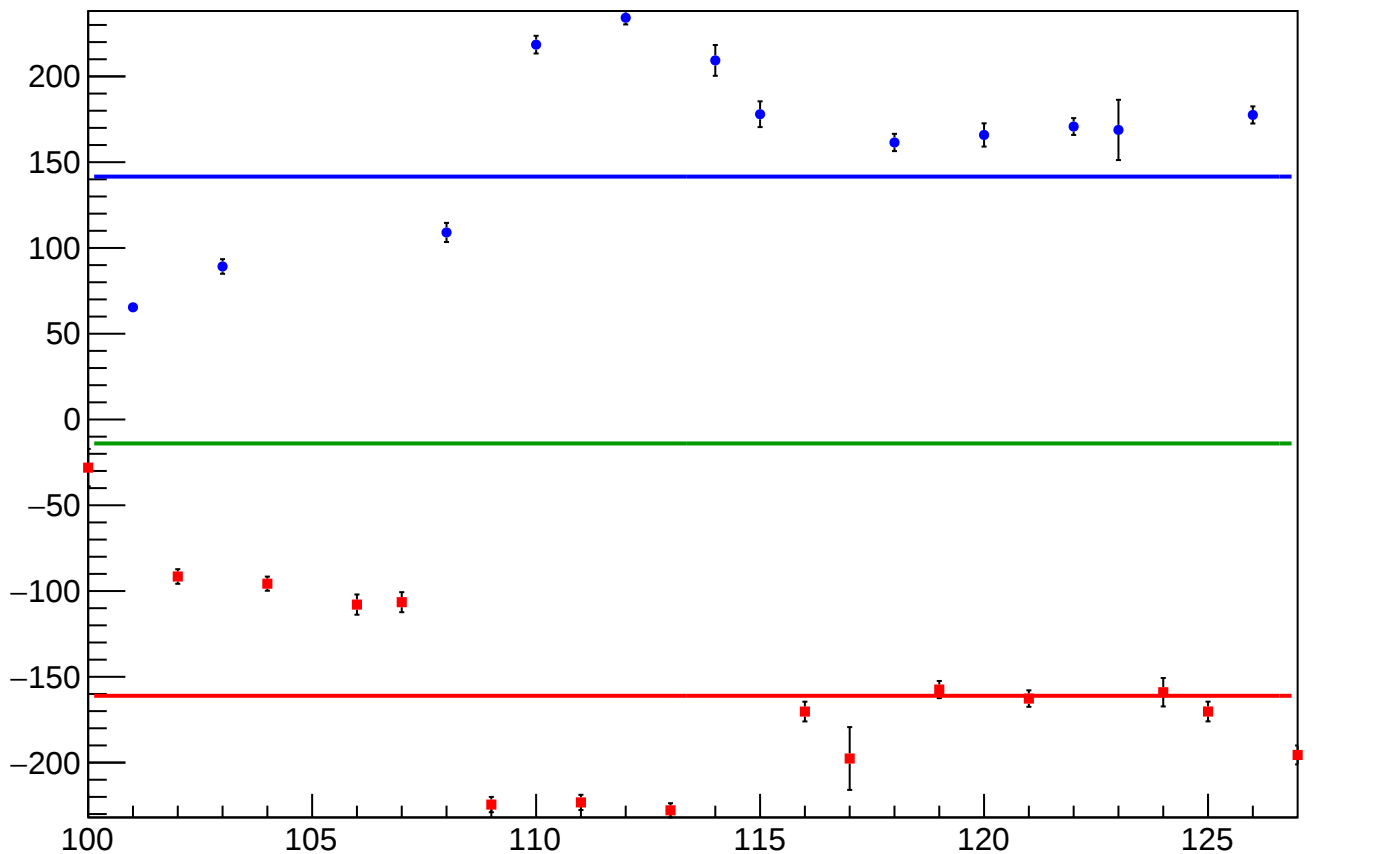
reg_asym_usr_diff_bpm4eX_slope vs Slug, Sign Corrected
