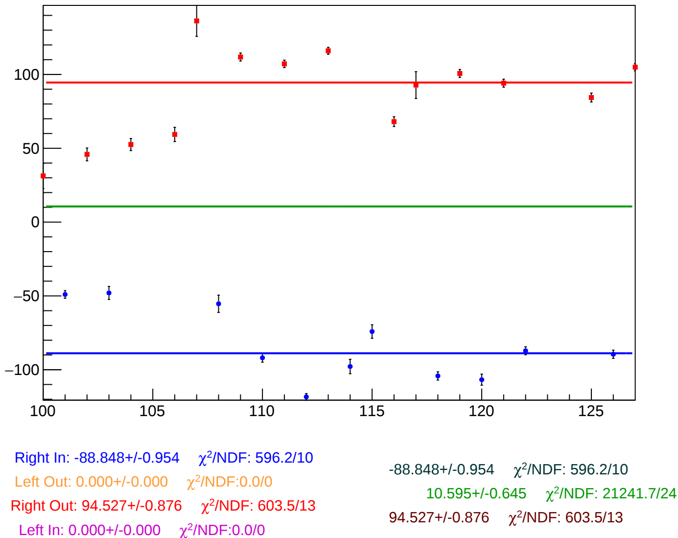
reg_asym_usl_diff_bpm4aX_slope vs Slug, Sign Corrected
