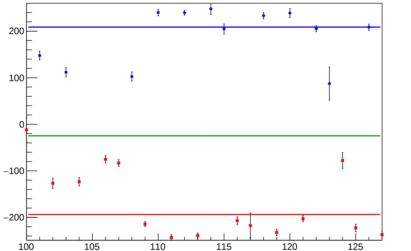
reg_asym_atl_dd_atr_dd_avg_diff_bpm4aX_slope vs Slug, Sign Corrected
