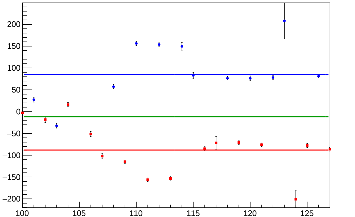
reg_asym_atl_dd_atr_dd_dd_diff_bpm4eX_slope vs Slug, Sign Corrected
