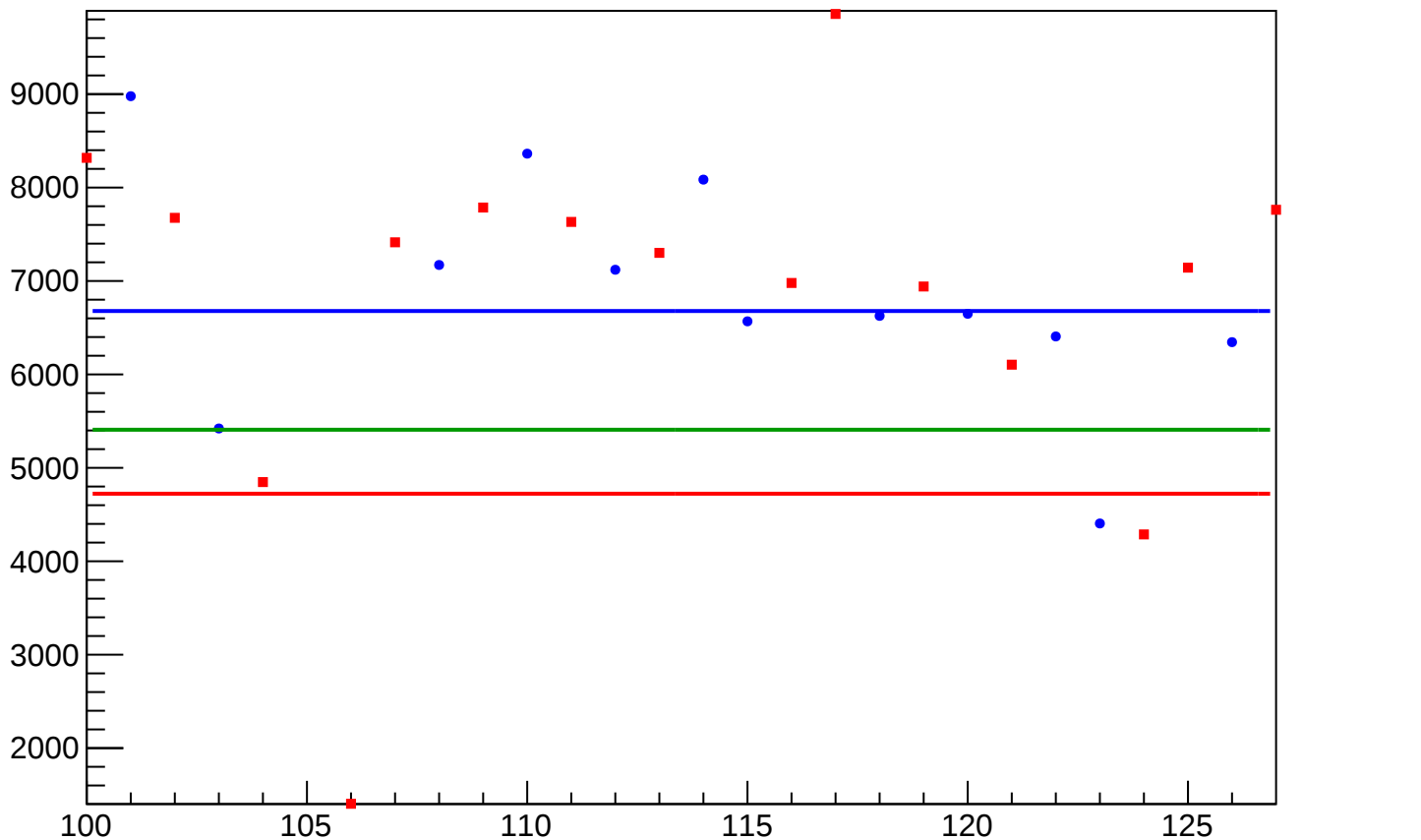
asym_at2_avg_correction_rms vs Slug, Sign Corrected
