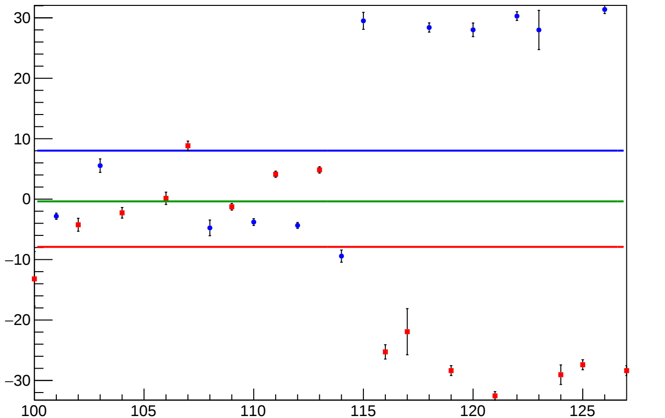
reg_asym_sam_15_37_dd_diff_bpm4eY_slope vs Slug, Sign Corrected
