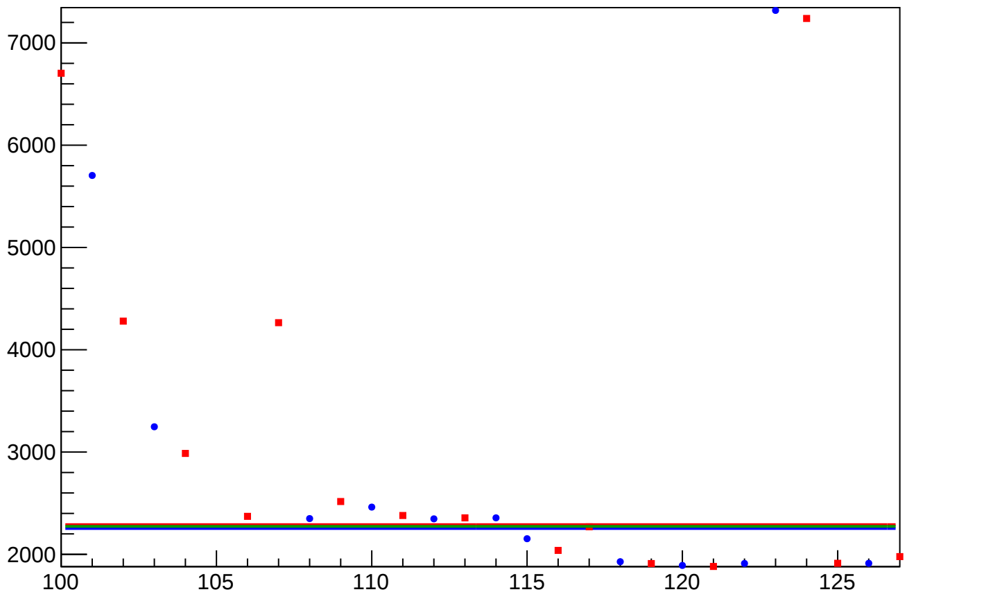
asym_at1_avg_rms vs Slug, Sign Corrected
