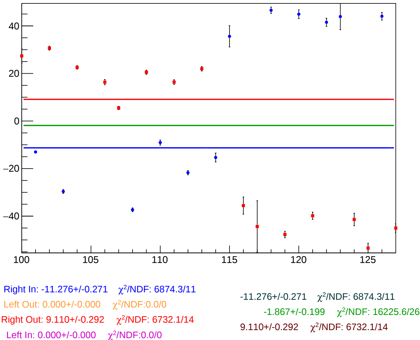
reg_asym_sam6_diff_bpm4eY_slope vs Slug, Sign Corrected
