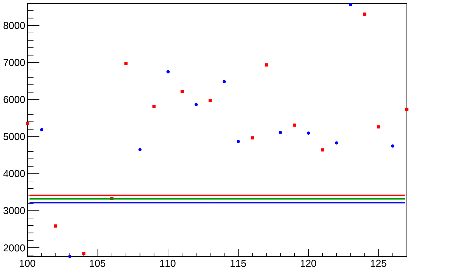
asym_atl1r2_avg_rms vs Slug, Sign Corrected
