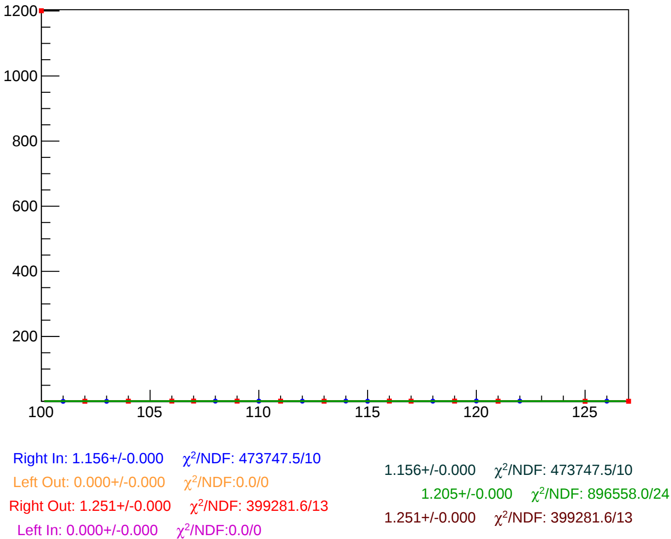
asym_ds_dd_correction_rms vs Slug, Sign Corrected
