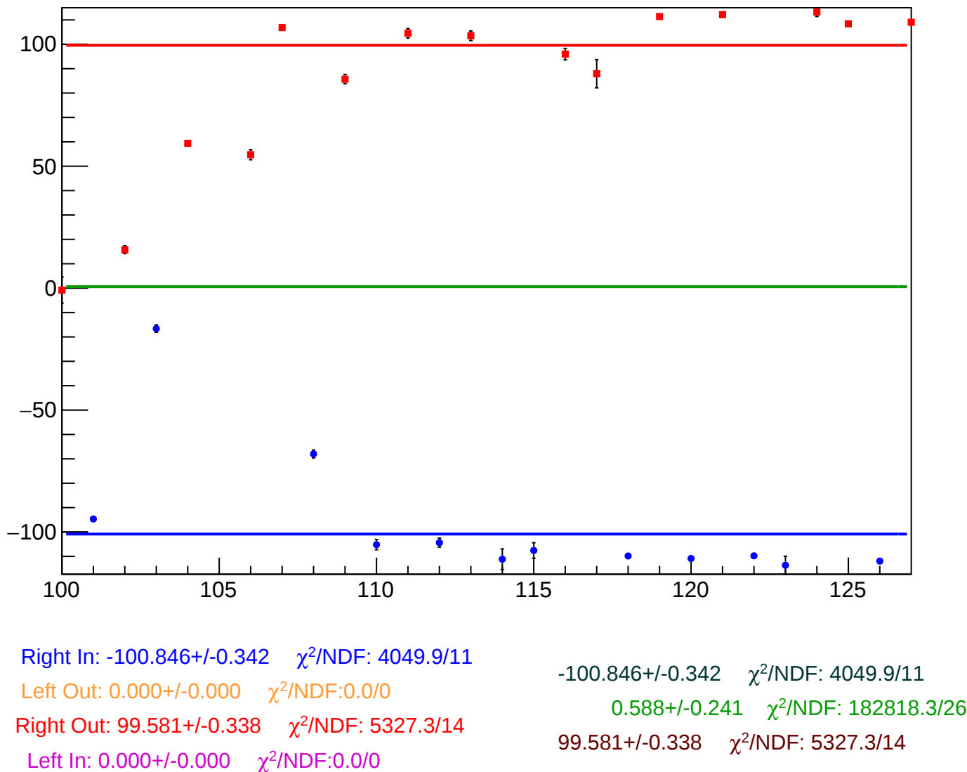
reg_asym_sam_26_48_dd_diff_bpm4eY_slope vs Slug, Sign Corrected
