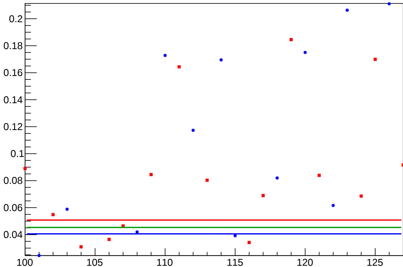
yield_bpm1X_rms vs Slug, Sign Corrected
