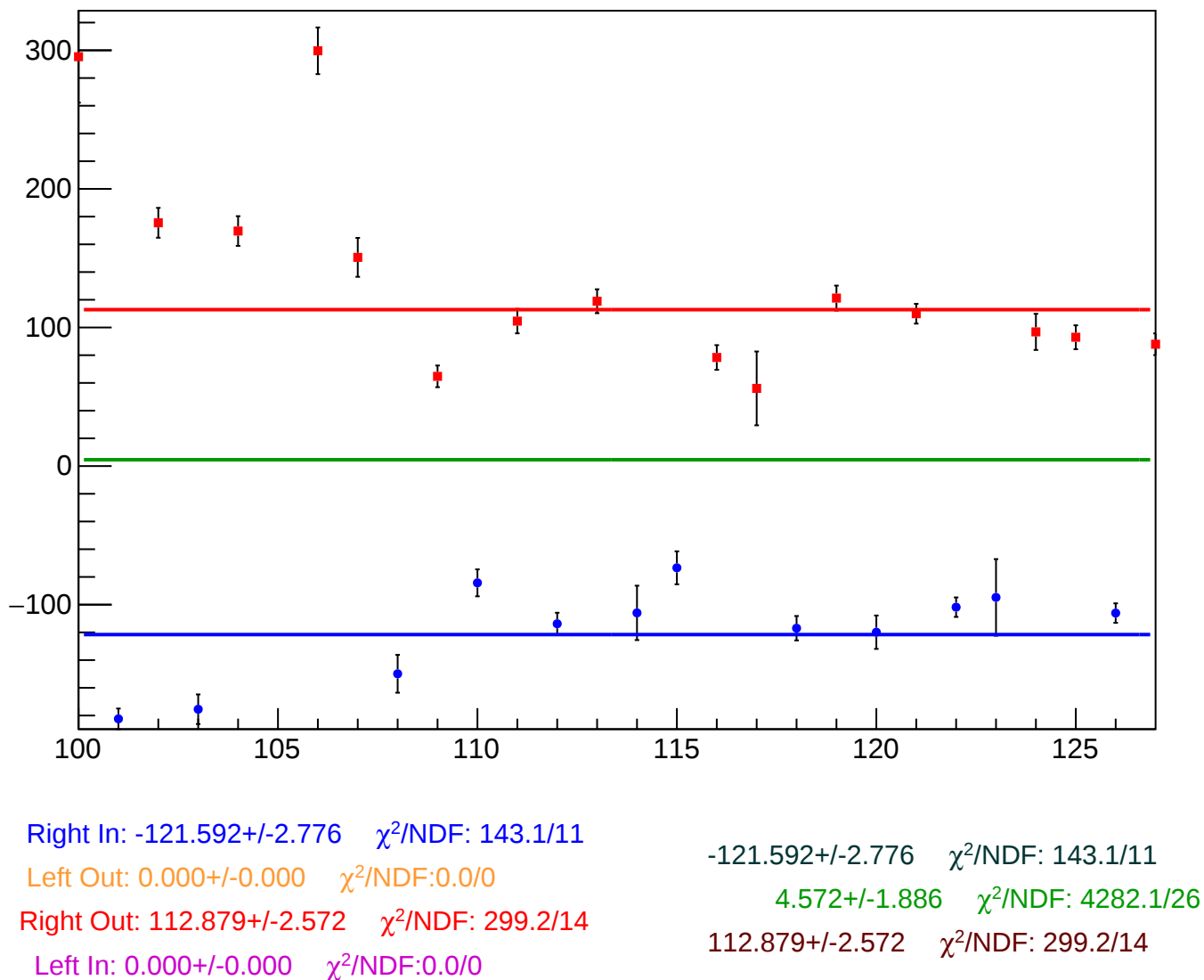
reg_asym_sam2_diff_bpm4aX_slope vs Slug, Sign Corrected
