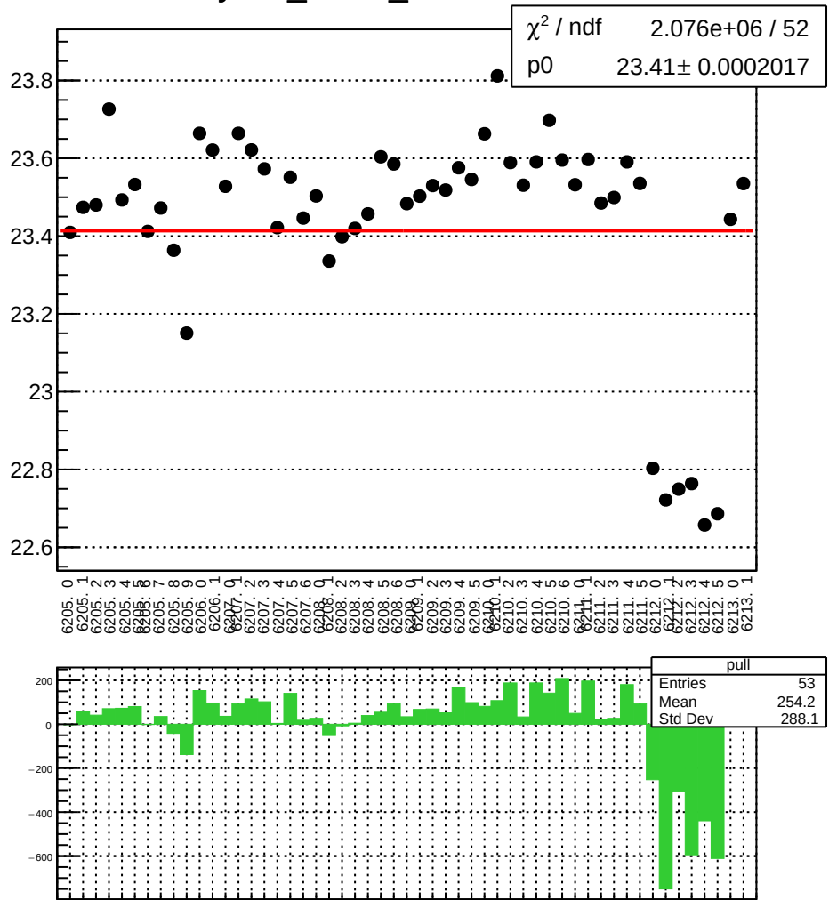
yield_sam2_mean vs run
