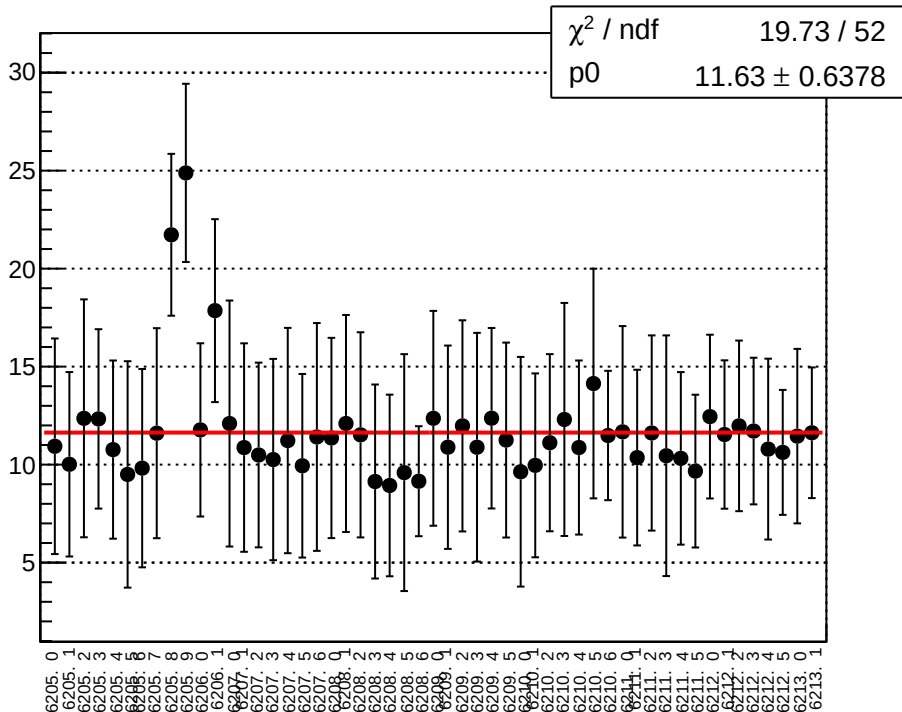
reg asym sam7 diff bpm4aY slope vs run
