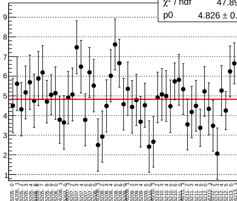
reg_asym_at1_dd_diff_bpm12X_slope vs run
