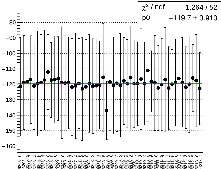
reg asym sam 26 dd diff bpm4eY slope vs run
