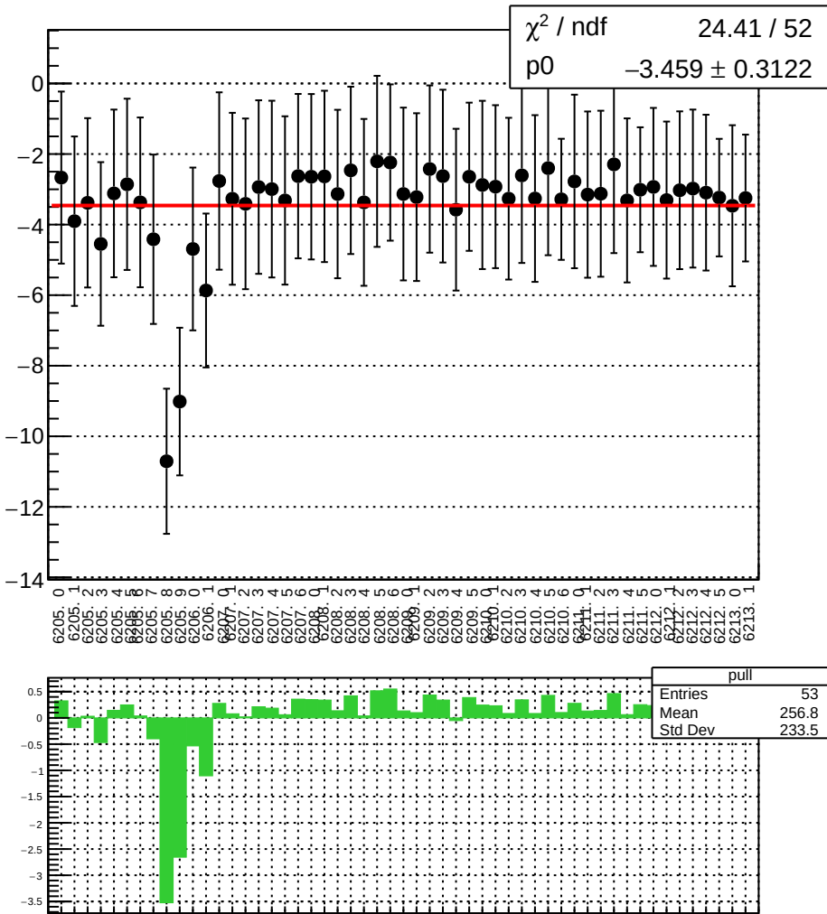
reg asym sam4 diff bpm12X slope vs run
