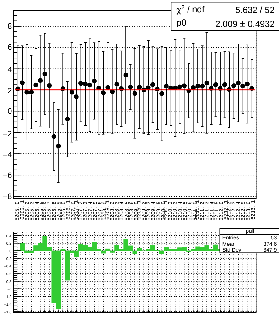
reg_asym_sam_1357_2468_dd_diff_bpm4aY_slope vs run
