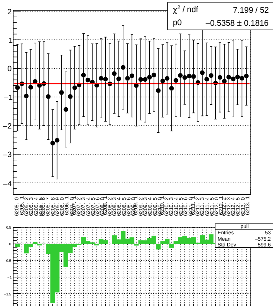
reg_asym_sam3_diff_bpm12X_slope vs run
