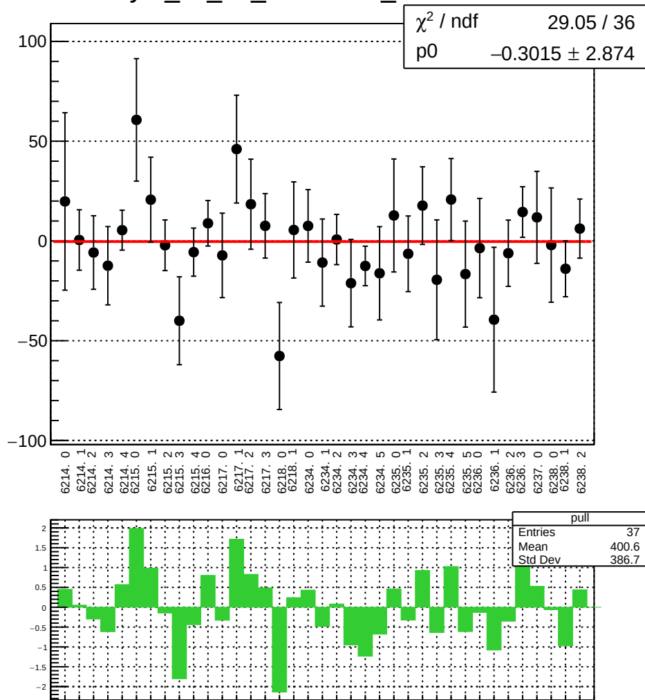
asym_ds_dd_correction_mean vs run
