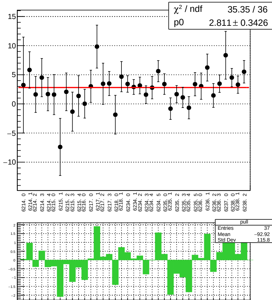
reg_asym_bcm_an_us_diff_bpm4aX_slope vs run
