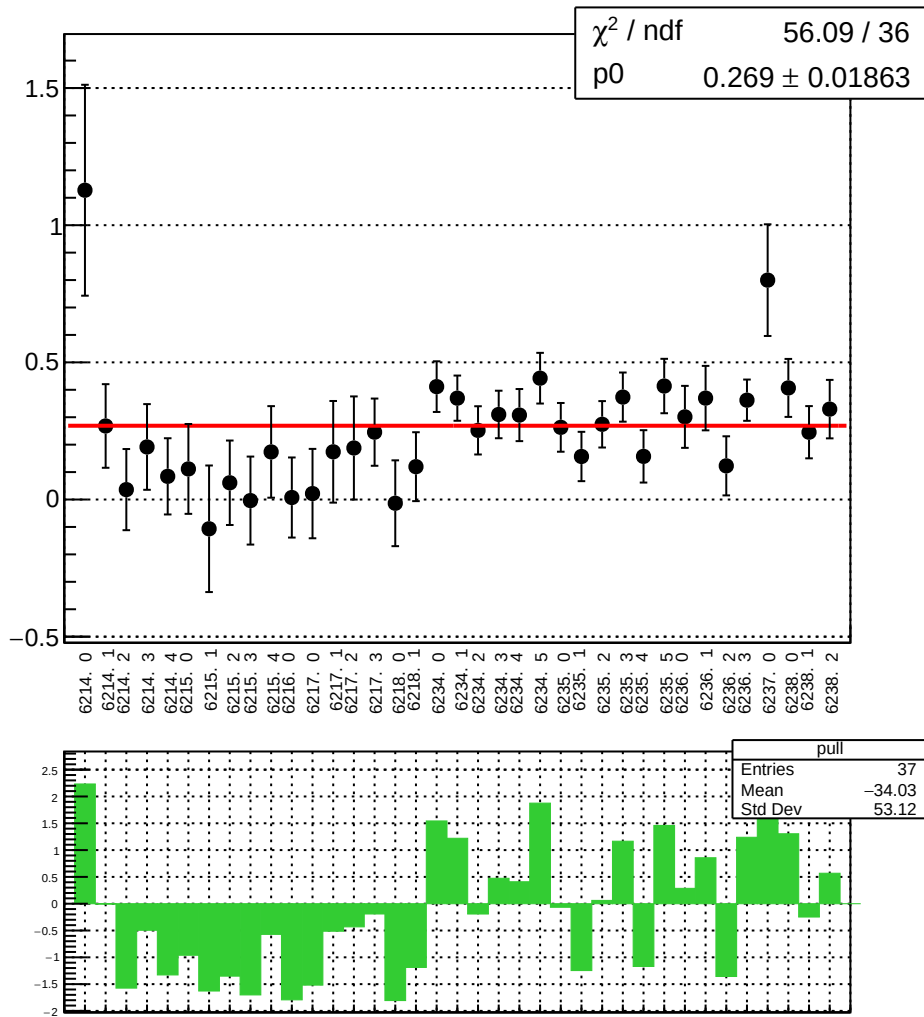
reg_asym_bcm_an_ds_diff_bpm12X_slope vs run
