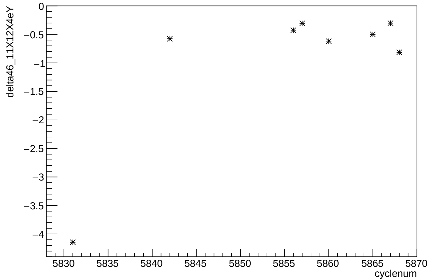
delta46_11X12X4eY:cyclenum
