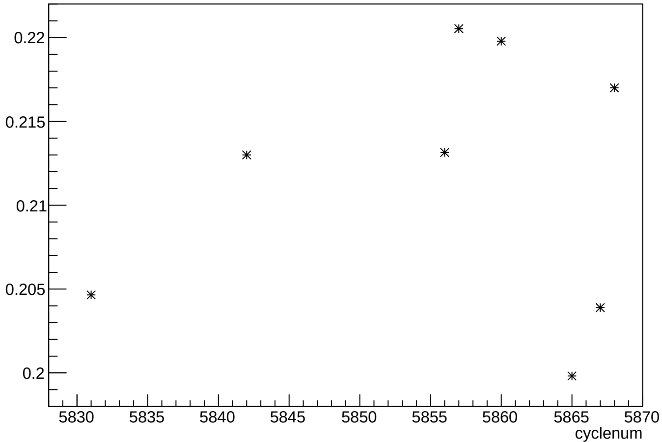
alpha13_4eX4aX:cyclenum
