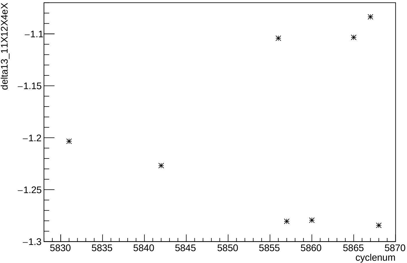
delta13_11X12X4eX:cyclenum
