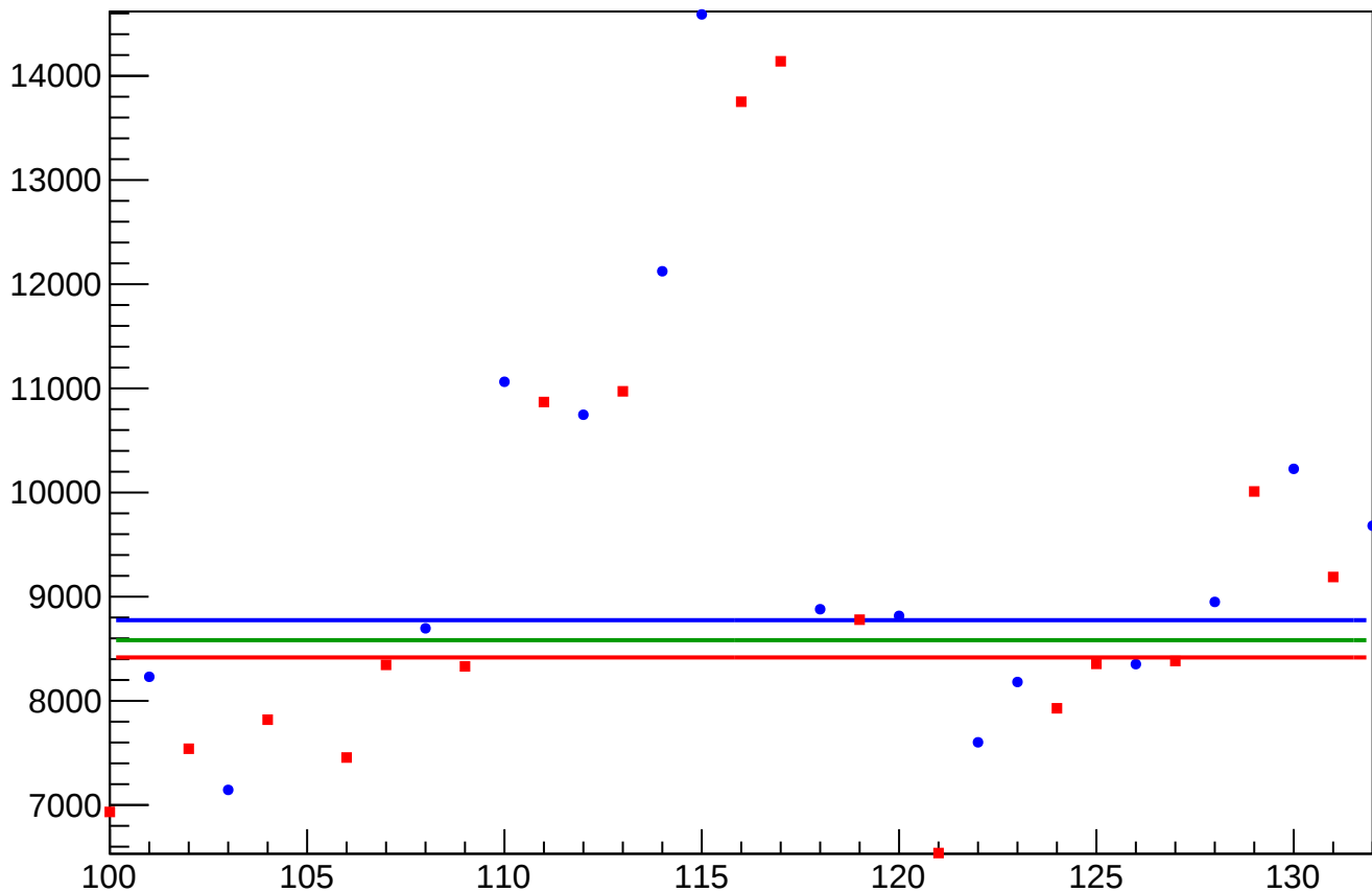
diff_bpm4aY_rms vs Slug, Sign Corrected
