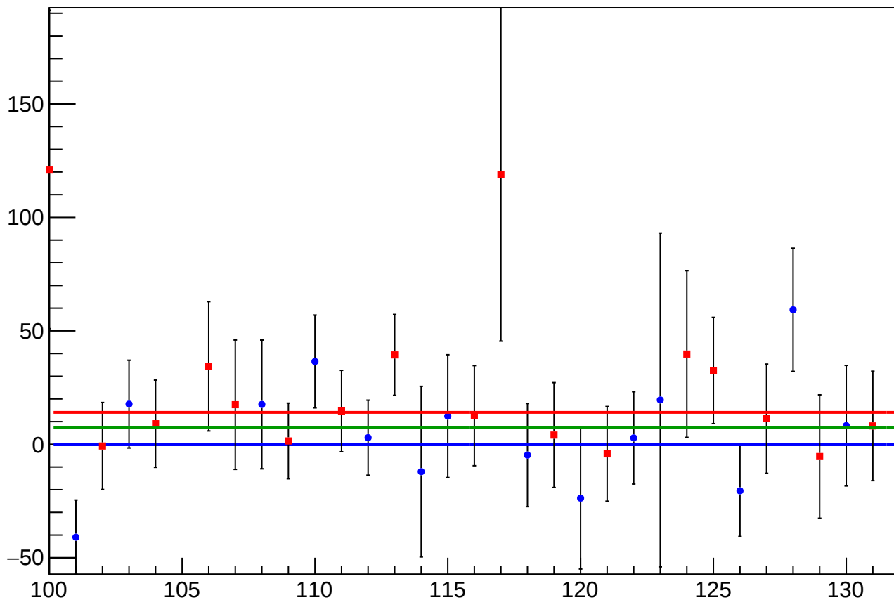
diff_bpm4ecX_mean vs Slug, Sign Corrected
