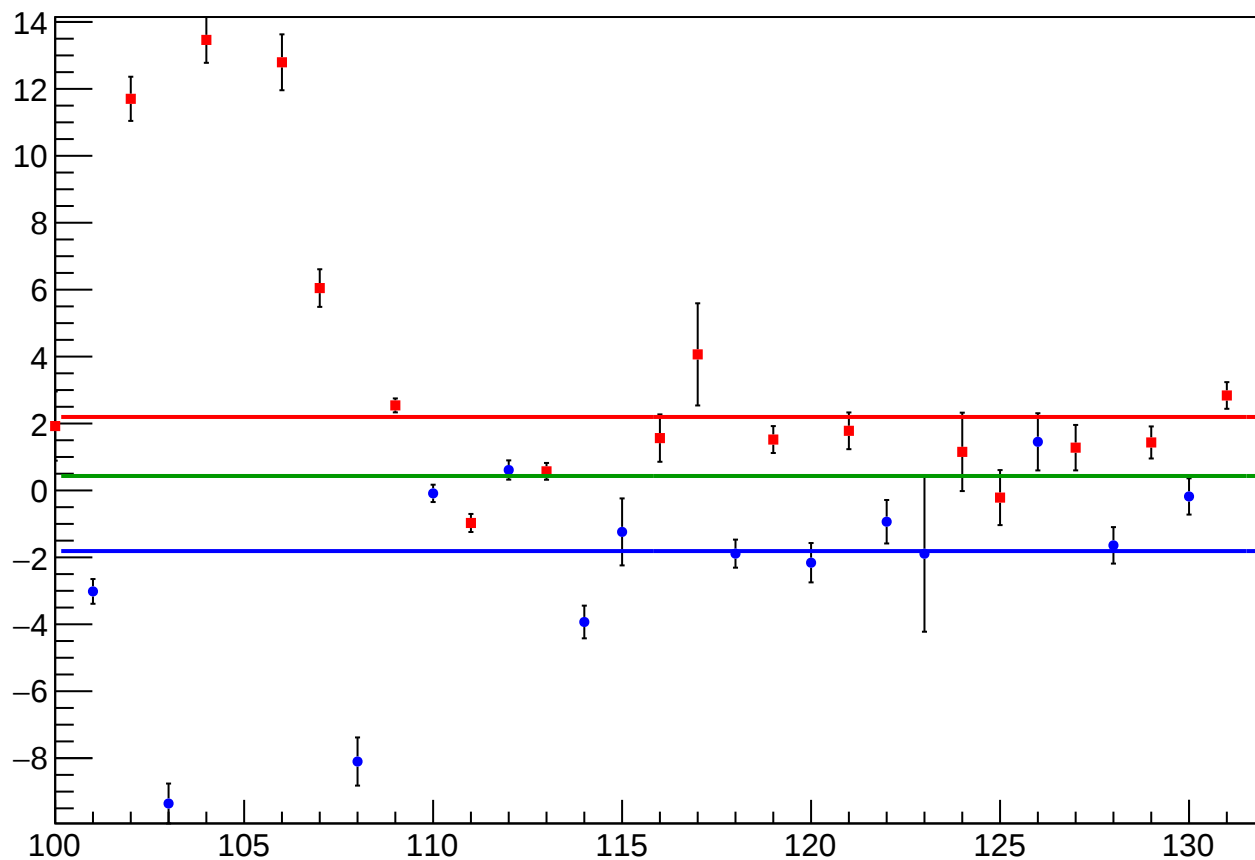
reg_asym_bcm_an_ds_diff_bpm4eX_slope vs Slug, Sign Corrected
