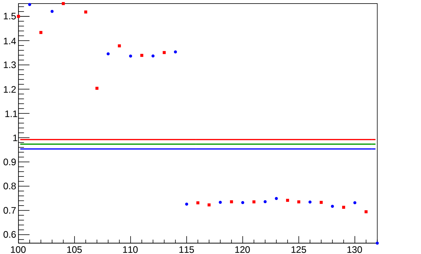
yield_bpm4acY_mean vs Slug, Sign Corrected
