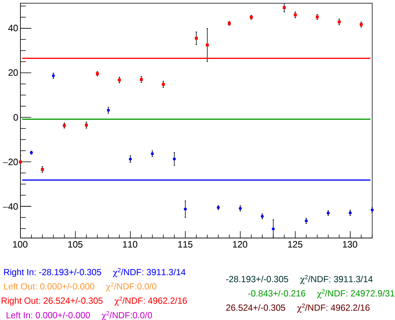
reg_asym_sam_15_dd_diff_bpm4eY_slope vs Slug, Sign Corrected
