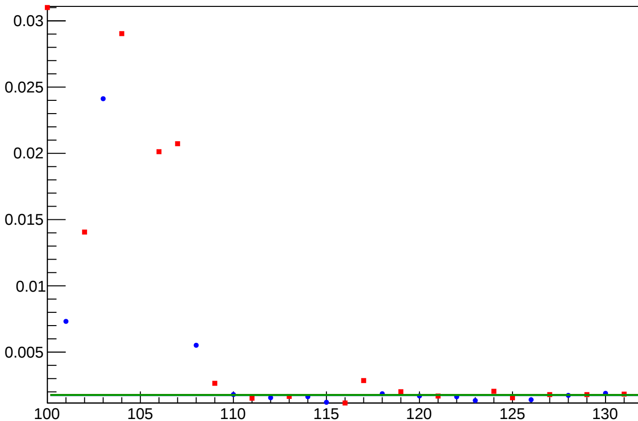
yield_cav4cX_rms vs Slug, Sign Corrected
