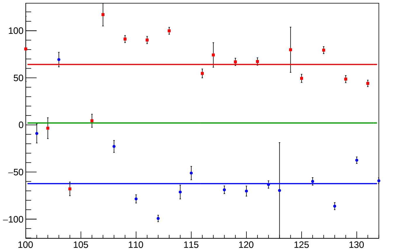
reg_asym_at1_avg_diff_bpm4aX_slope vs Slug, Sign Corrected
