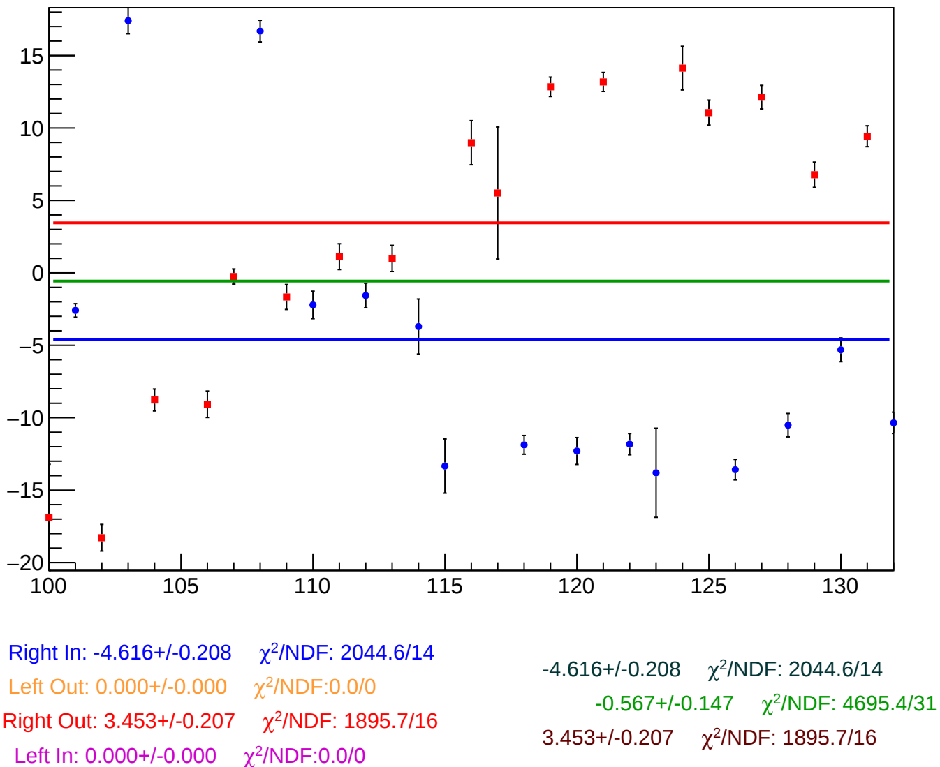
reg_asym_sam_13_57_dd_diff_bpm4eY_slope vs Slug, Sign Corrected
