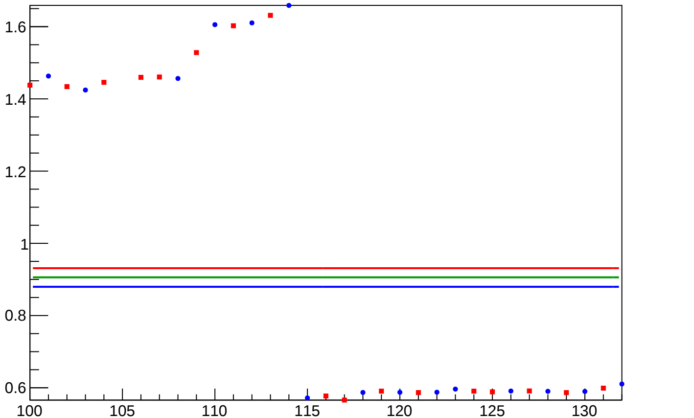
yield_bpm4aY_mean vs Slug, Sign Corrected
