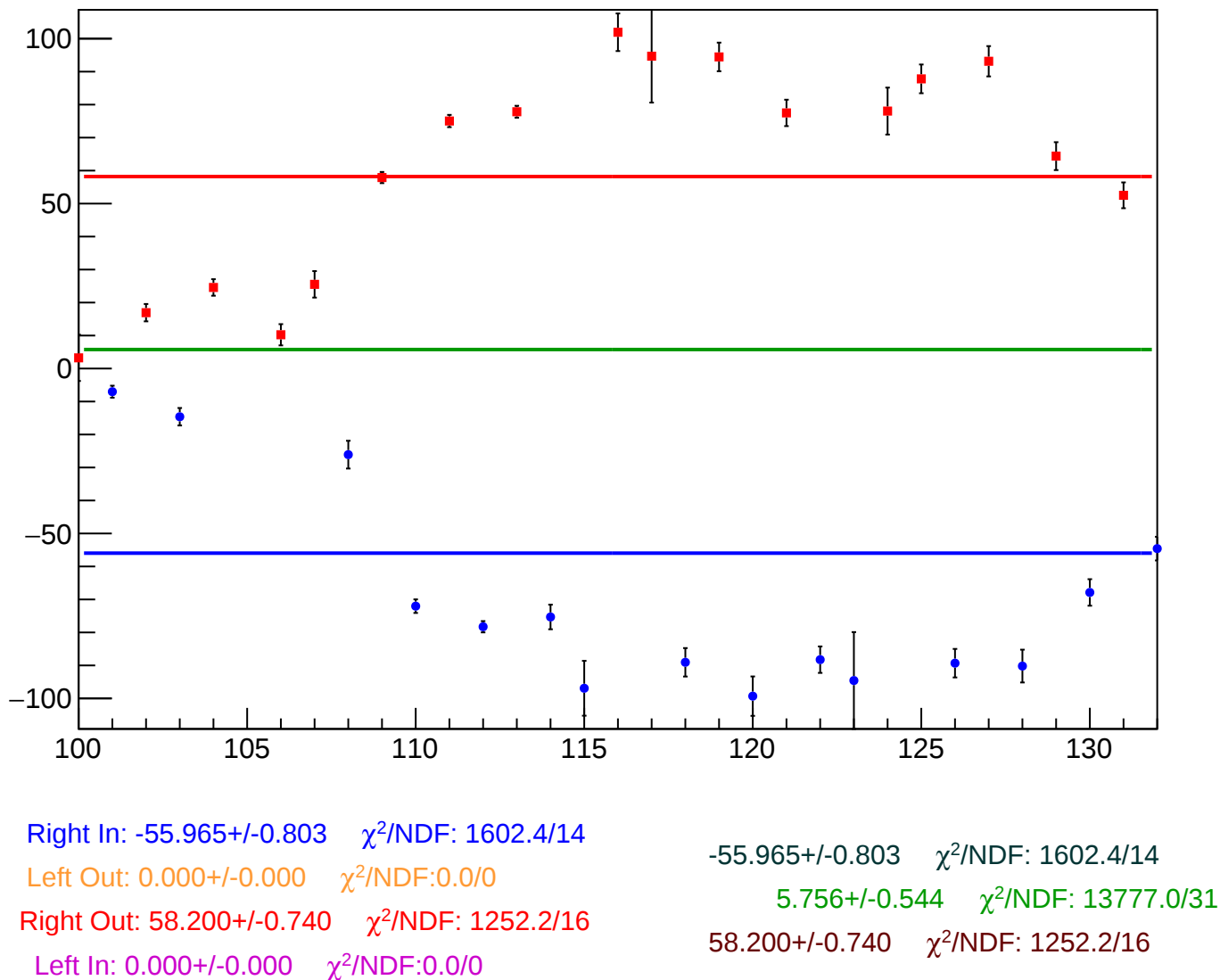
reg_asym_sam_48_avg_diff_bpm4eX_slope vs Slug, Sign Corrected
