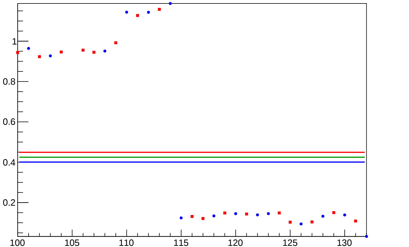
yield_bpm4ecY_mean vs Slug, Sign Corrected
