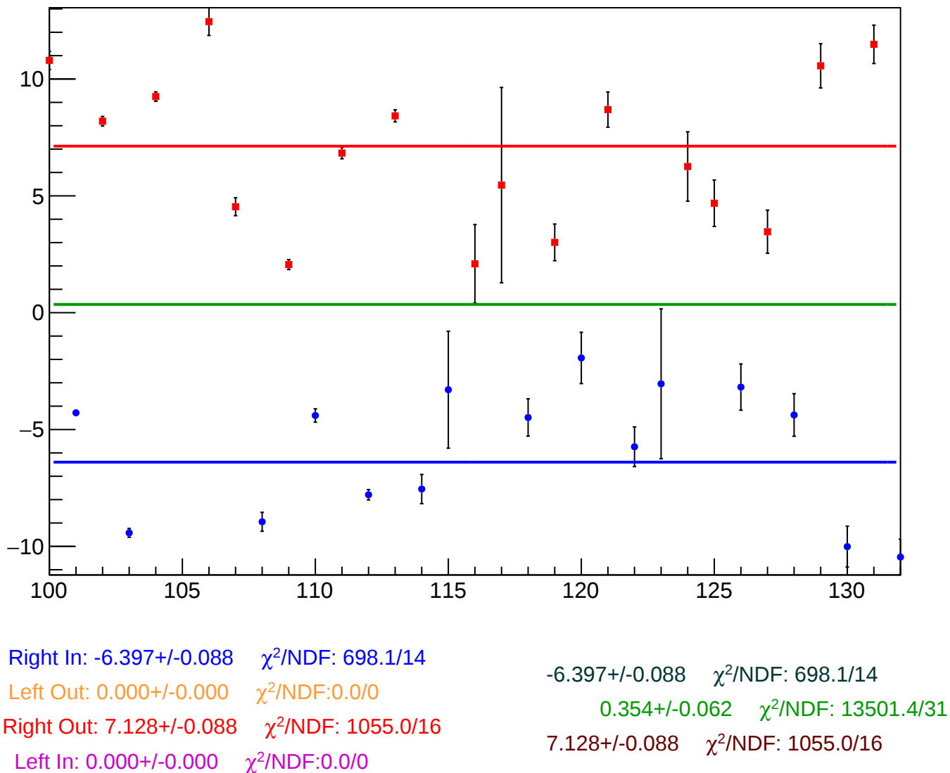
reg_asym_sam_15_avg_diff_bpm4aX_slope vs Slug, Sign Corrected
