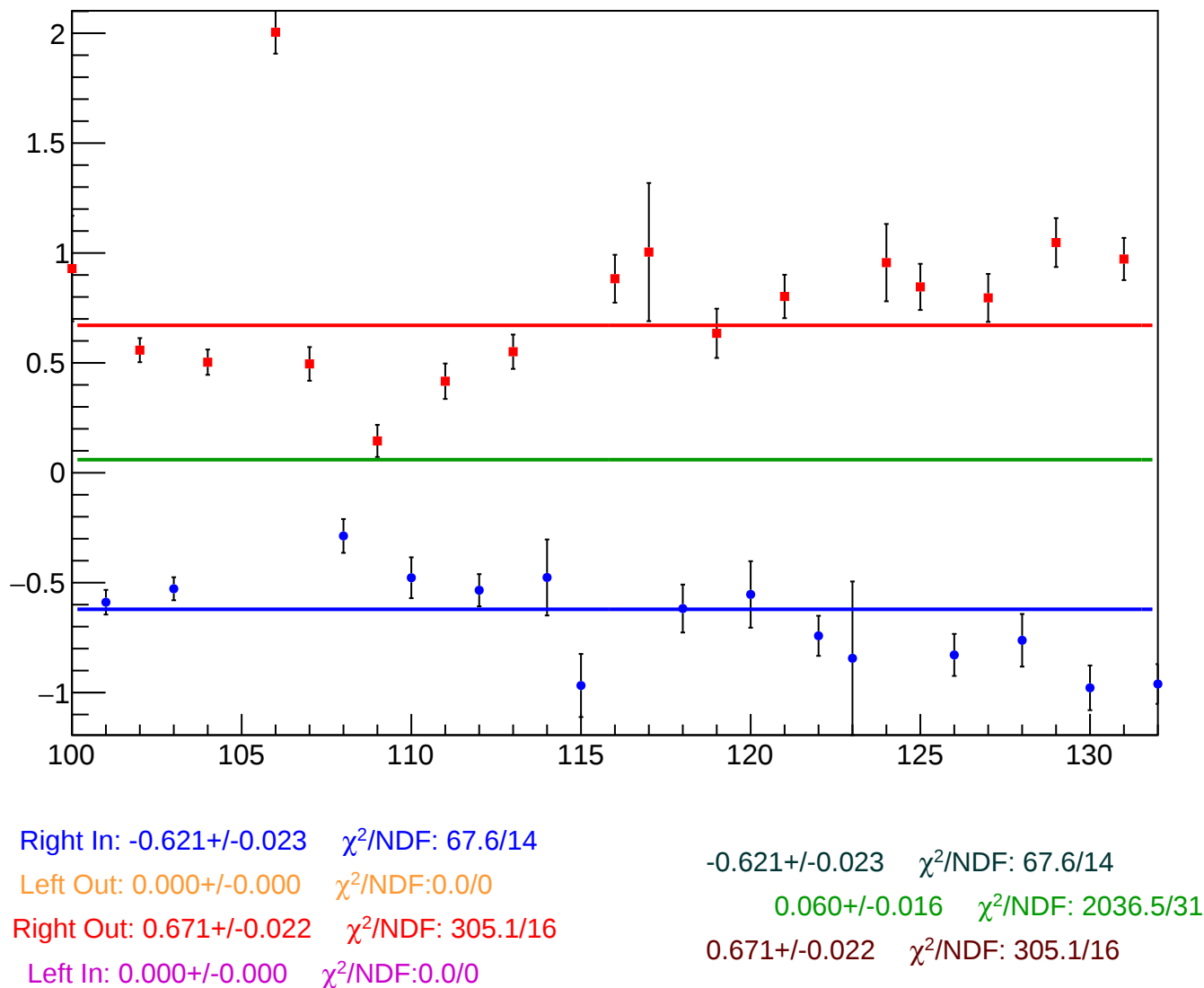
reg_asym_sam_12345678_avg_diff_bpm12X_slope vs Slug, Sign Corrected
