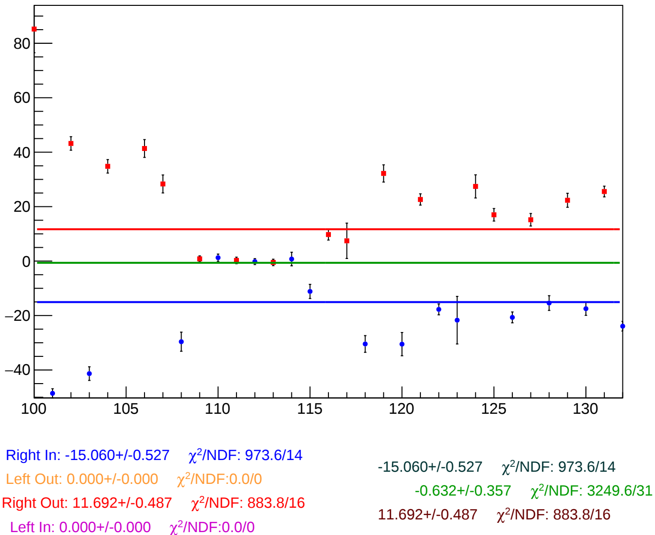
reg_asym_sam_37_avg_diff_bpm4aX_slope vs Slug, Sign Corrected
