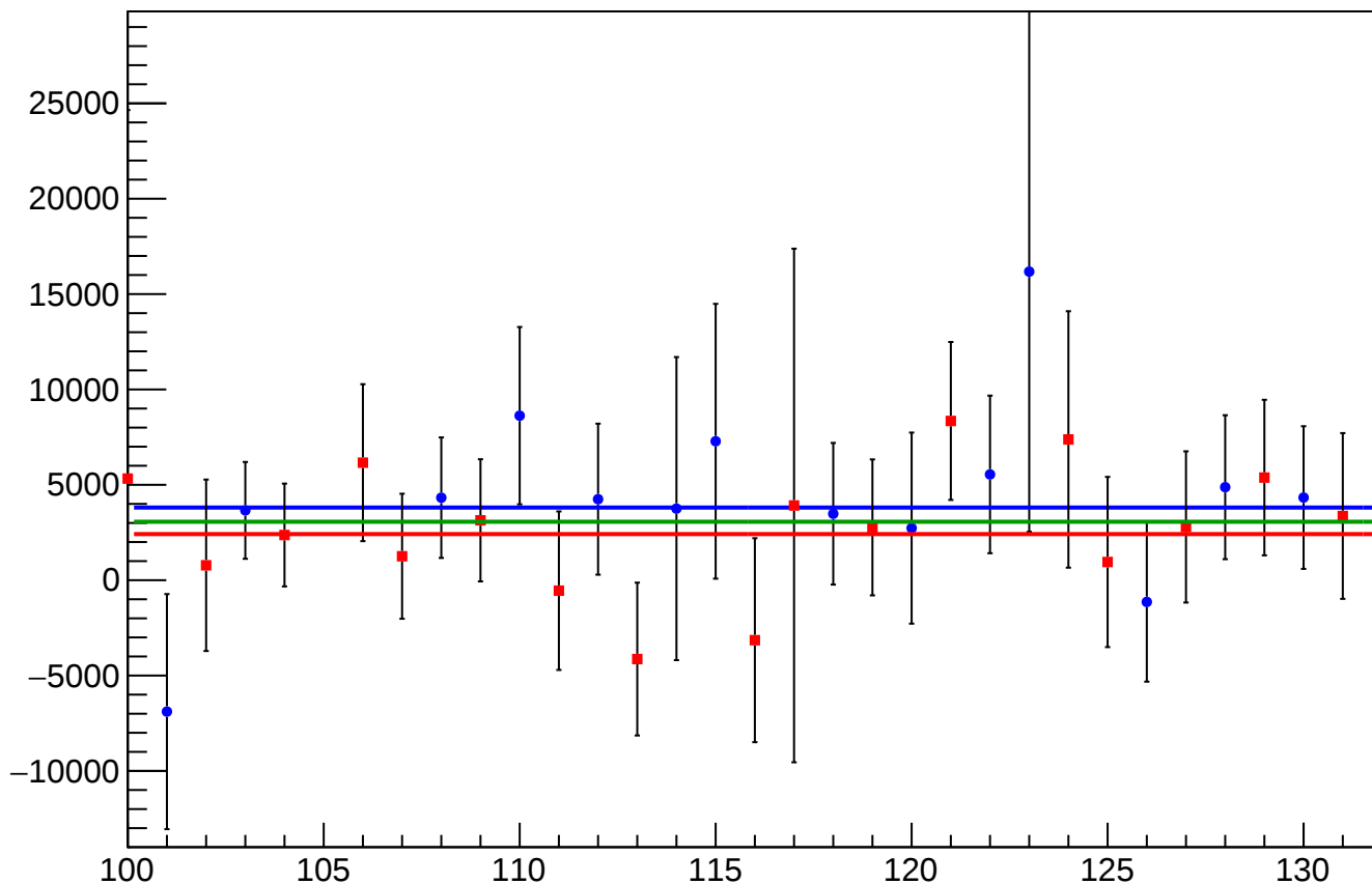
reg_asym_atr2_mean vs Slug, Sign Corrected
