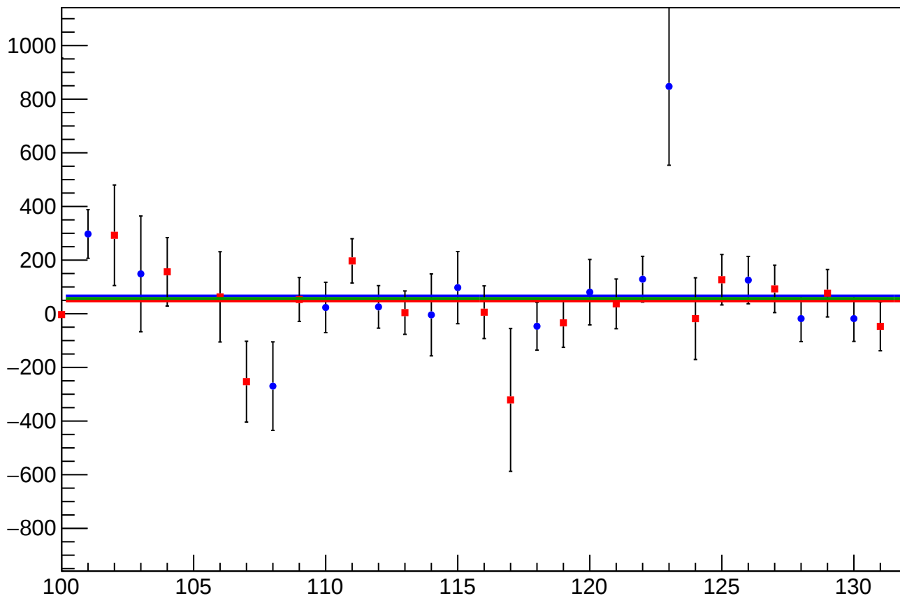
reg_asym_sam_37_dd_mean vs Slug, Sign Corrected
