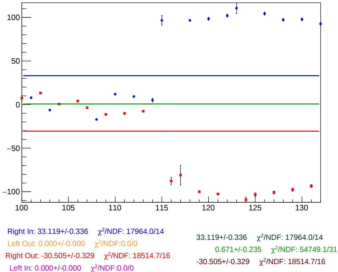
reg_asym_sam5_diff_bpm4eY_slope vs Slug, Sign Corrected
