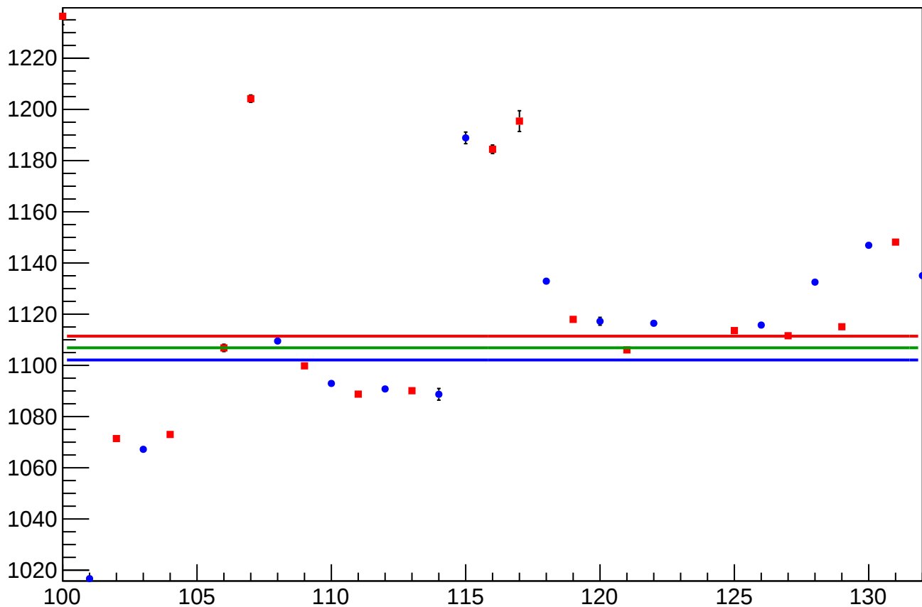
reg_asym_usl_rms vs Slug, Sign Corrected
