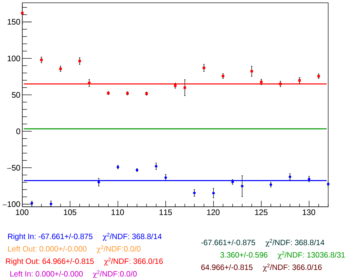
reg_asym_sam3_diff_bpm4aX_slope vs Slug, Sign Corrected
