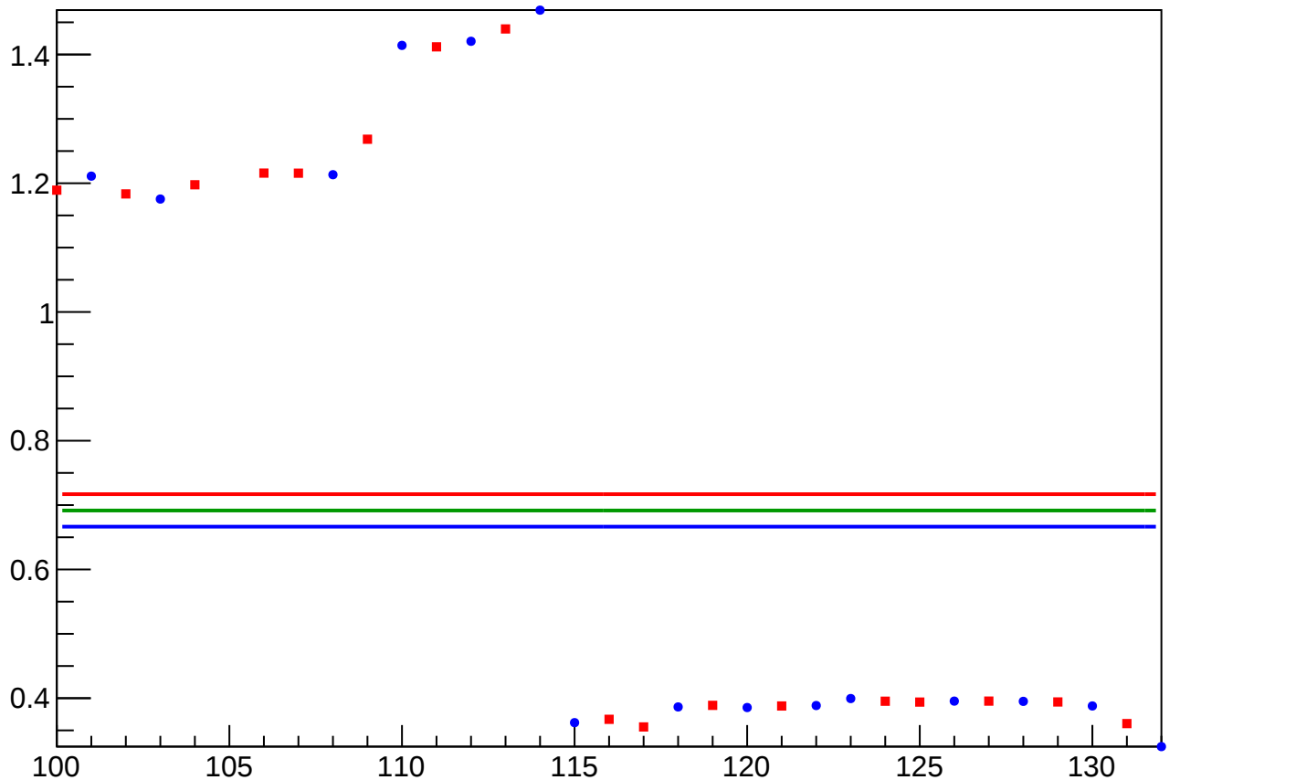
yield_bpm4eY_mean vs Slug, Sign Corrected
