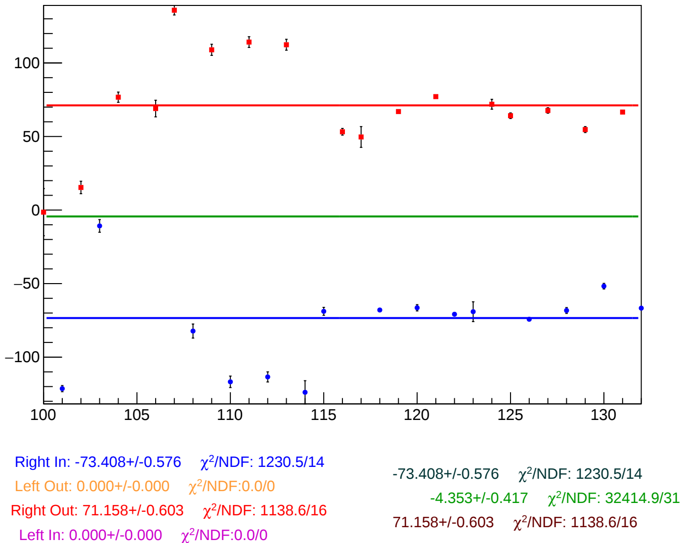
reg_asym_sam_26_avg_diff_bpm4eY_slope vs Slug, Sign Corrected
