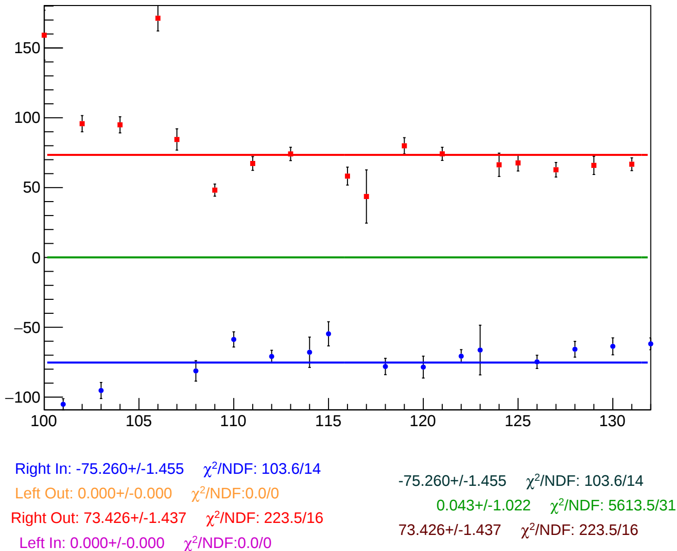
reg_asym_sam_26_dd_diff_bpm4aX_slope vs Slug, Sign Corrected
