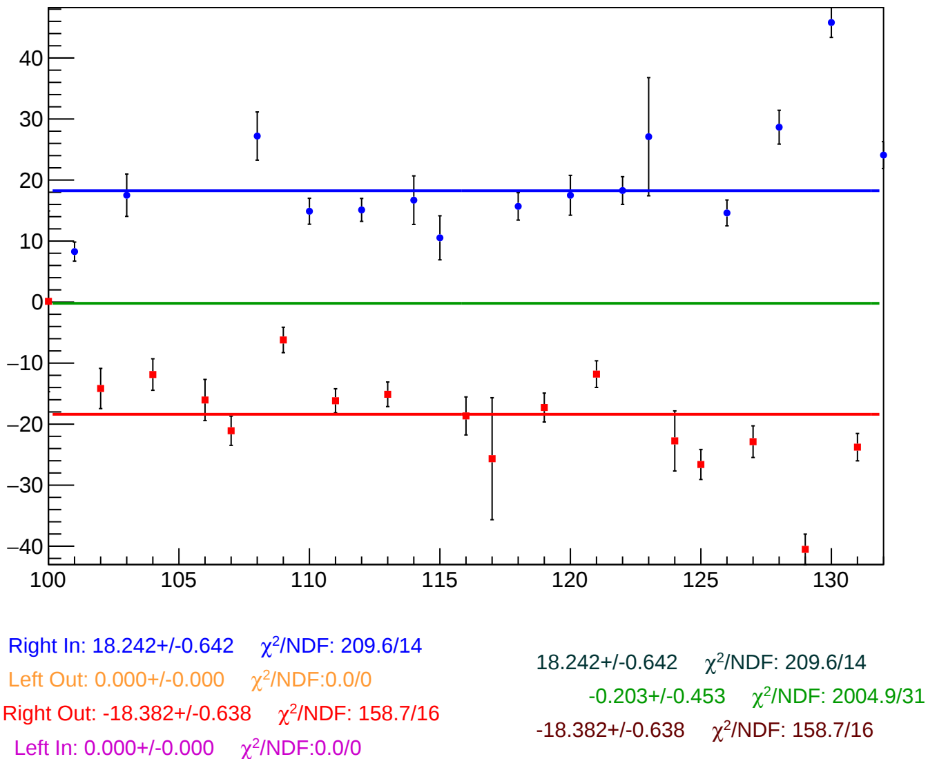
reg_asym_sam3_diff_bpm4eY_slope vs Slug, Sign Corrected
