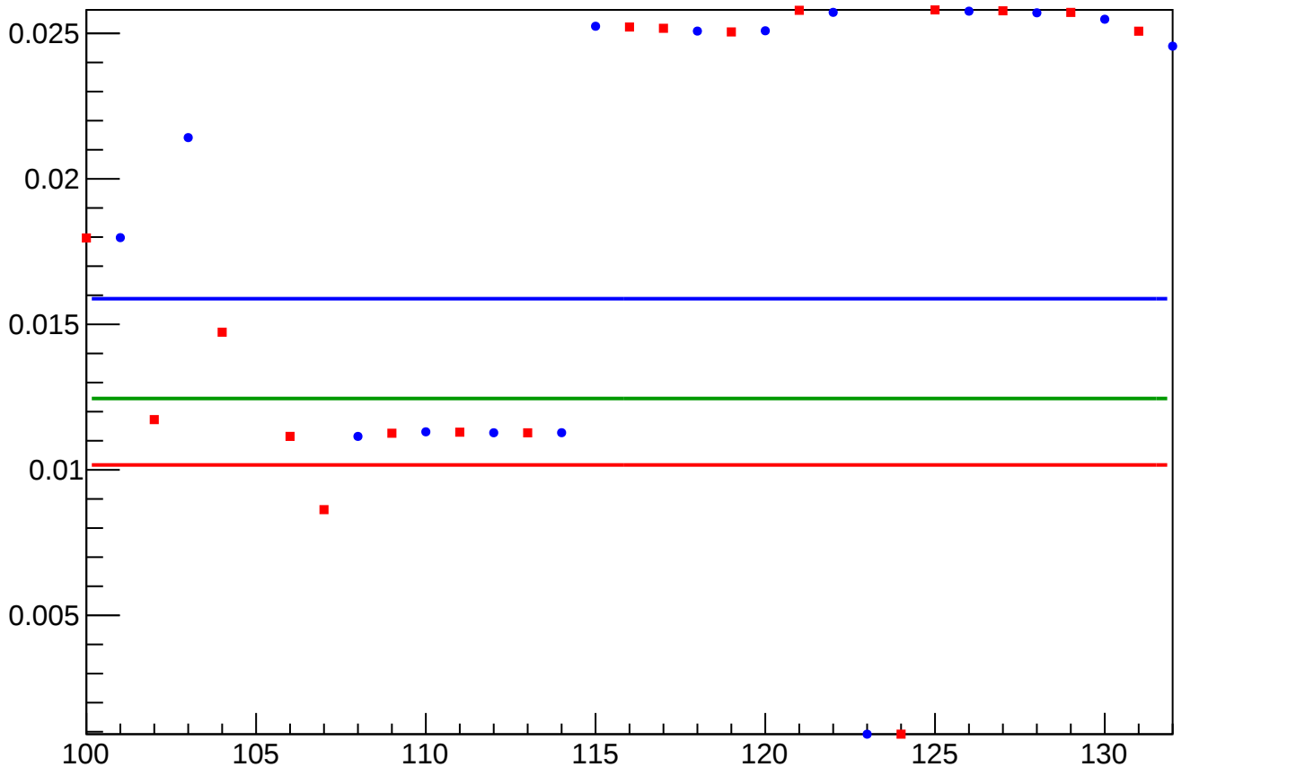
yield_atl1_mean vs Slug, Sign Corrected
