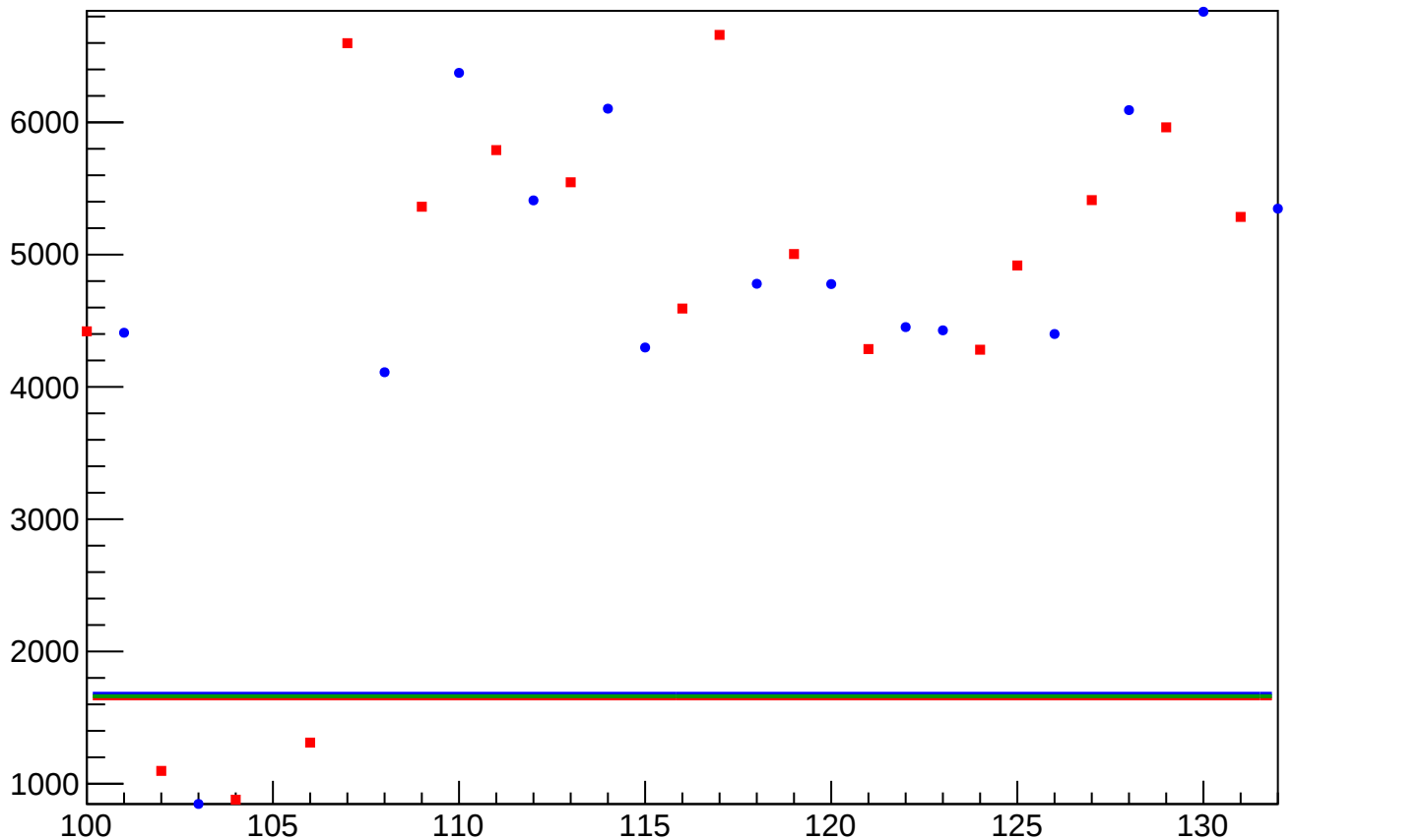
asym_atl1r2_avg_correction_rms vs Slug, Sign Corrected
