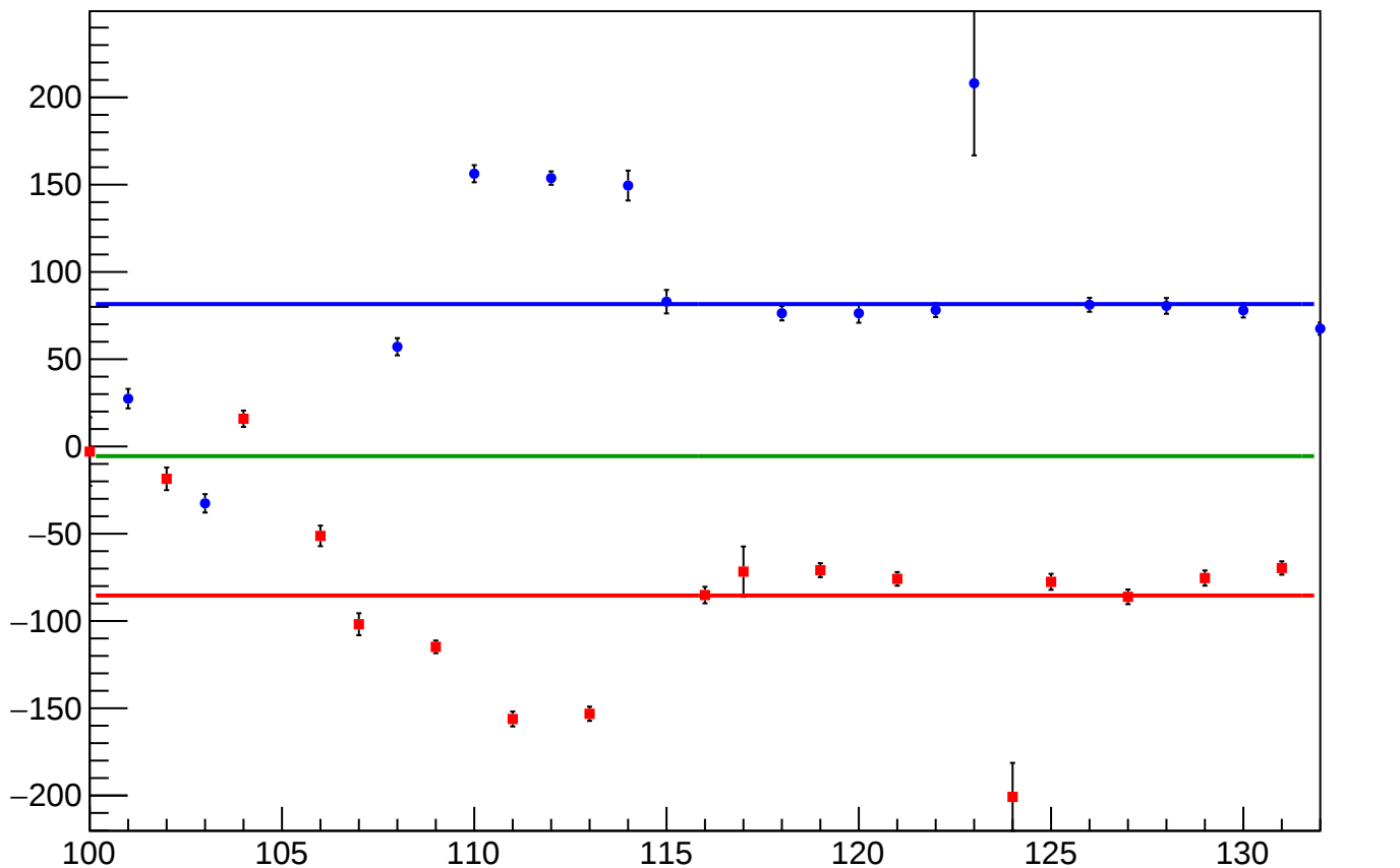
reg_asym_atl_dd_atr_dd_diff_bpm4eX_slope vs Slug, Sign Corrected
