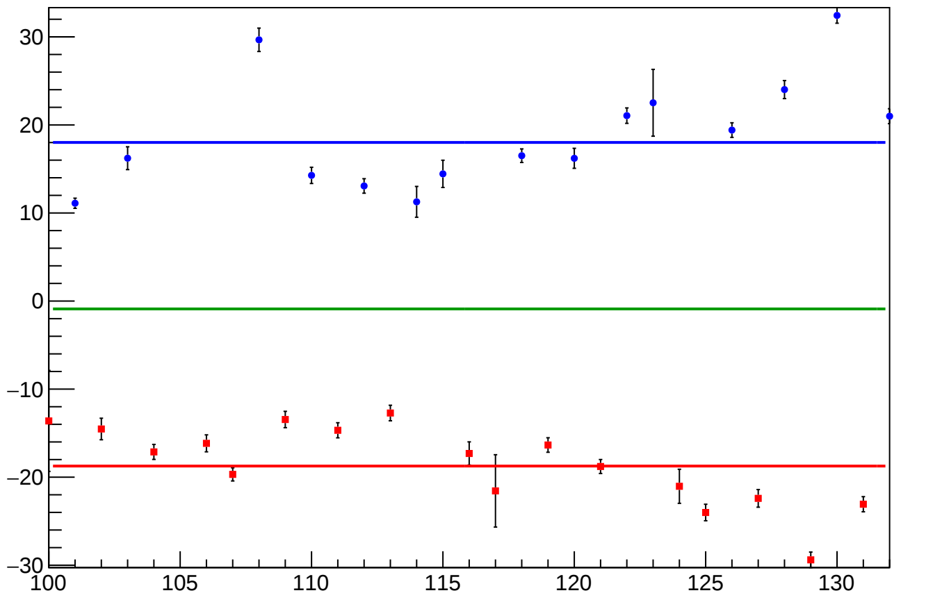
reg_asym_sam_37_dd_diff_bpm4eY_slope vs Slug, Sign Corrected
