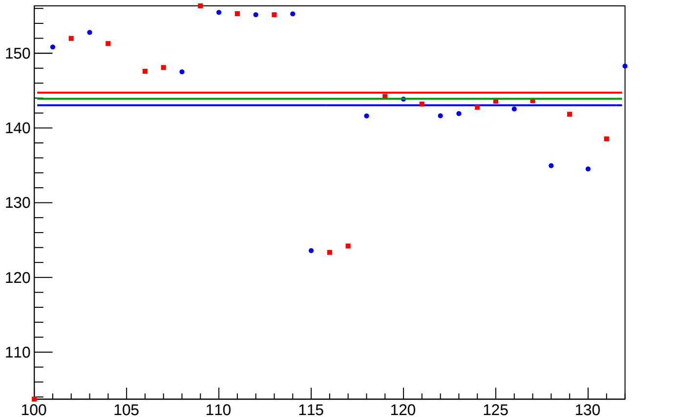
yield_bcm_dg_ds_mean vs Slug, Sign Corrected
