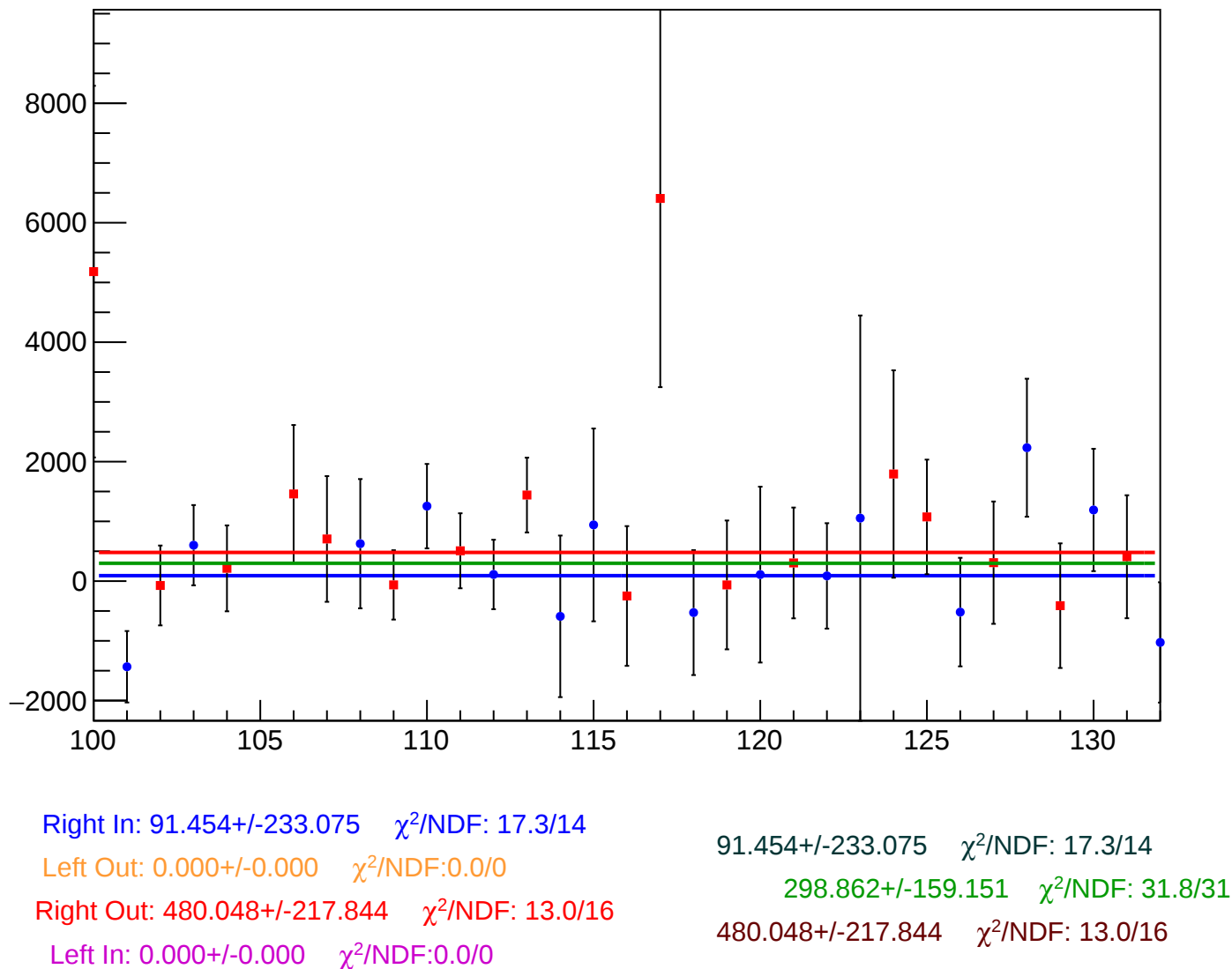
asym_sam_1357_avg_correction_mean vs Slug, Sign Corrected
