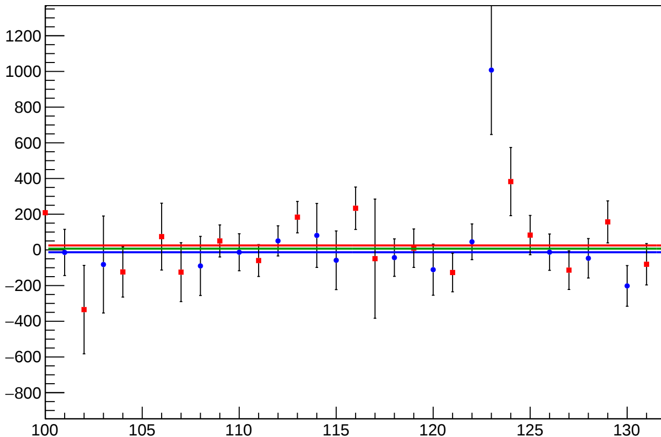
reg_asym_sam_37_avg_mean vs Slug, Sign Corrected
