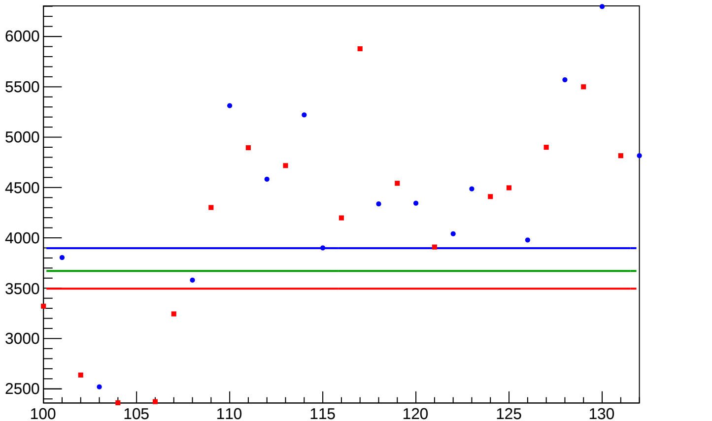
asym_atr_dd_correction_rms vs Slug, Sign Corrected
