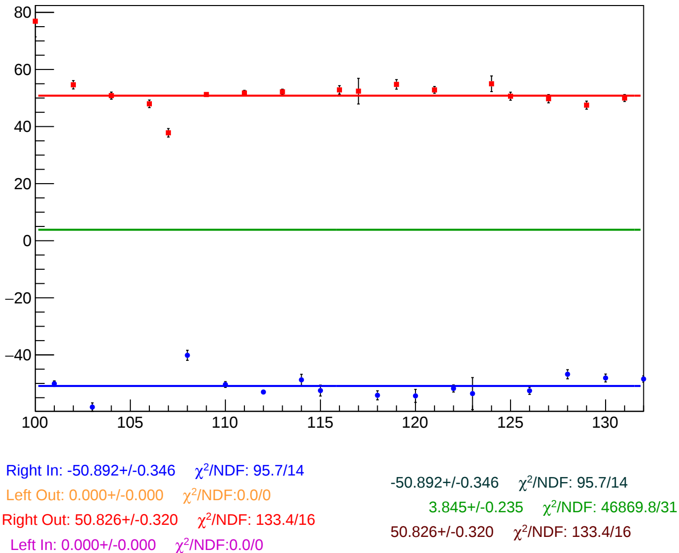
reg_asym_sam_37_dd_diff_bpm4aX_slope vs Slug, Sign Corrected
