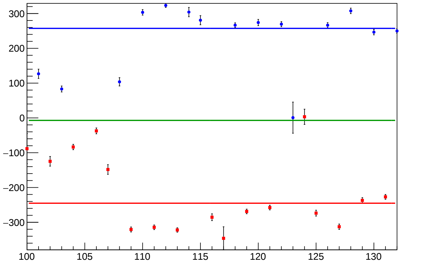
reg_asym_atr1l2_avg_diff_bpm4eX_slope vs Slug, Sign Corrected
