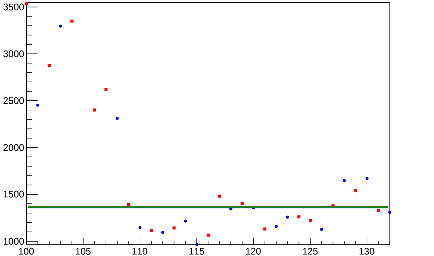
diff_cav4cX_rms vs Slug, Sign Corrected
