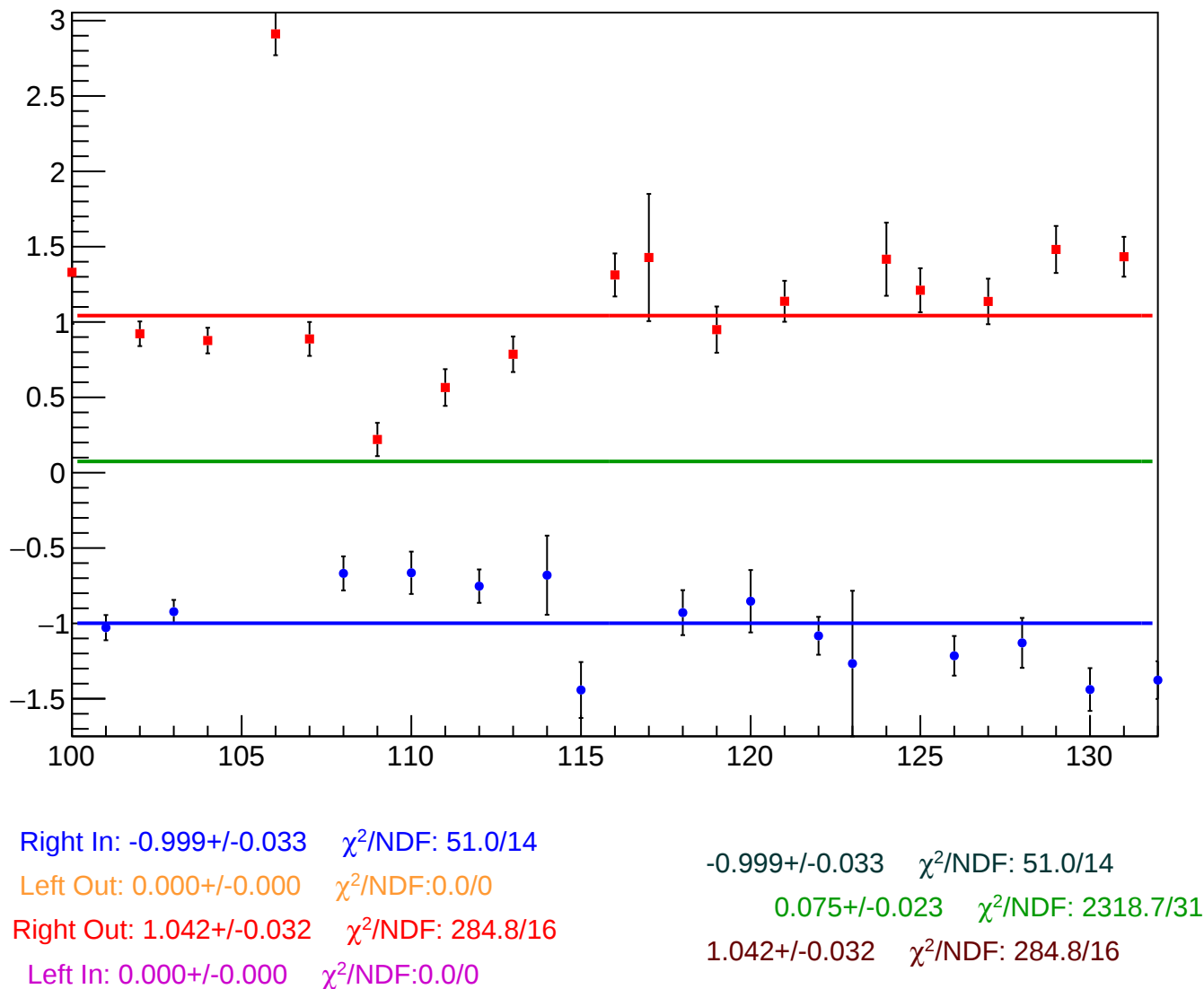
reg_asym_sam_2468_avg_diff_bpm12X_slope vs Slug, Sign Corrected
