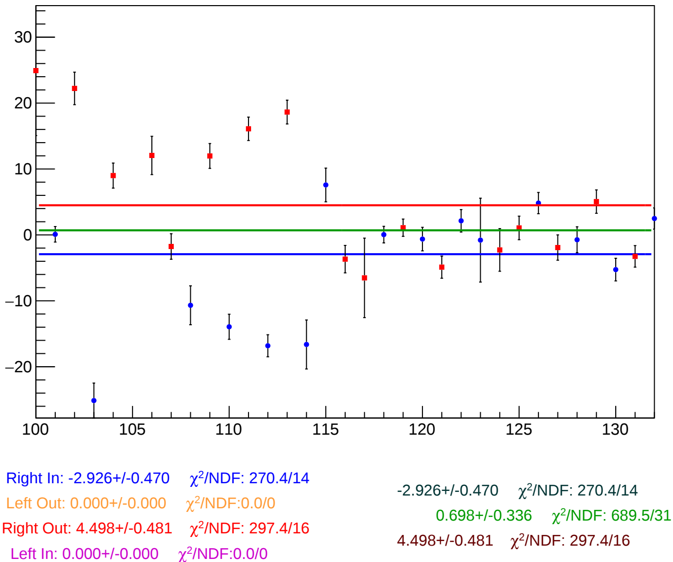
reg_asym_sam_2468_avg_diff_bpm4aY_slope vs Slug, Sign Corrected
