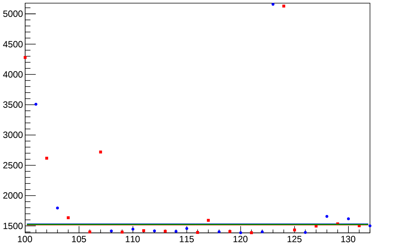
reg_asym_atl_avg_atr_avg_dd_rms vs Slug, Sign Corrected
