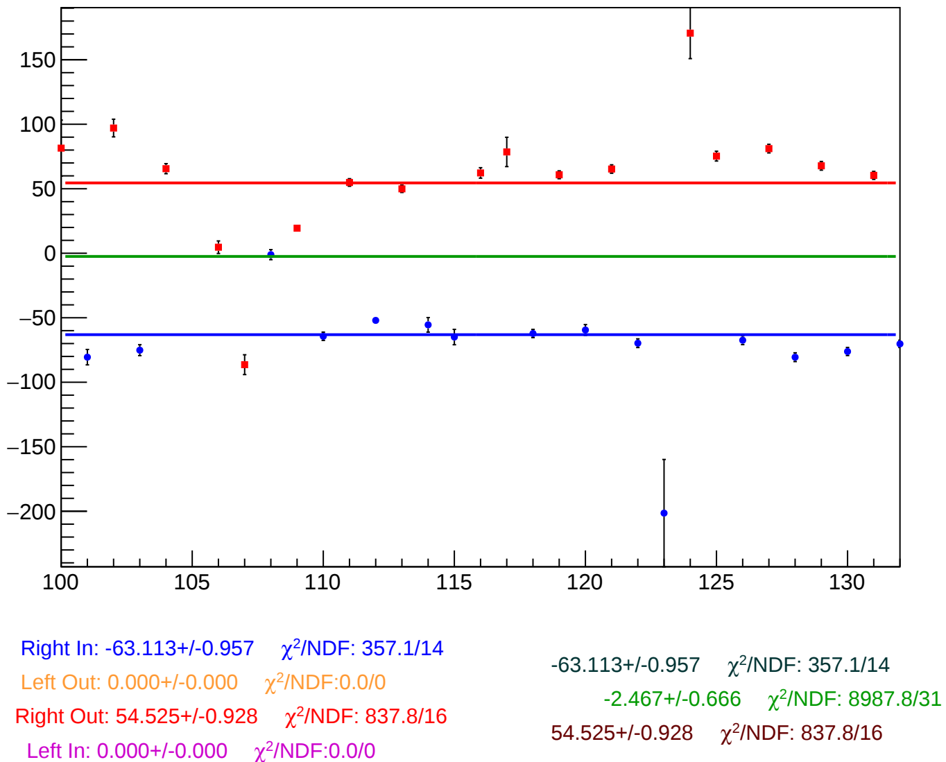
reg_asym_atl_avg_atr_avg_dd_diff_bpm4eX_slope vs Slug, Sign Corrected
