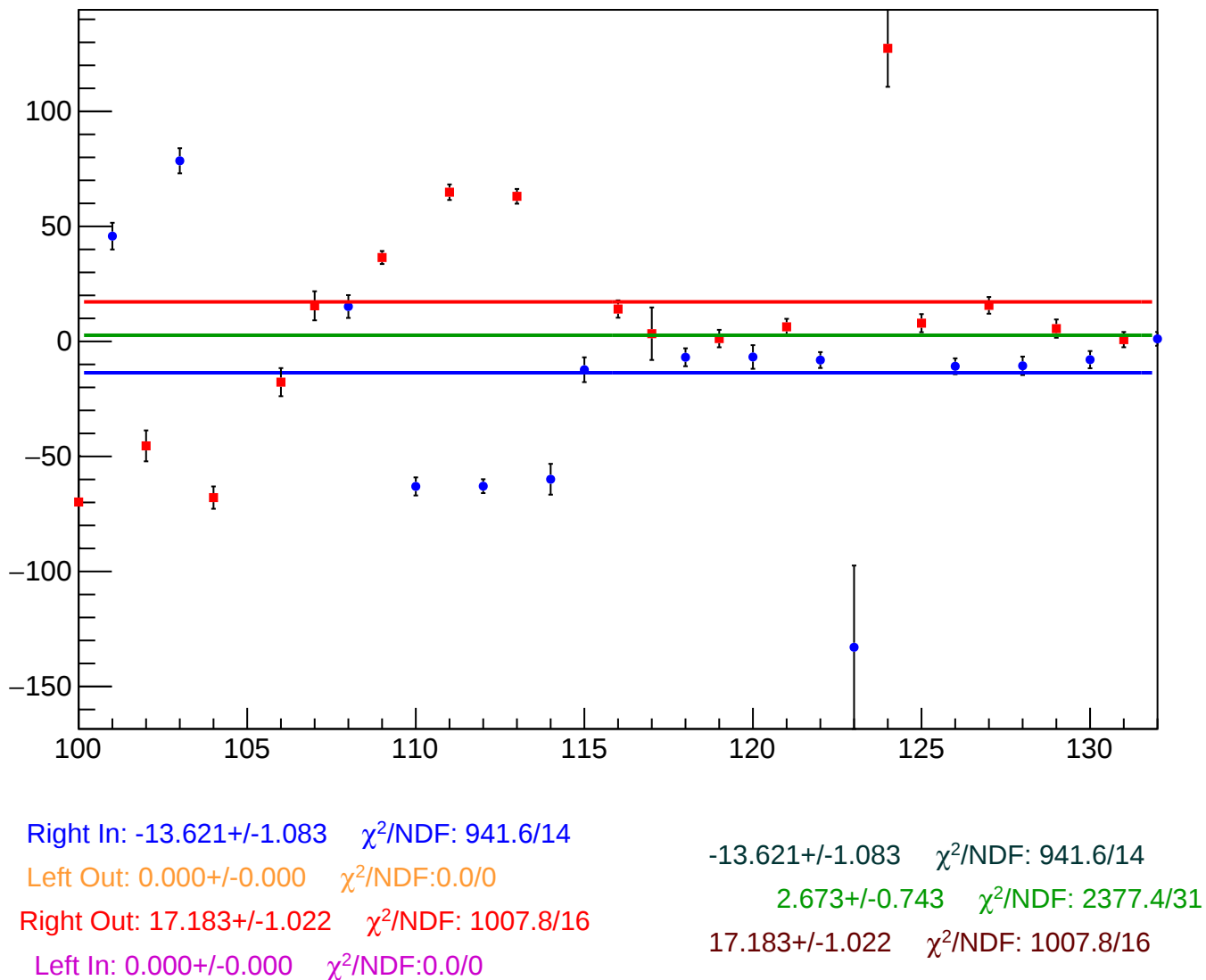
reg_asym_atl_dd_atr_dd_diff_bpm4aX_slope vs Slug, Sign Corrected
