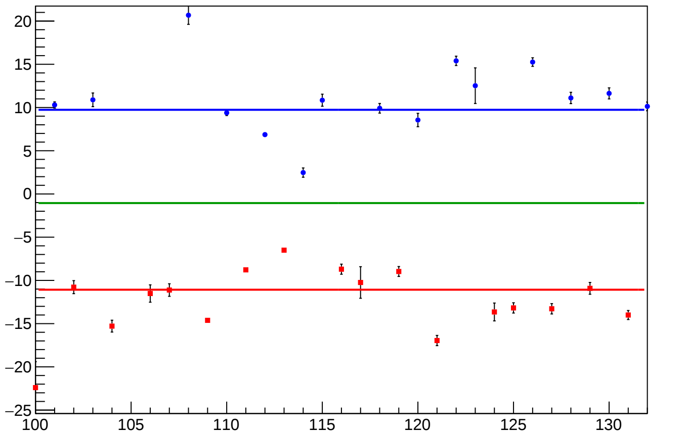
reg_asym_sam7_diff_bpm4aY_slope vs Slug, Sign Corrected
