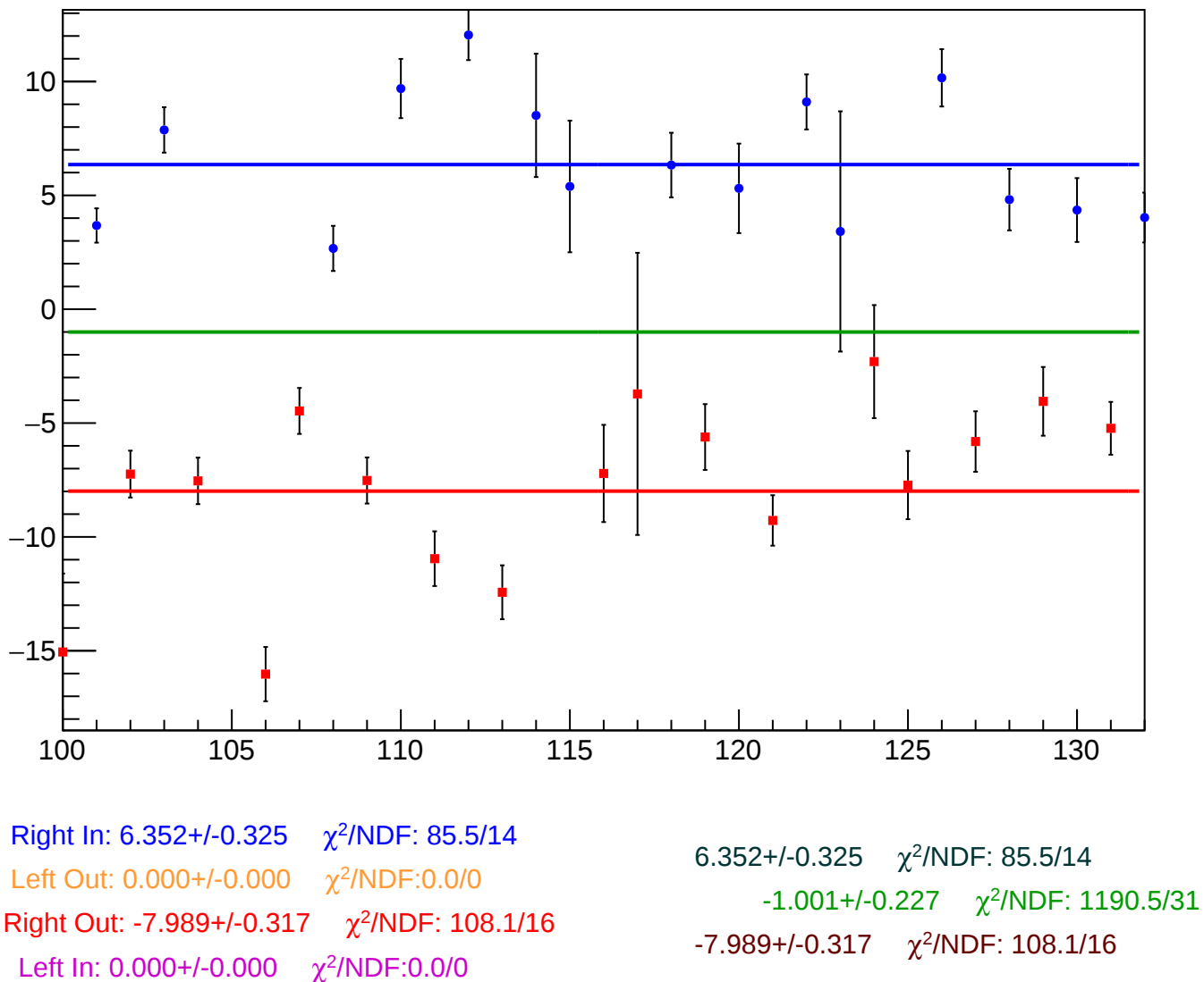
reg_asym_sam_13_57_dd_diff_bpm4eX_slope vs Slug, Sign Corrected
