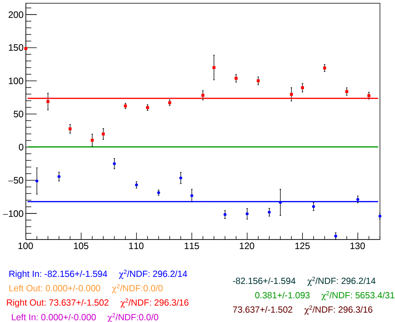
reg_asym_atr1_diff_bpm4aX_slope vs Slug, Sign Corrected
