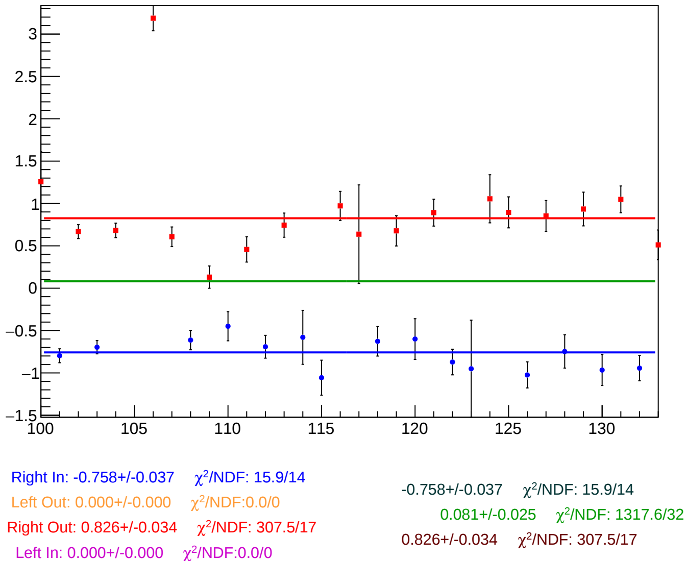
reg_asym_sam_24_68_dd_diff_bpm12X_slope vs Slug, Sign Corrected
