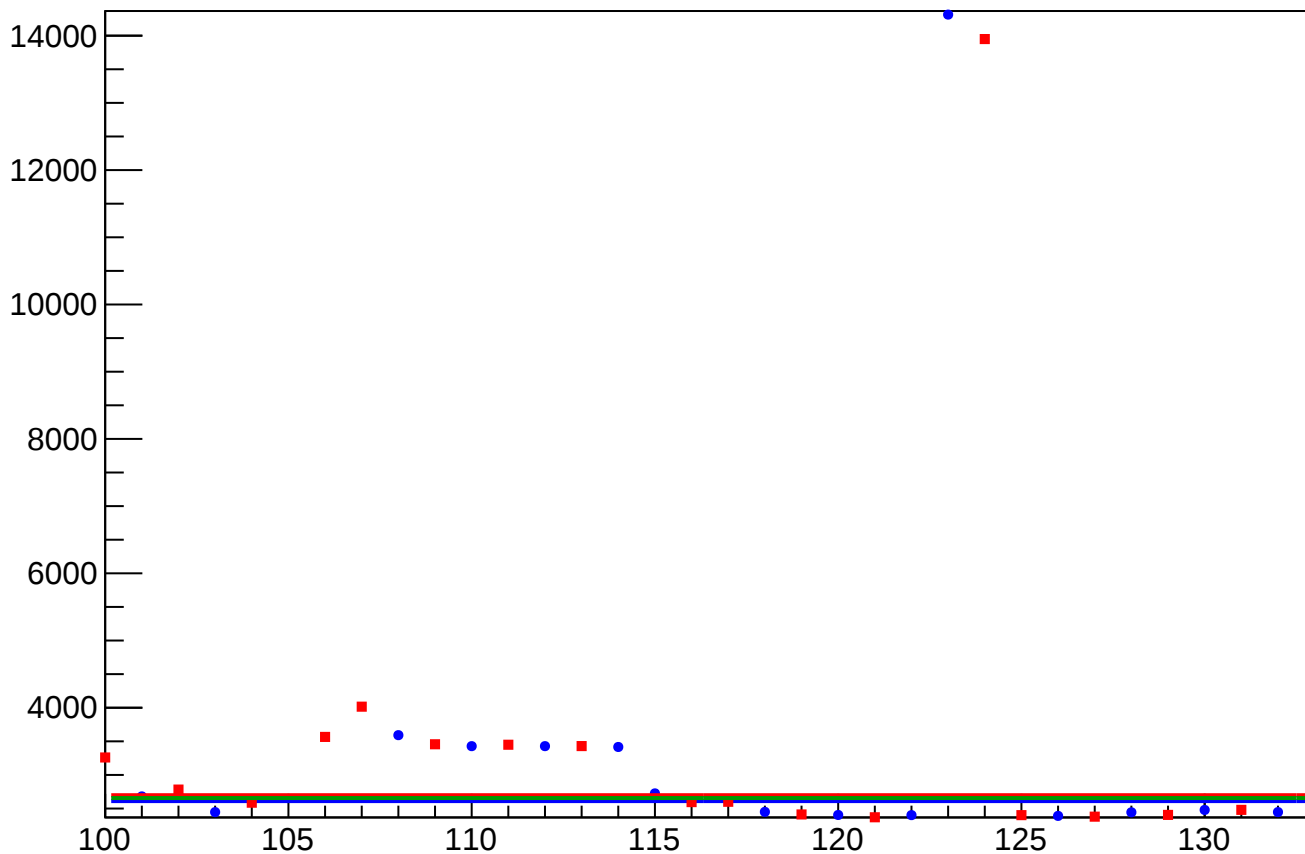
reg_asym_atl1_rms vs Slug, Sign Corrected
