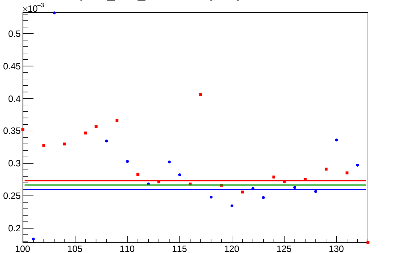
yield_atr2_rms vs Slug, Sign Corrected
