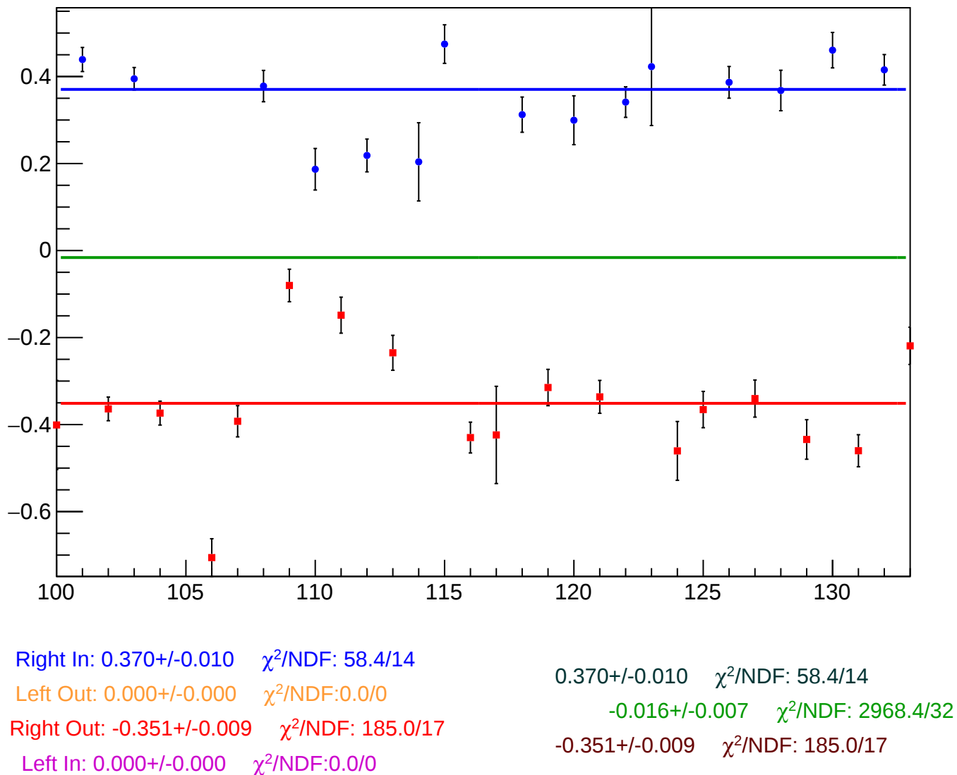
reg_asym_sam_1357_2468_dd_diff_bpm12X_slope vs Slug, Sign Corrected
