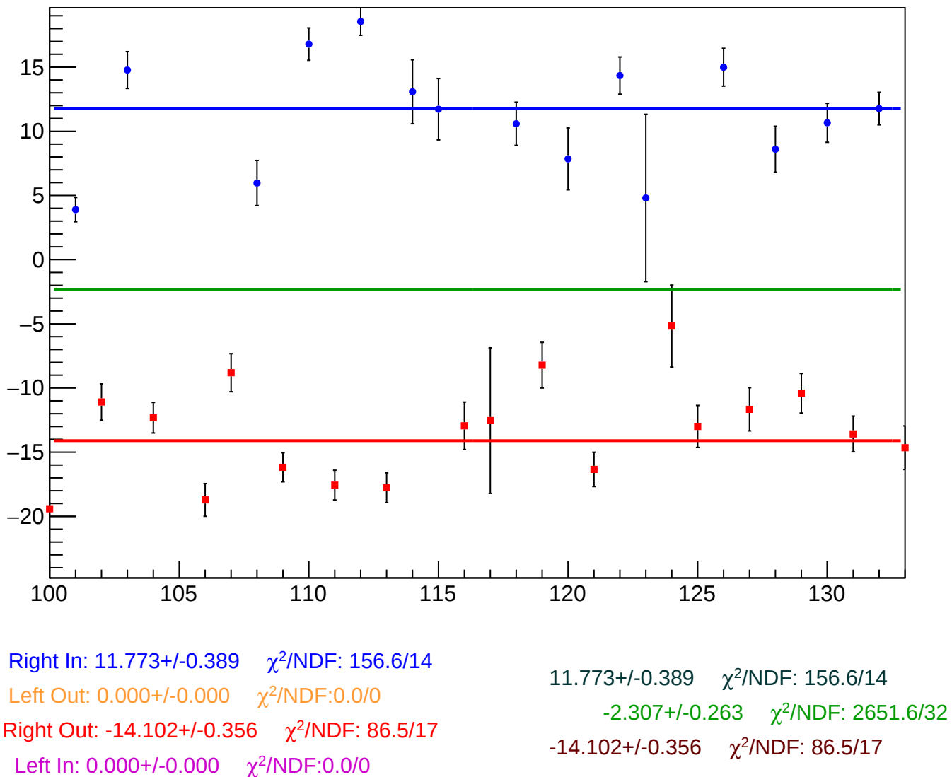
reg_asym_sam_37_dd_diff_bpm4eX_slope vs Slug, Sign Corrected
