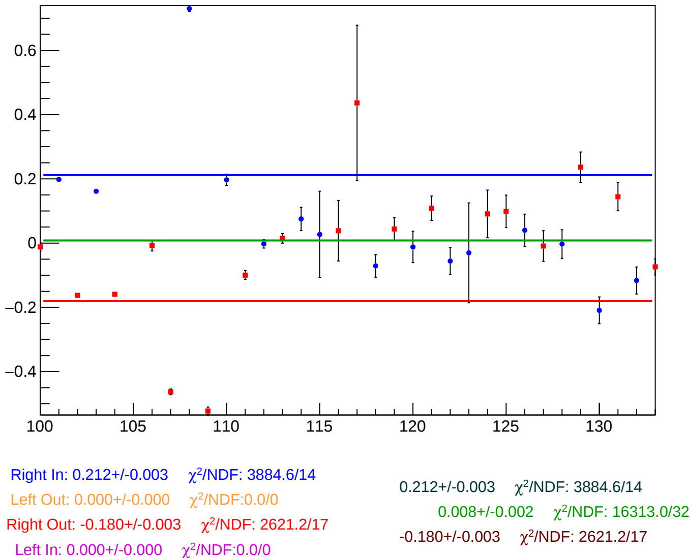
reg_asym_sam_15_avg_diff_bpm12X_slope vs Slug, Sign Corrected
