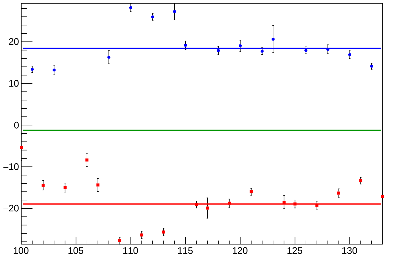
reg_asym_sam_1357_2468_dd_diff_bpm4eX_slope vs Slug, Sign Corrected
