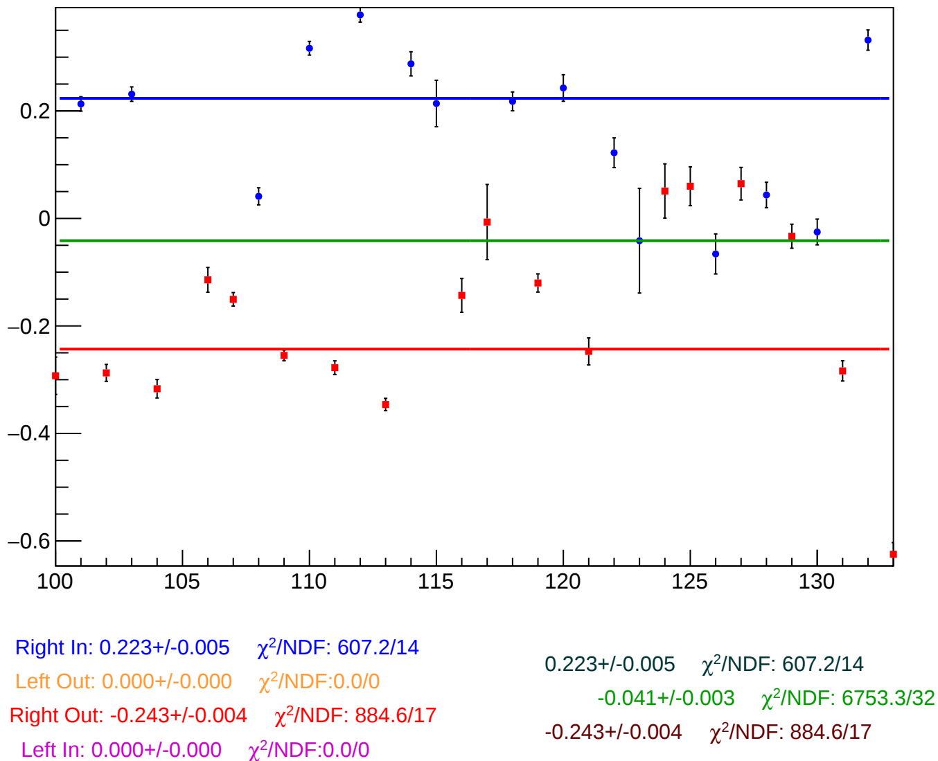
reg_asym_bcm_an_us_diff_bpm12X_slope vs Slug, Sign Corrected
