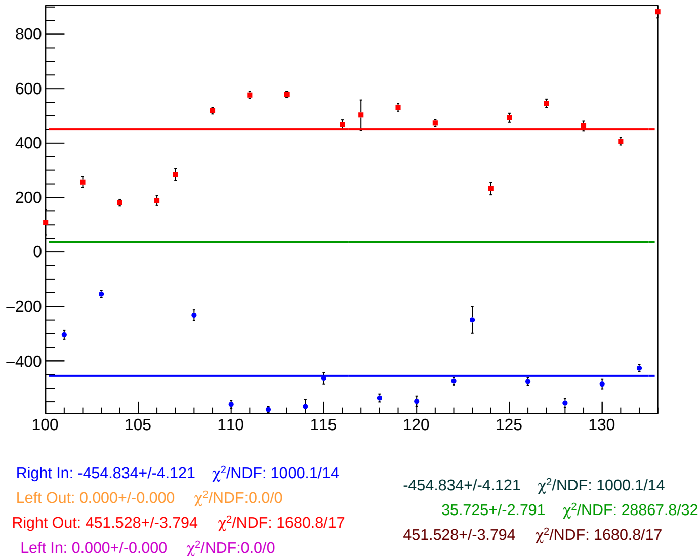
reg_asym_at2_avg_diff_bpm4aX_slope vs Slug, Sign Corrected
