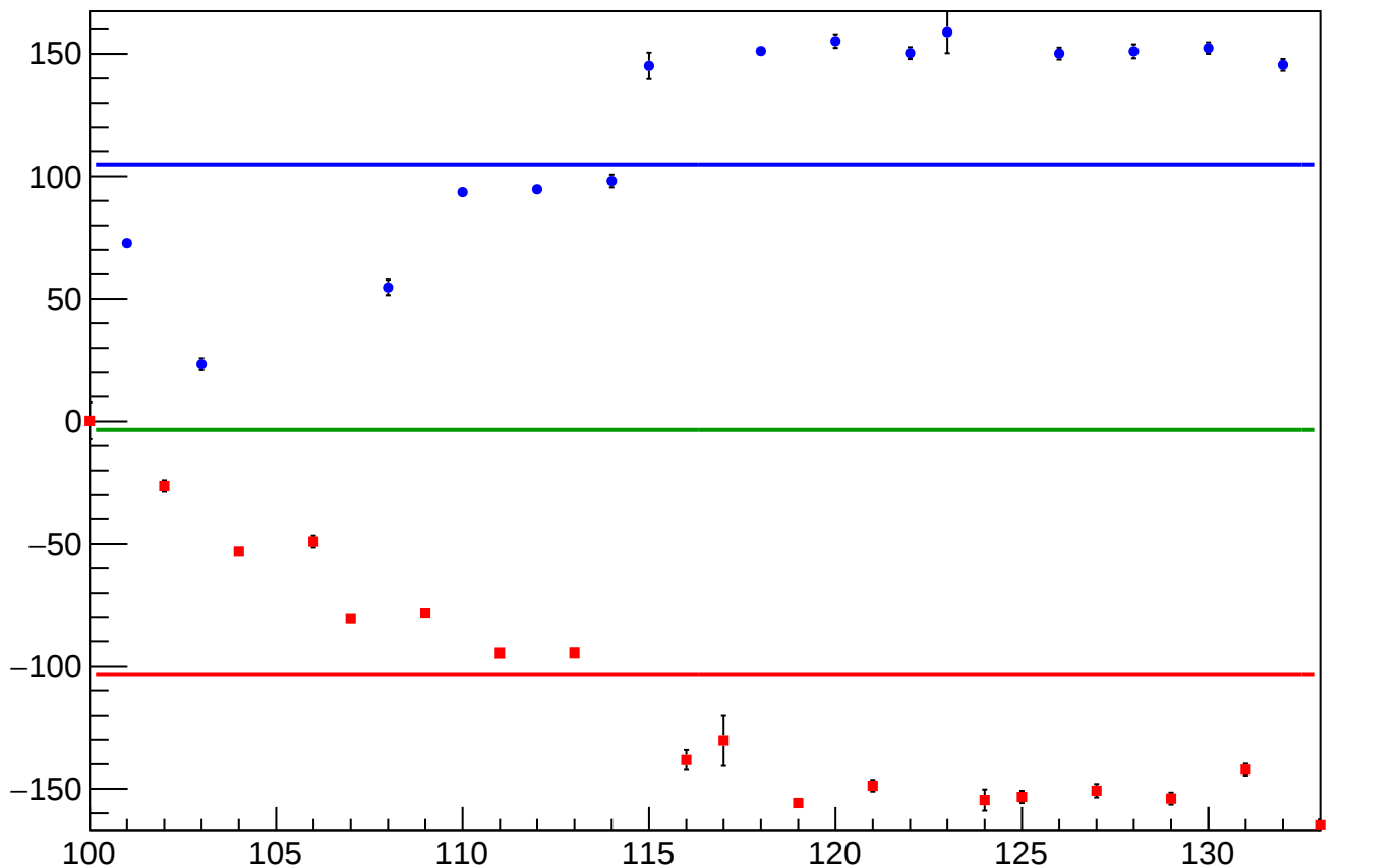
reg_asym_sam_48_avg_diff_bpm4eY_slope vs Slug, Sign Corrected
