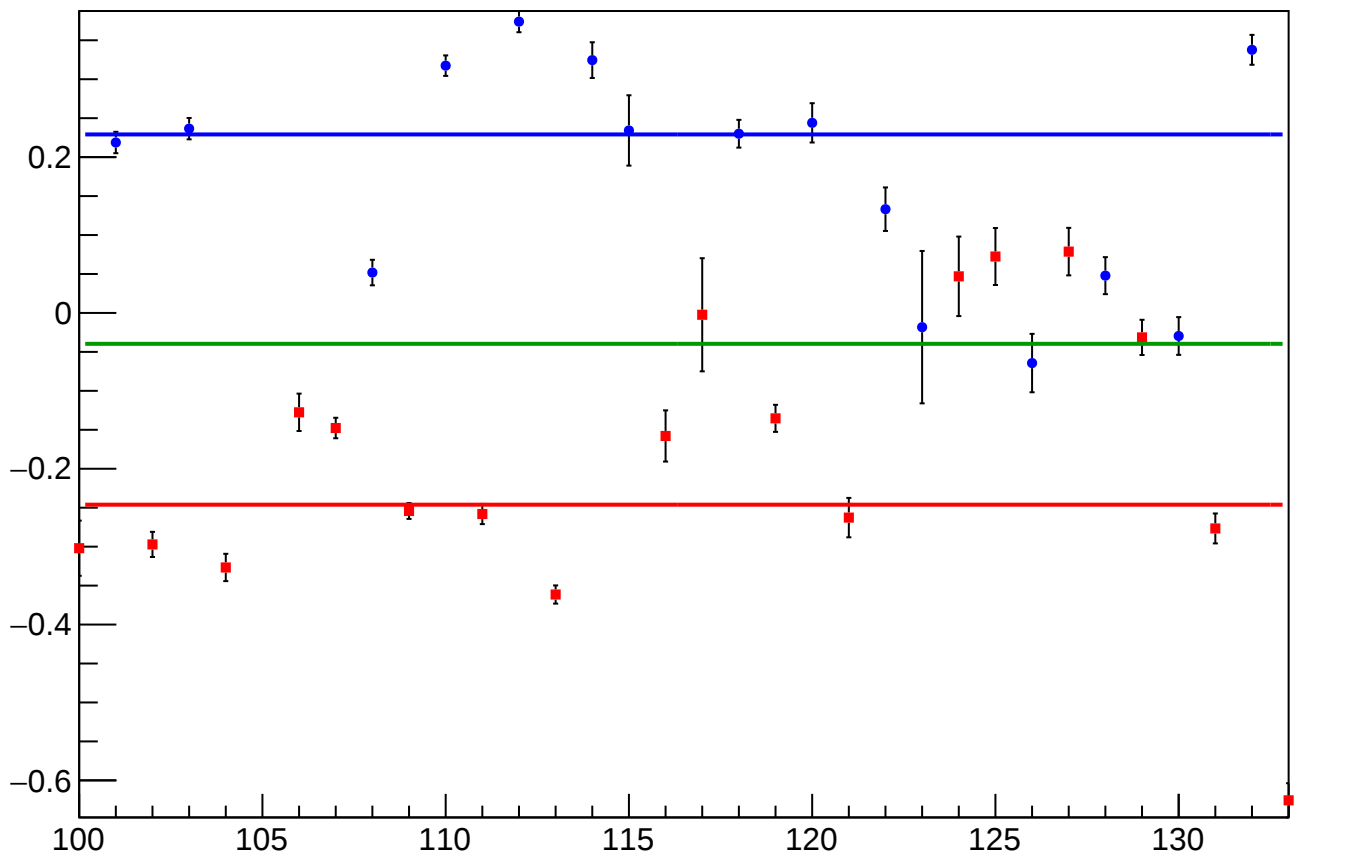
reg_asym_bcm_dg_ds_diff_bpm12X_slope vs Slug, Sign Corrected
