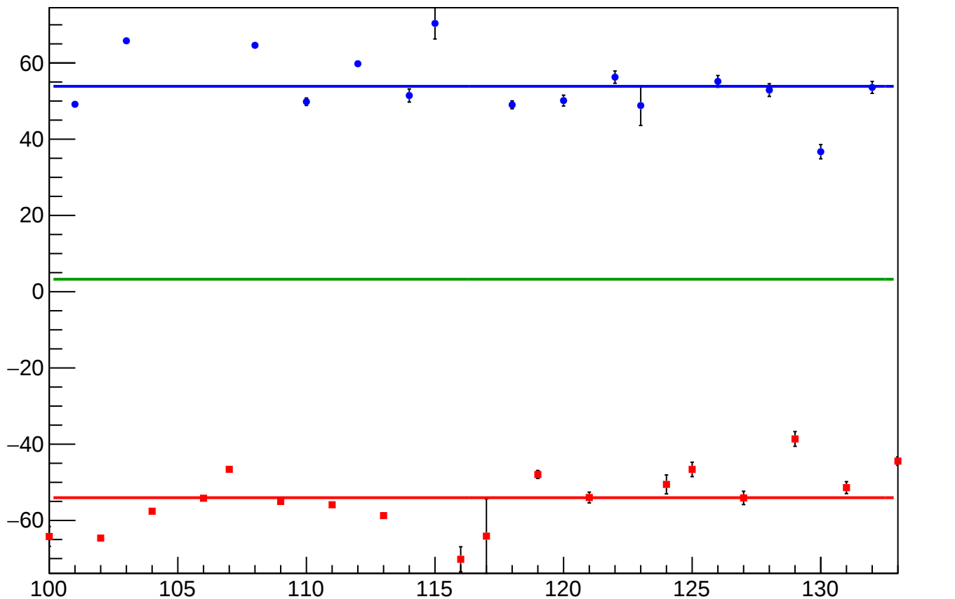
reg_asym_sam6_diff_bpm4aY_slope vs Slug, Sign Corrected
