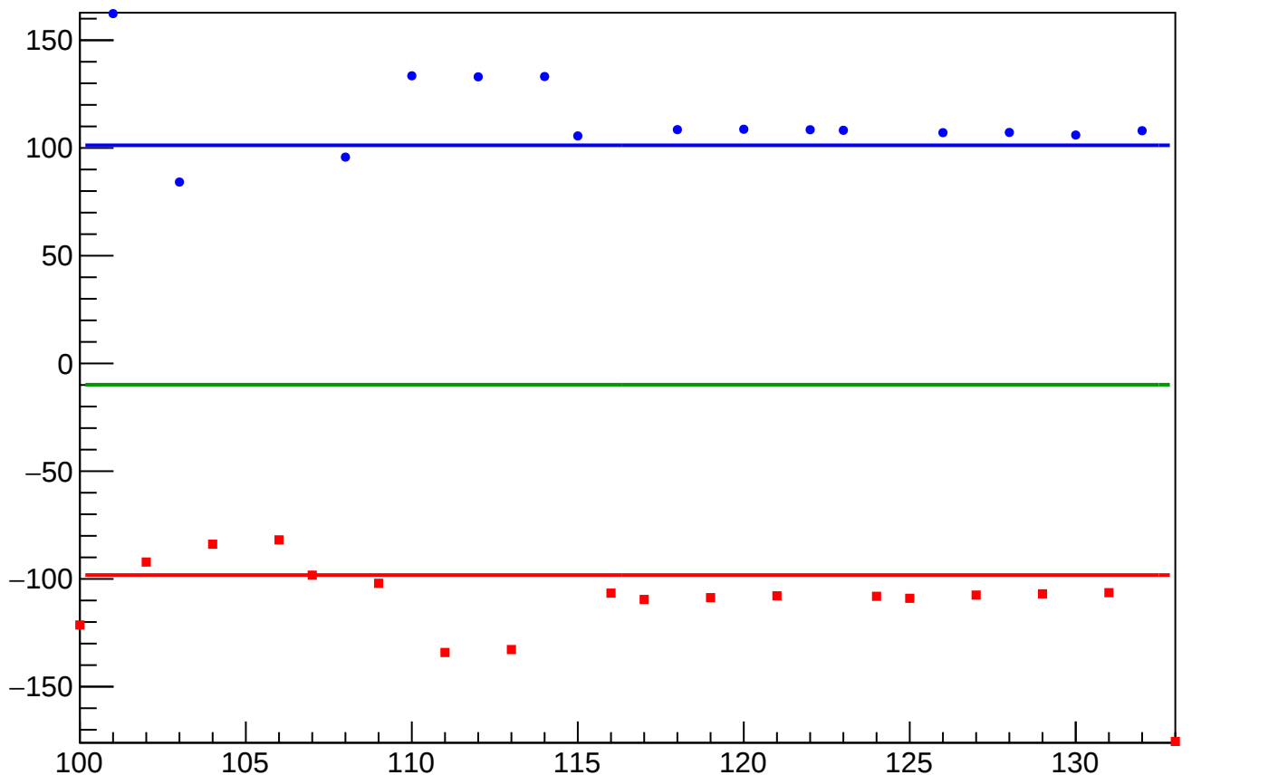
reg_asym_atr_dd_diff_bpm12X_slope vs Slug, Sign Corrected
