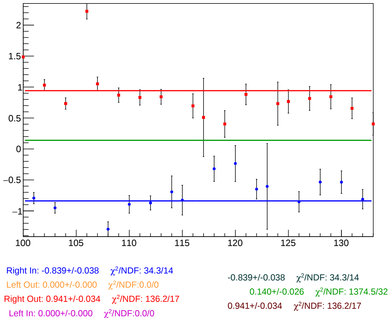
reg_asym_sam3_diff_bpm12X_slope vs Slug, Sign Corrected
