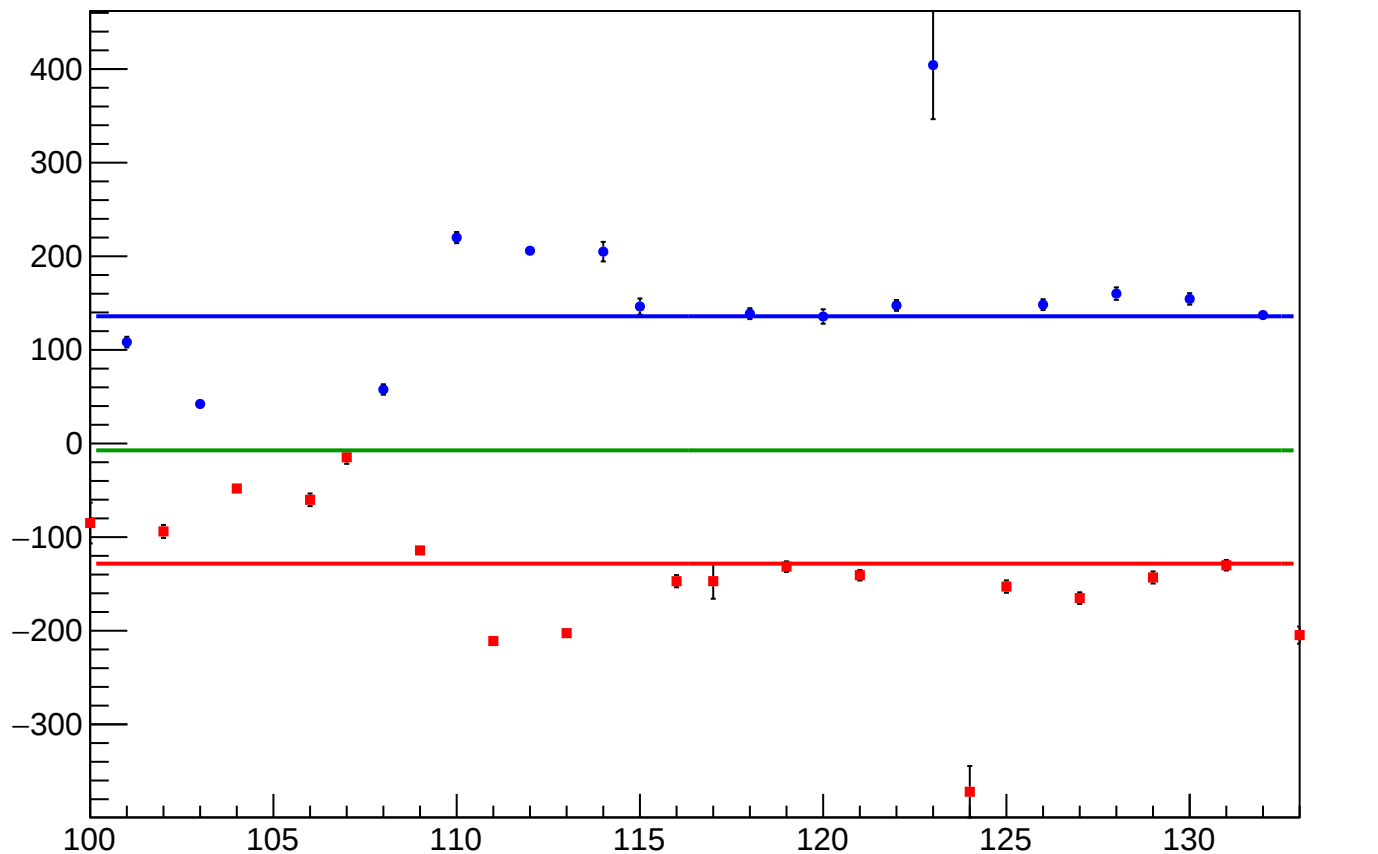
reg_asym_at2_dd_diff_bpm4eX_slope vs Slug, Sign Corrected
