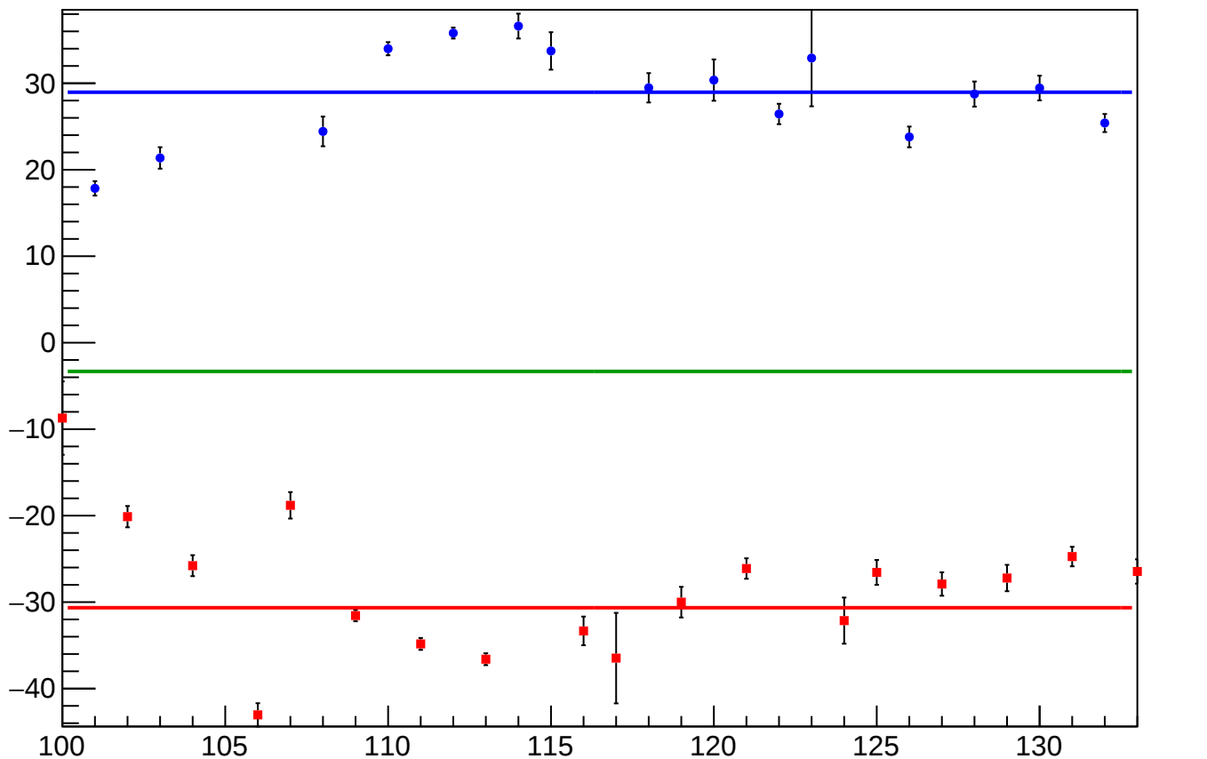
reg_asym_sam_15_37_dd_diff_bpm4eX_slope vs Slug, Sign Corrected
