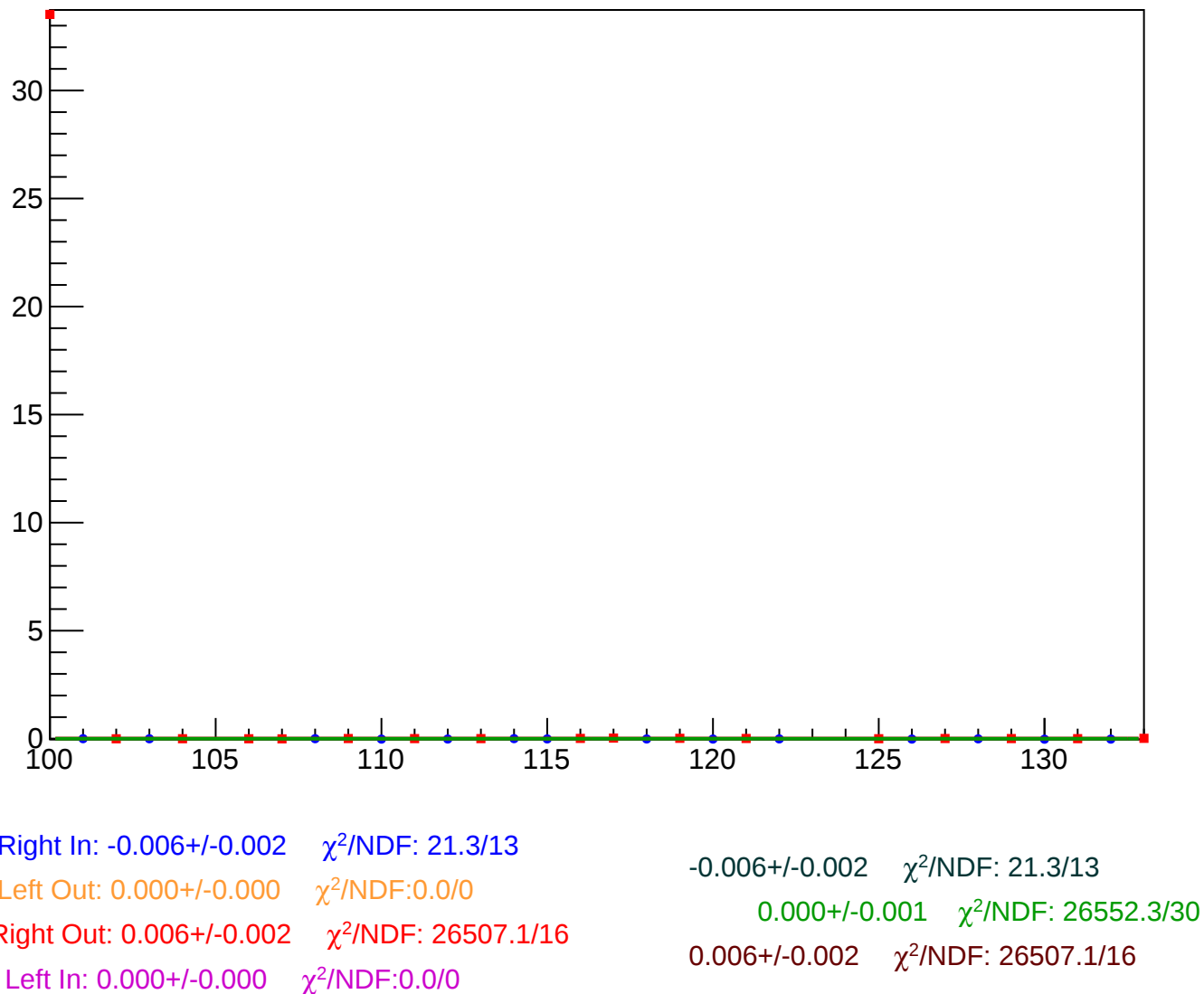
reg_asym_ds_avg_diff_bpm12X_slope vs Slug, Sign Corrected
