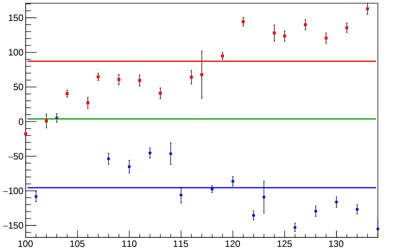
reg_asym_atr_dd_diff_bpm4eY_slope vs Slug, Sign Corrected
