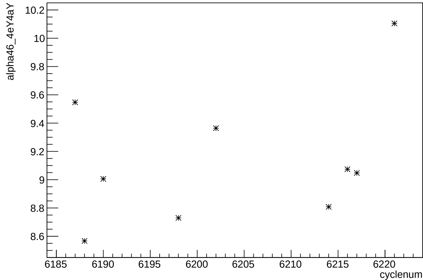
alpha46_4eY4aY:cyclenum
