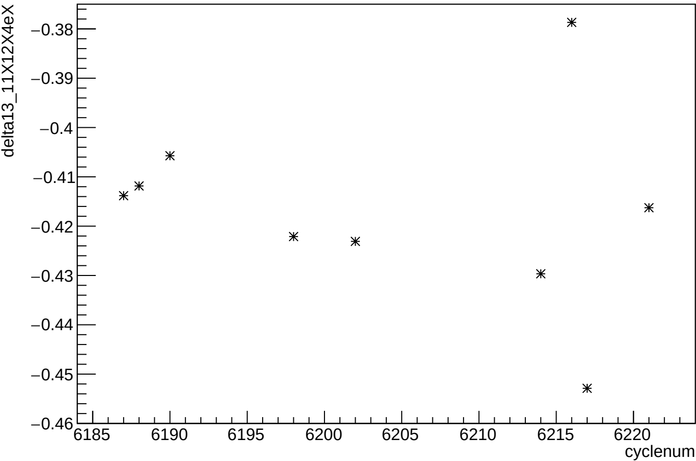
delta13_11X12X4eX:cyclenum
