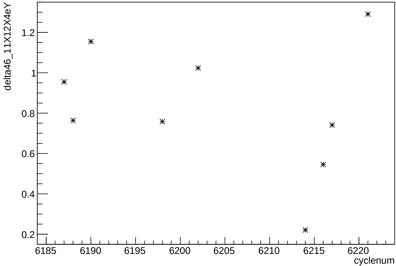
delta46_11X12X4eY:cyclenum
